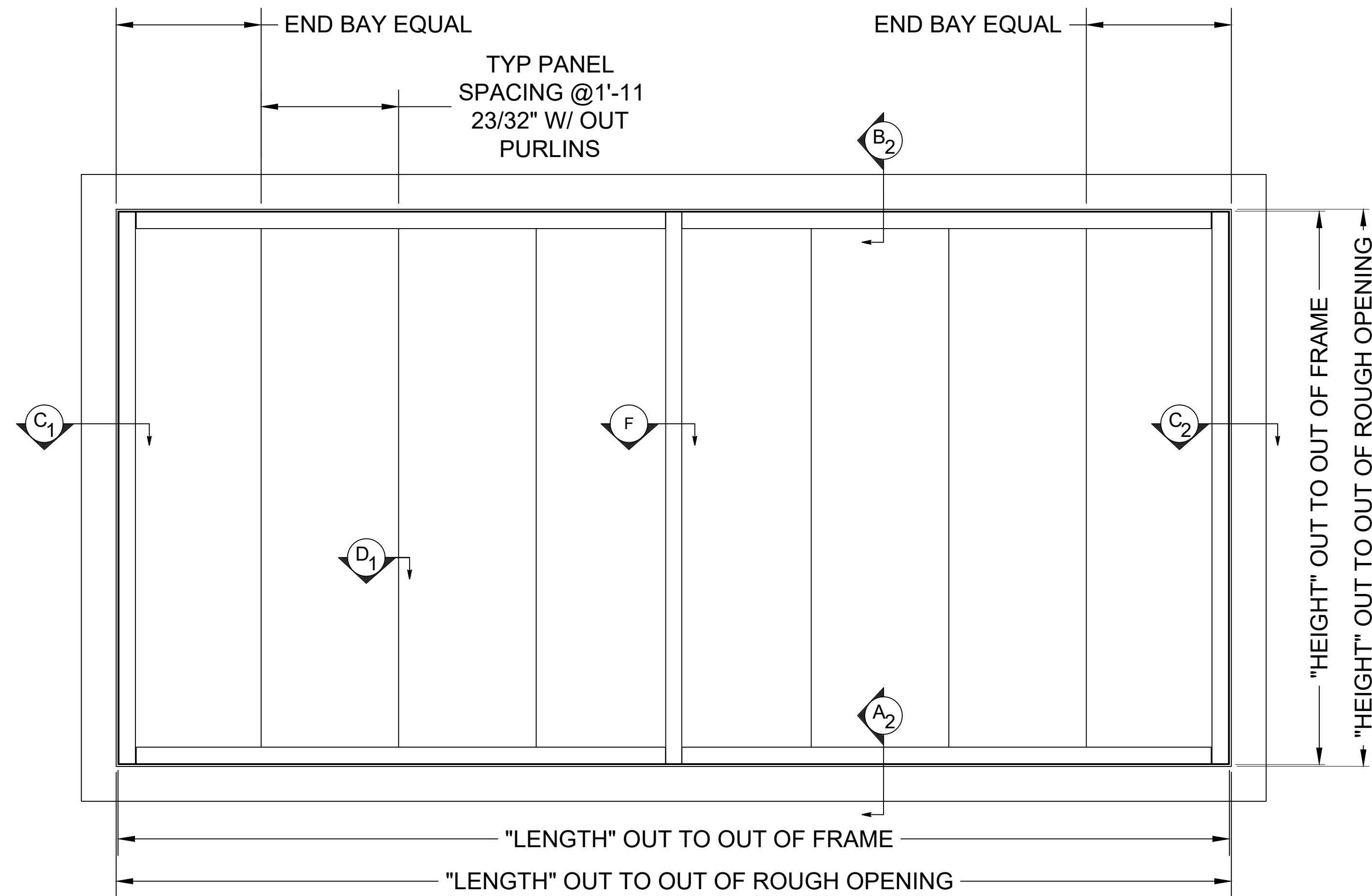
ELEVATION (W/ OPTIONAL MULLION)
