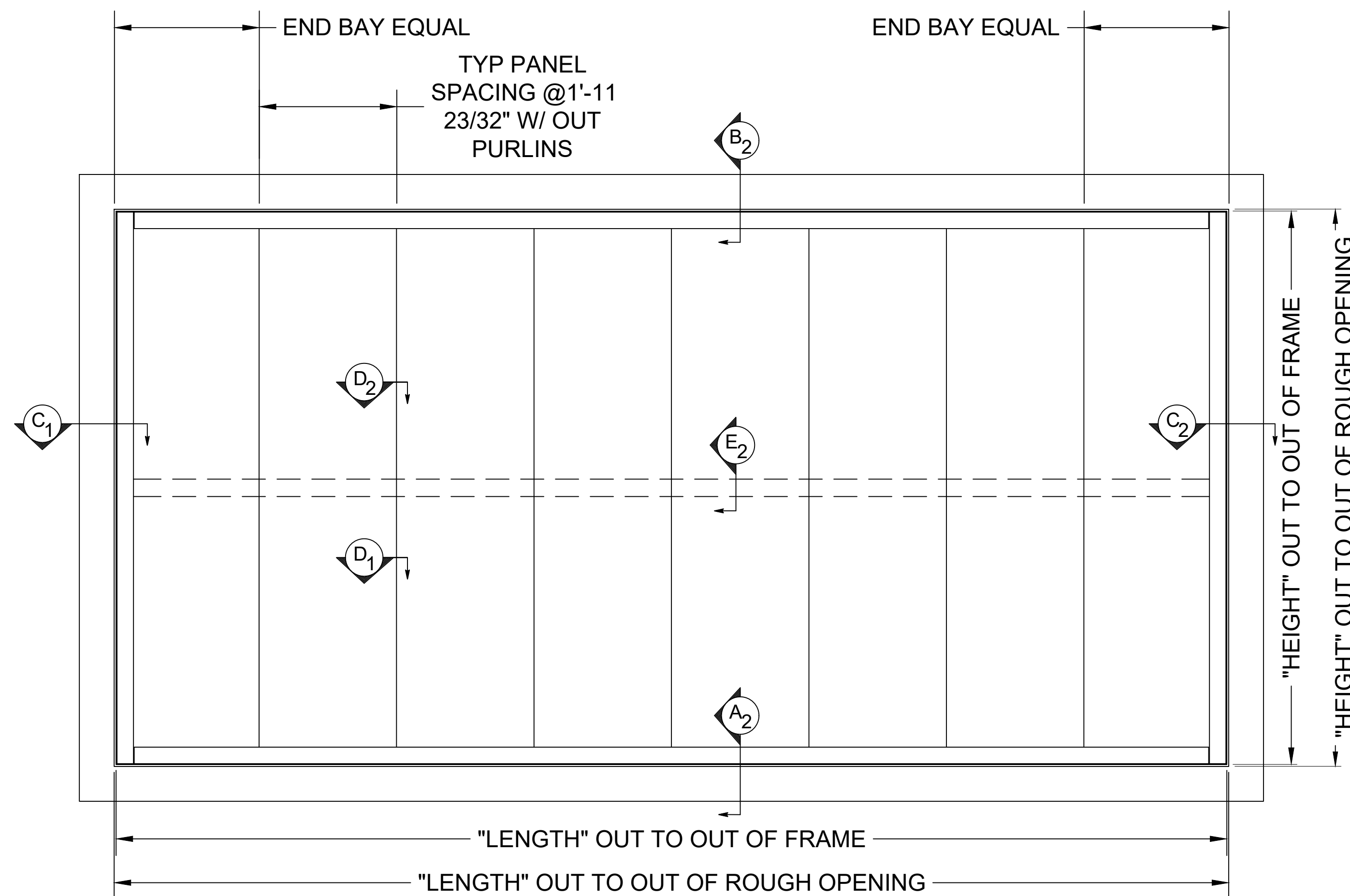
ELEVATION (FLUSH)
