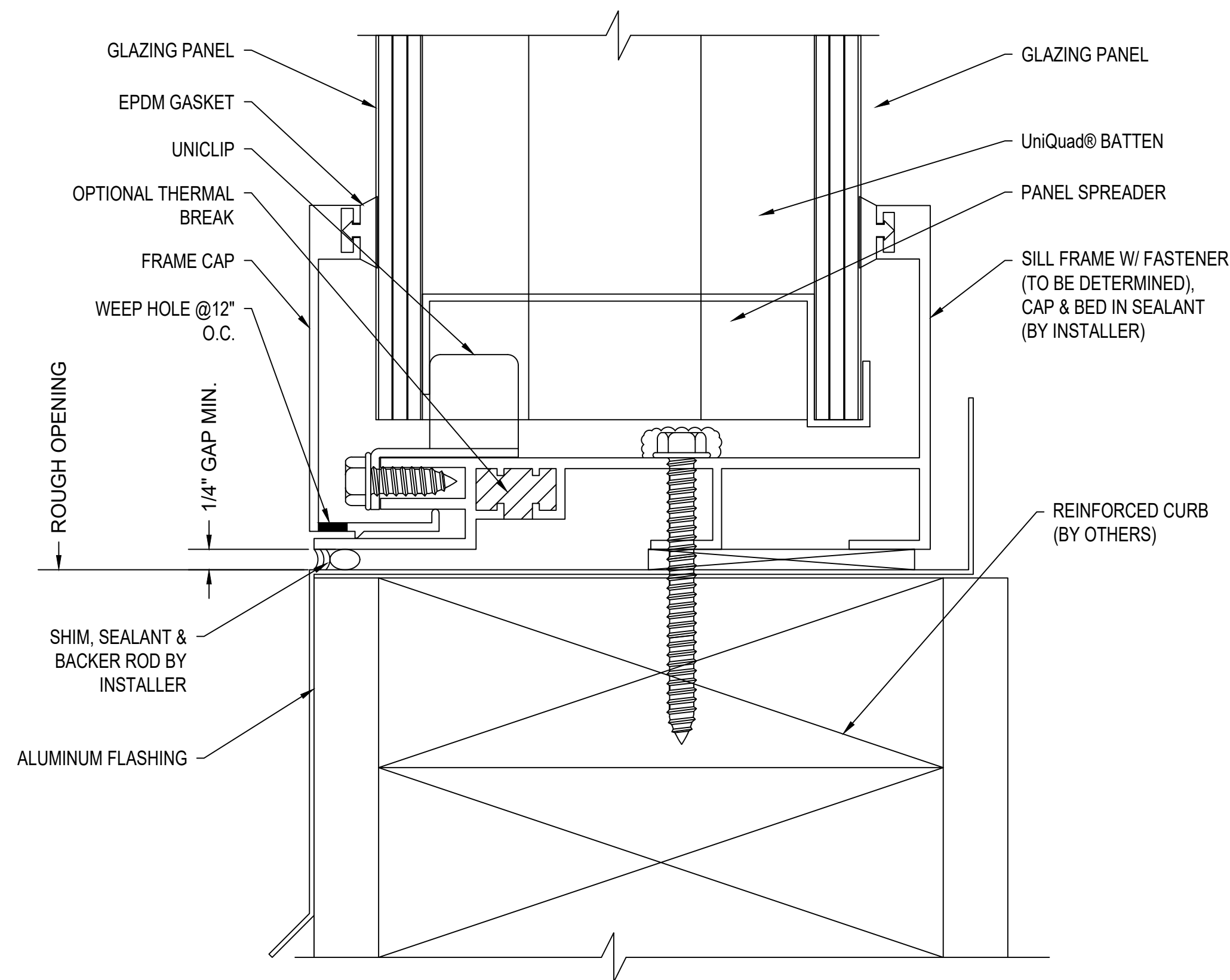
A 2 SECTION @ SILL 4" UniQuad®
