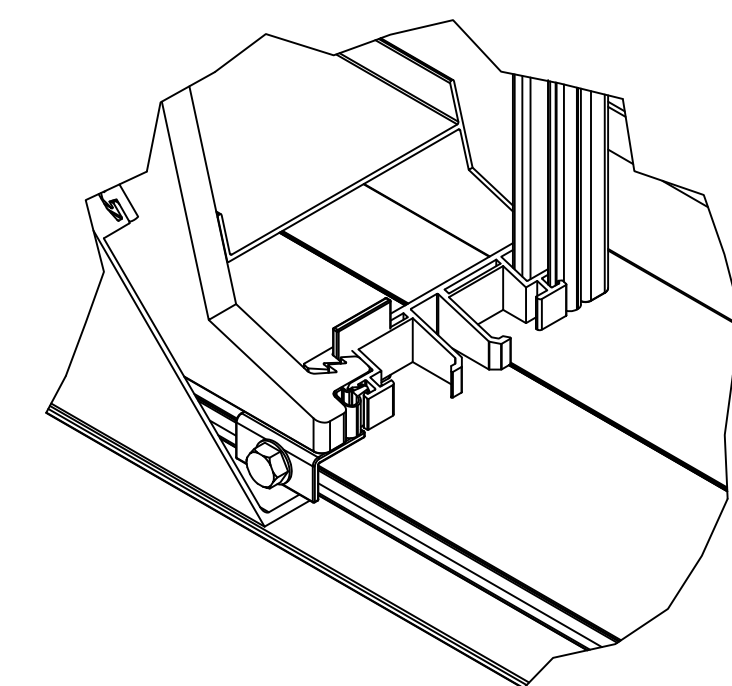
A 1 UNICLIP CONNECTION @ HEAD 4" UniQuad®
