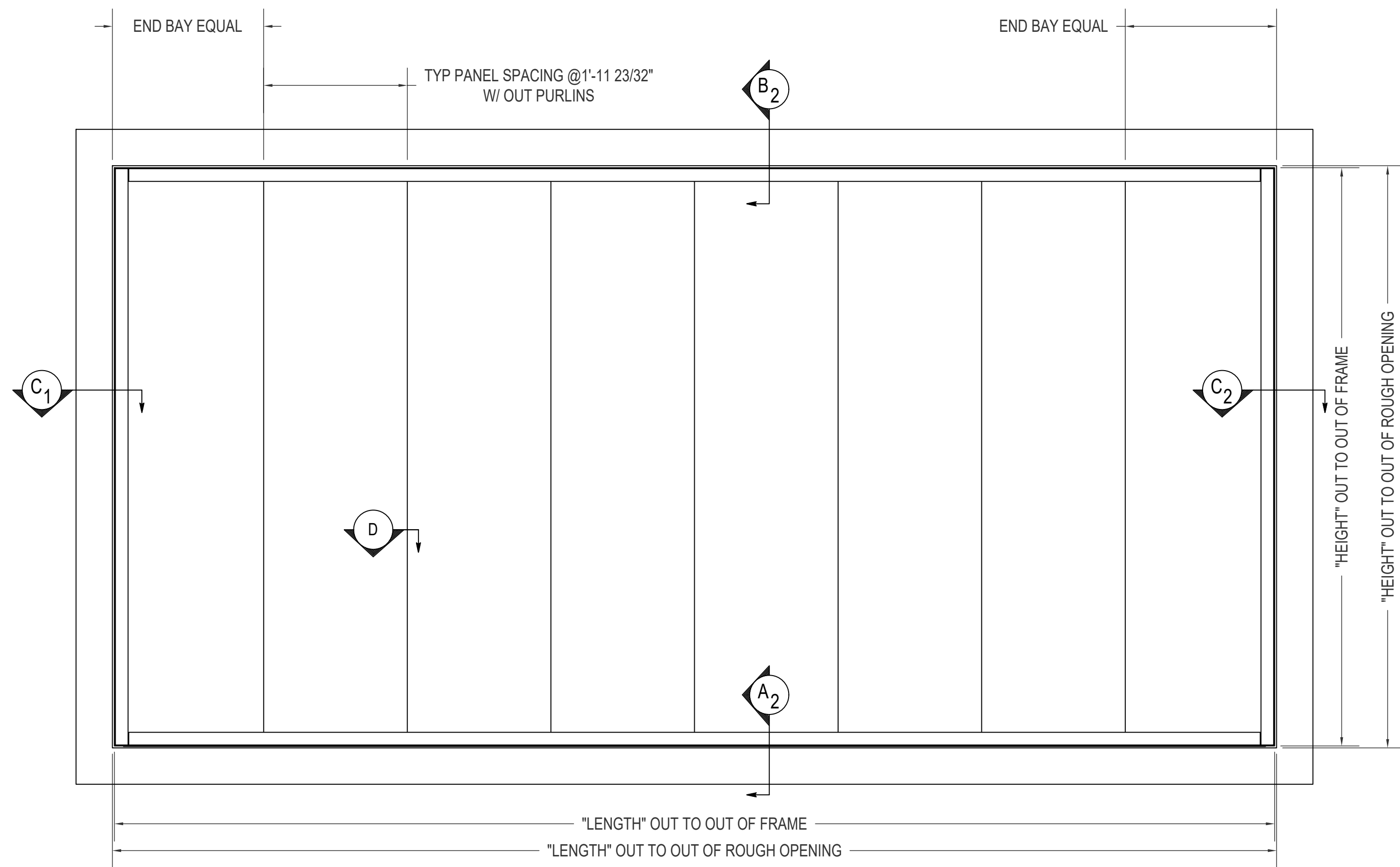
ELEVATION (FLUSH)
