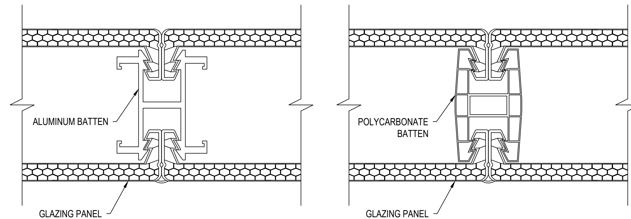
E 2 BATTEN DETAIL UniQuad® WINDOW
