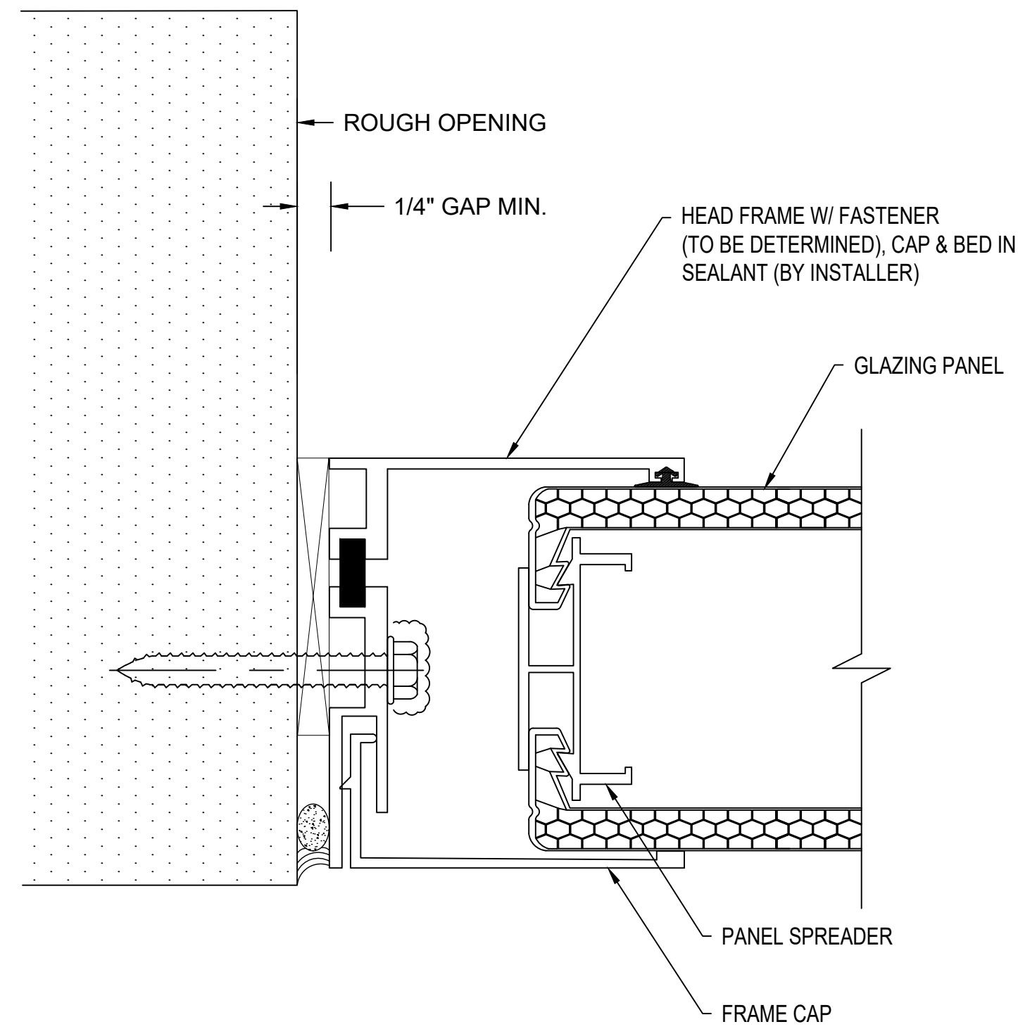
C 2 SECTION @ JAMB UniQuad® WINDOW
