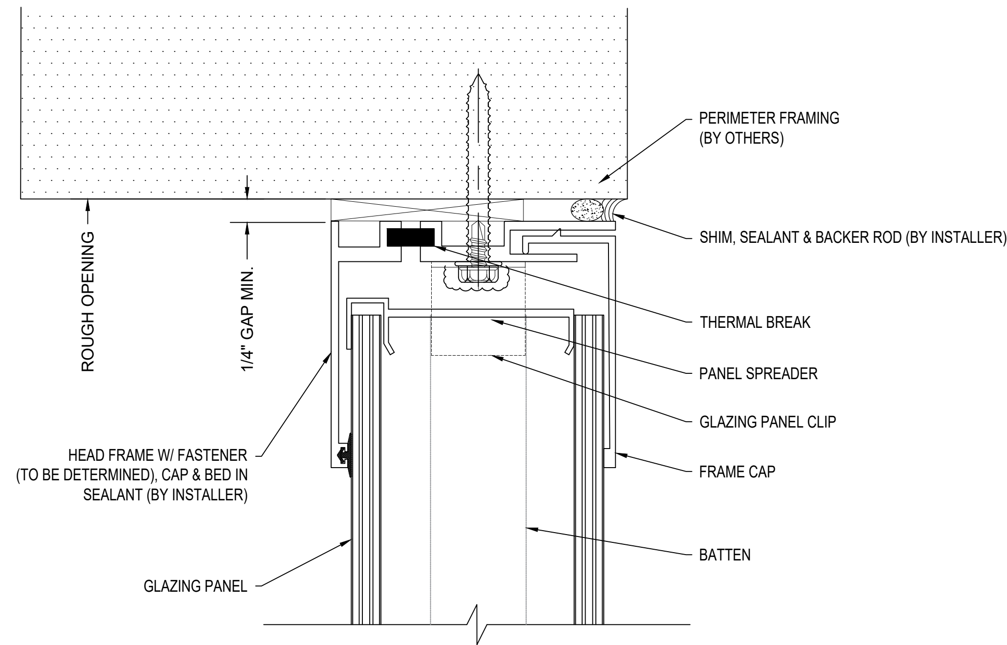
B 2 SECTION @ HEAD UniQuad® WINDOW
