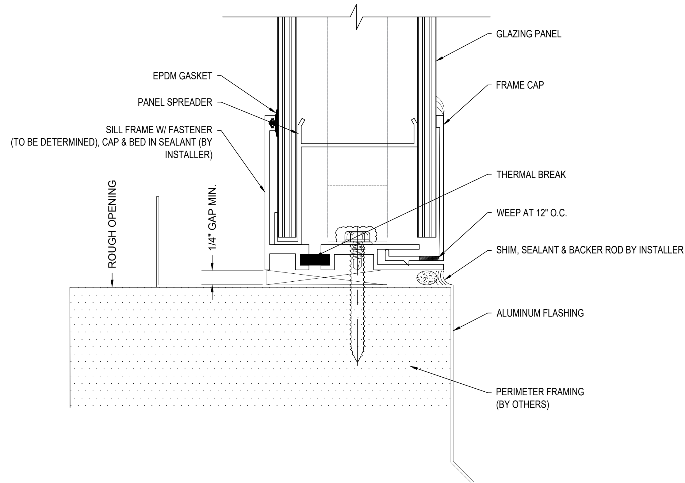
A 2 SECTION @ SILL UniQuad® WINDOW
