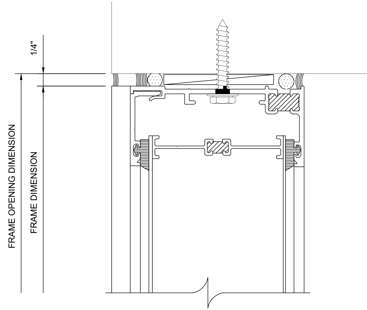
1 2 HEAD DETAIL SCALE: FULL
