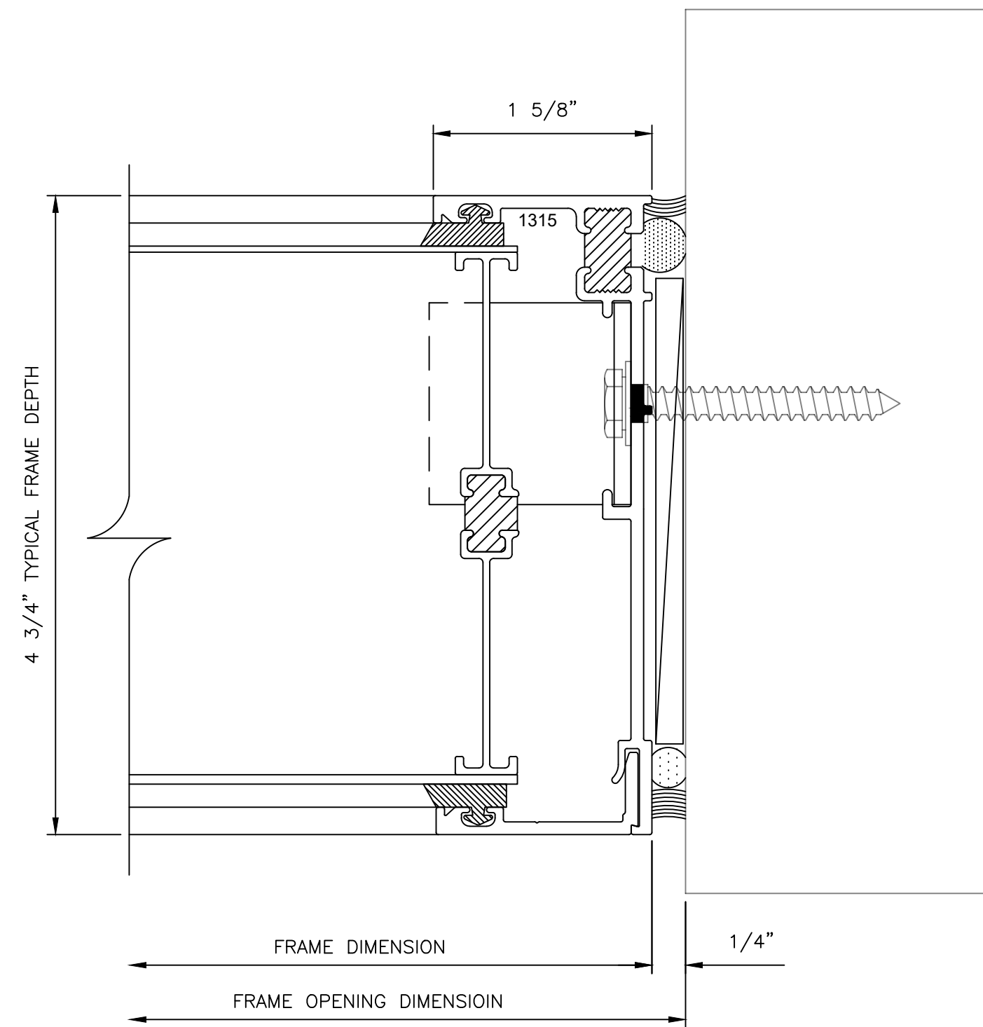
4 2 JAMB DETAIL - - SCALE: FULL
