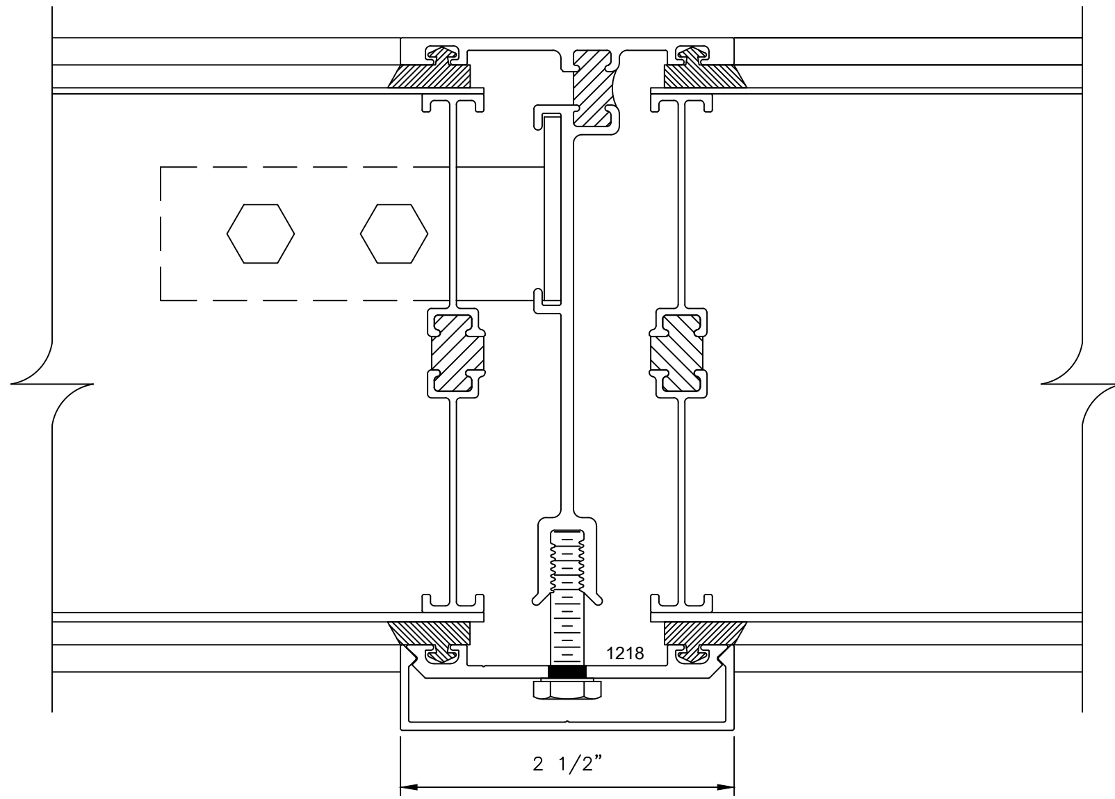
3 2 MULLION DETAIL - - SCALE: FULL
