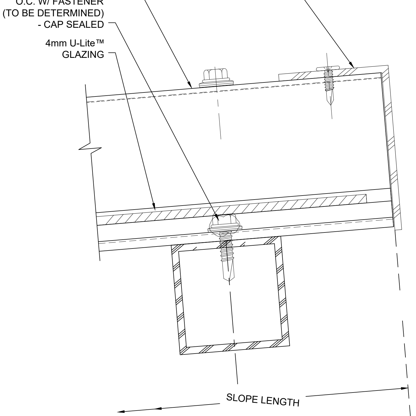
C 1 SECTION @ HEAD U-Lite™ SYSTEM
