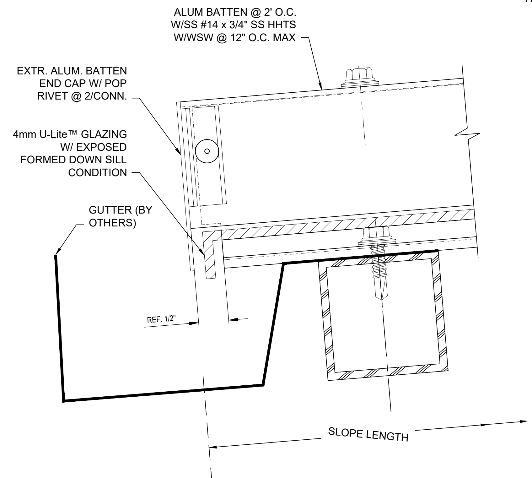
A 2 SECTION @ SILL W/ OPTIONAL GUTTER U-Lite™ SYSTEM
