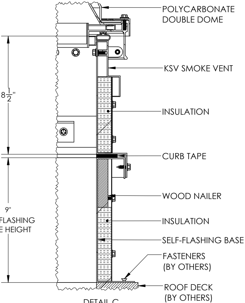
DETAIL C SCALE 1 : 4
