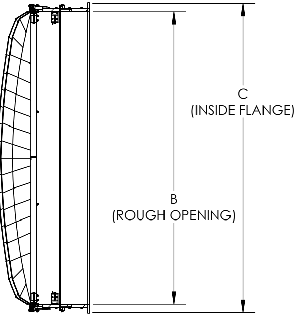
SECTION B-B
