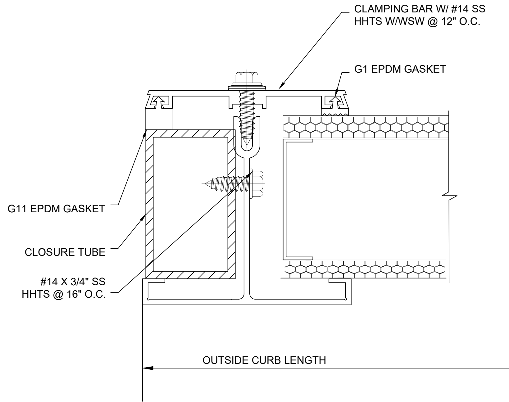
P SECTION @ OPEN END 2.75" QuadSpan™ SYSTEM (4" QuadSpan? SYSTEM SIMILAR)
