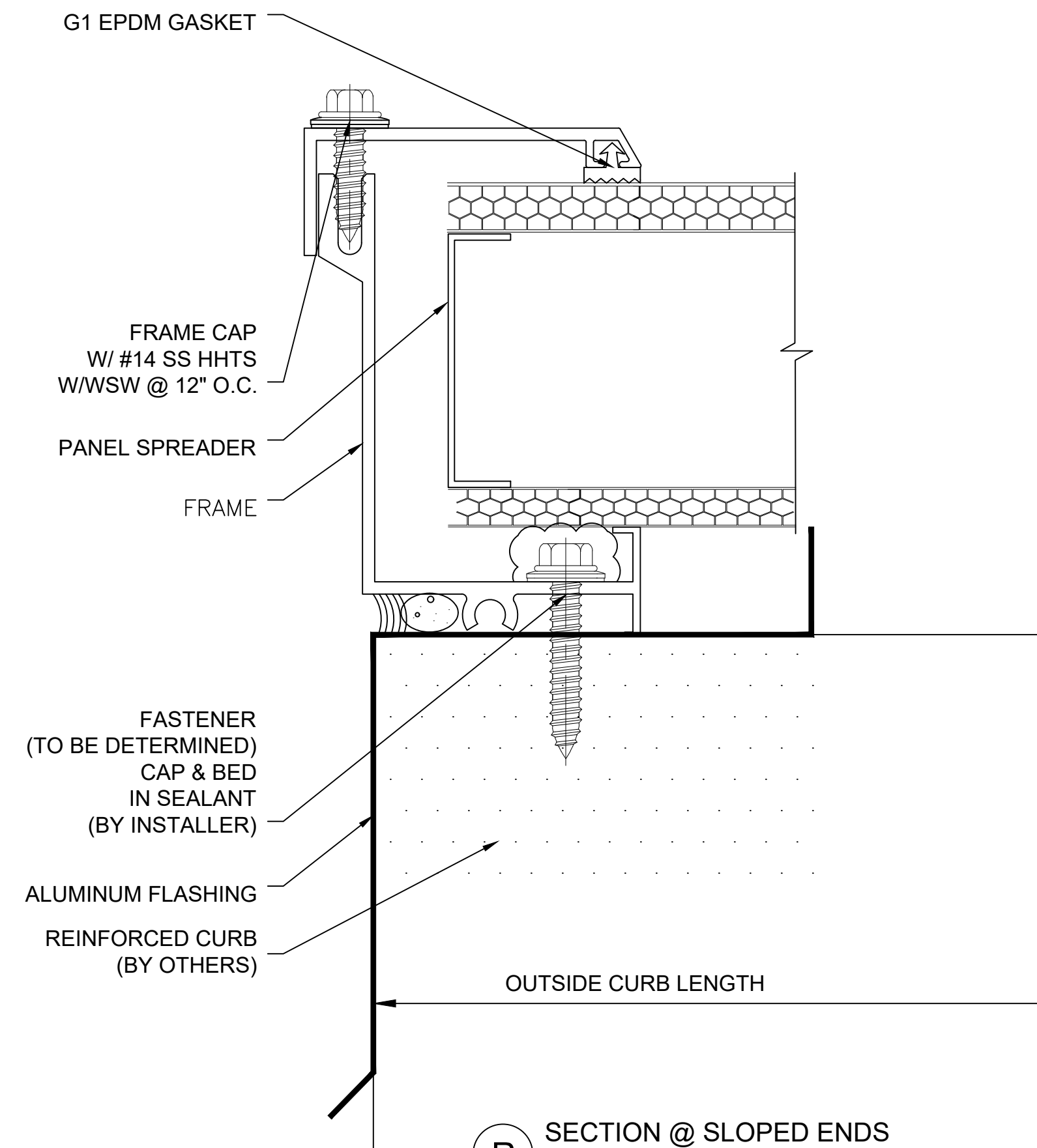
R SECTION @ SLOPED ENDS 2.75" QuadSpan™ SYSTEM (4" QuadSpan? SYSTEM SIMILAR)
