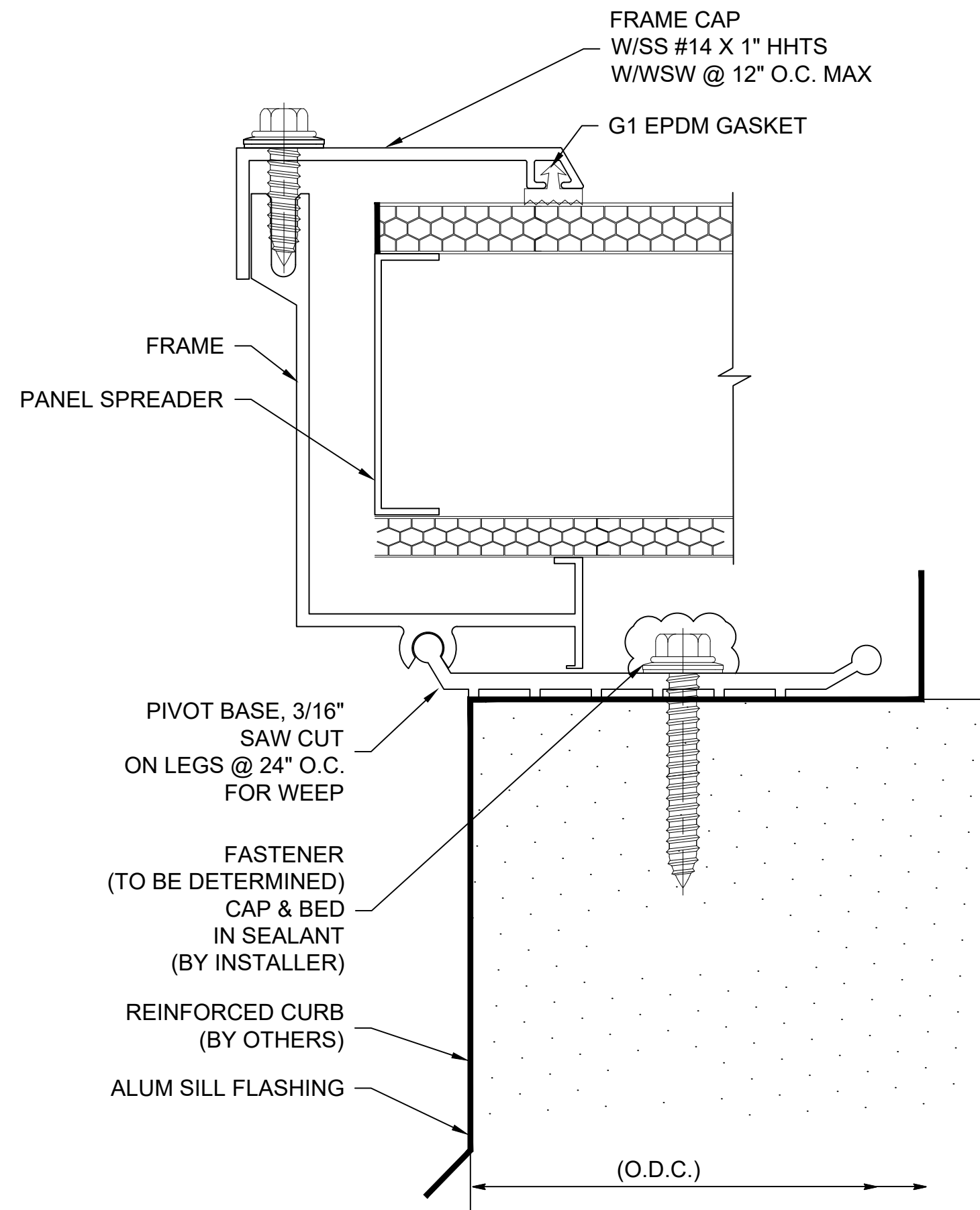
S SECTION @ SLOPED ENDS 2.75" QuadSpan™ SYSTEM (4" QuadSpan? SYSTEM SIMILAR)
