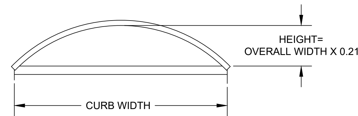
LOW-RISE ELEVATION
