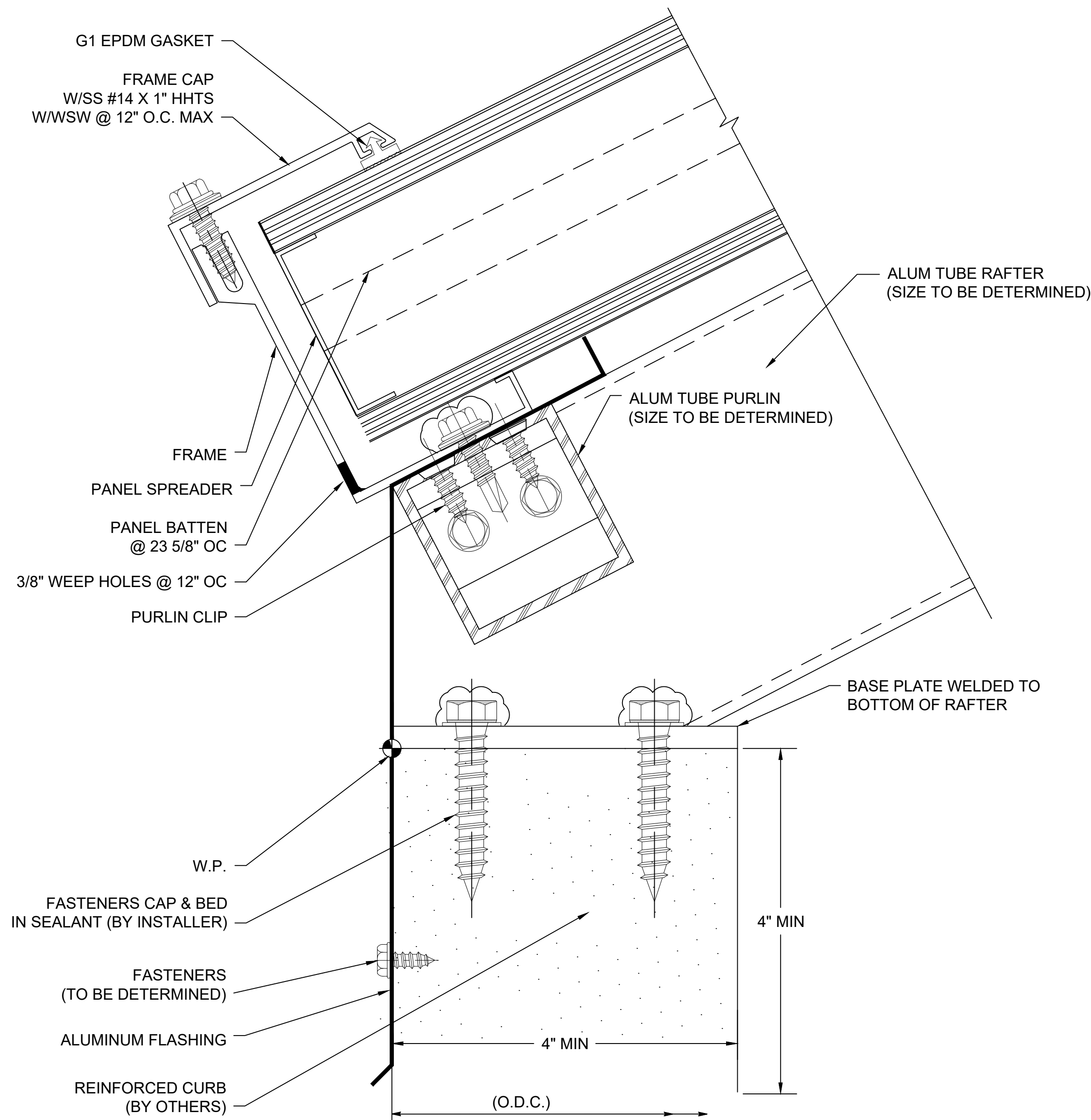
D SECTION @ SILL (FLAT CURB) 2.75" QuadSpan™ SYSTEM (4" QuadSpan™ SYSTEM SIMILAR)
