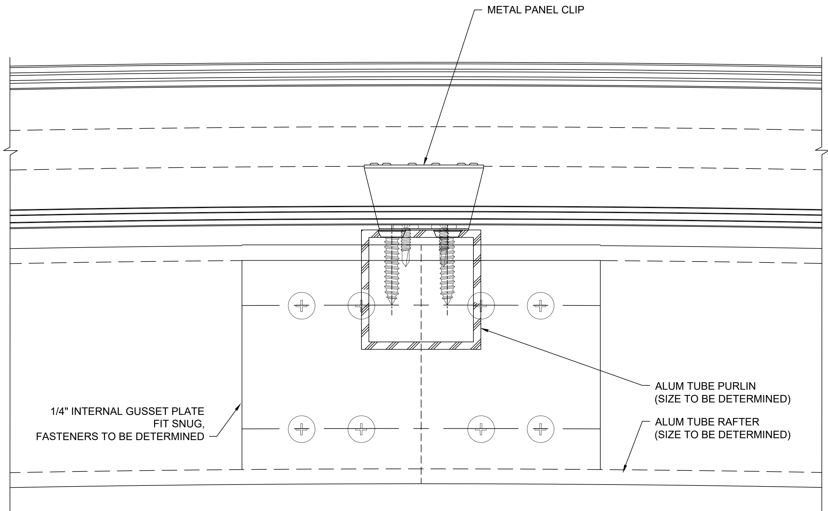
U SECTION @ APEX (W/ GUSSET PLATES) 2.75" QuadSpan™ SYSTEM (4" QuadSpan™ SYSTEM SIMILAR)
