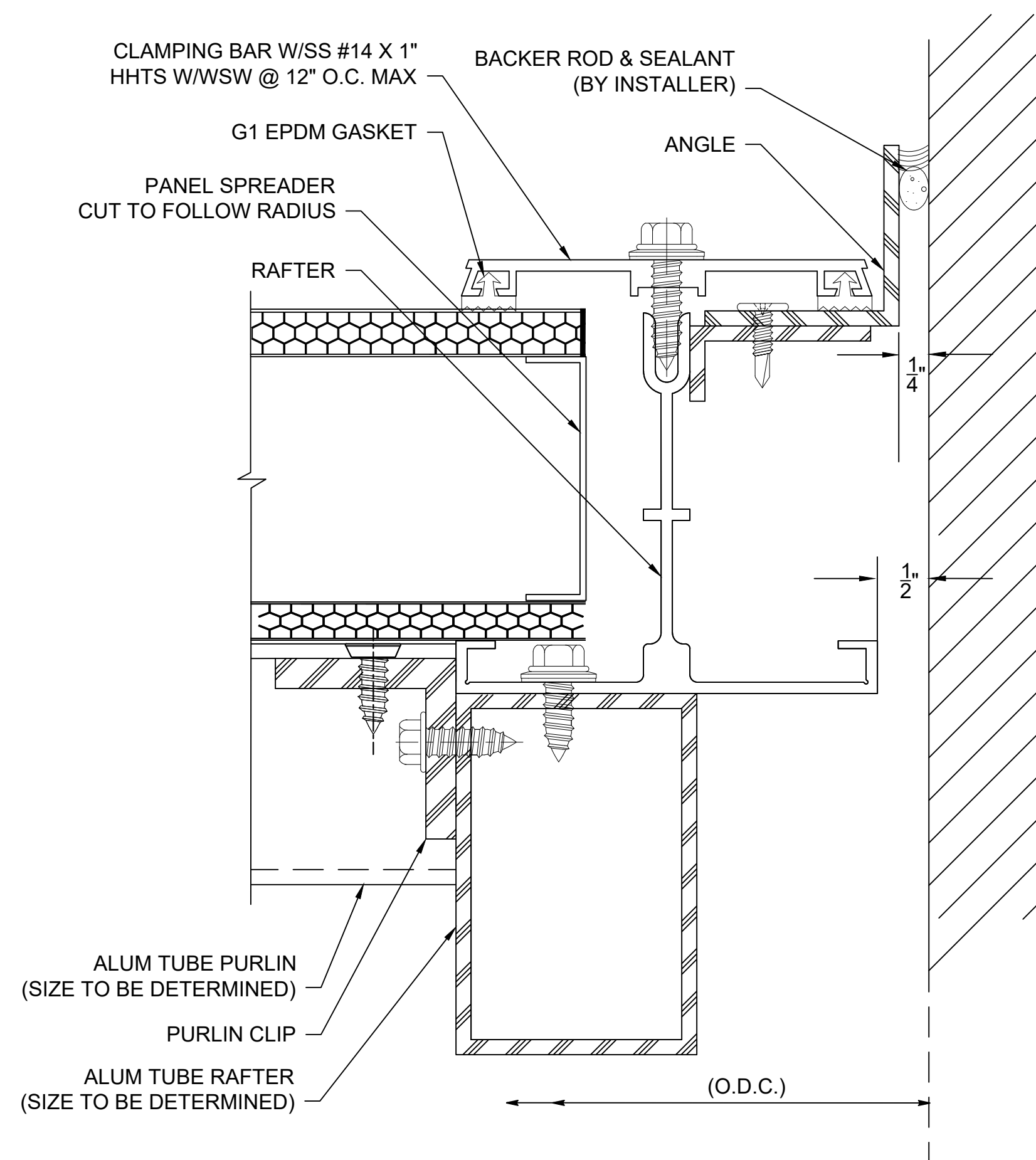
Y SECTION @ WALL END 2.75" QuadSpan™ SYSTEM (4" QuadSpan™ SYSTEM SIMILAR)
