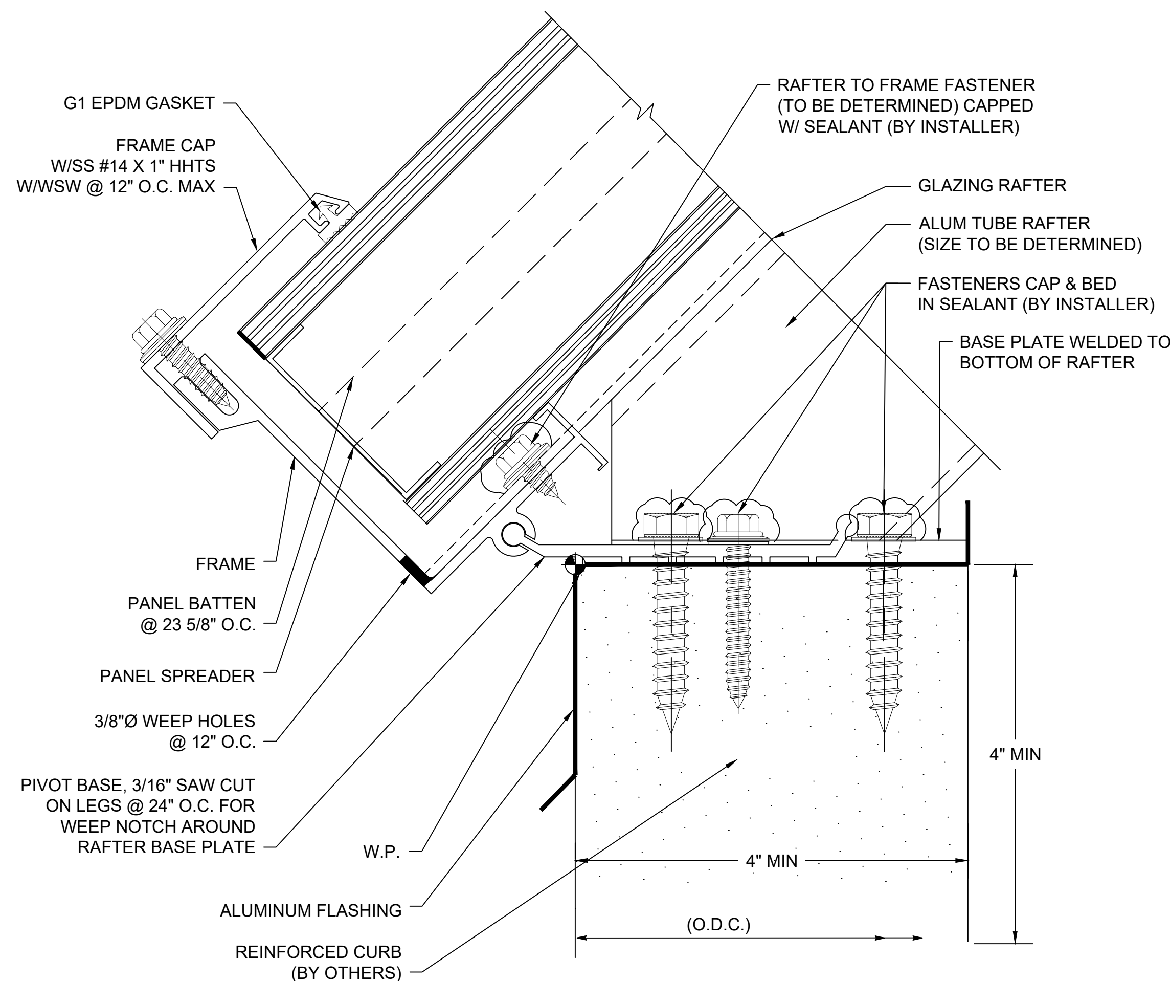
A SECTION @ SILL (FLAT CURB) 2.75" QuadSpan™ SYSTEM (4" QuadSpan™ SYSTEM SIMILAR)
