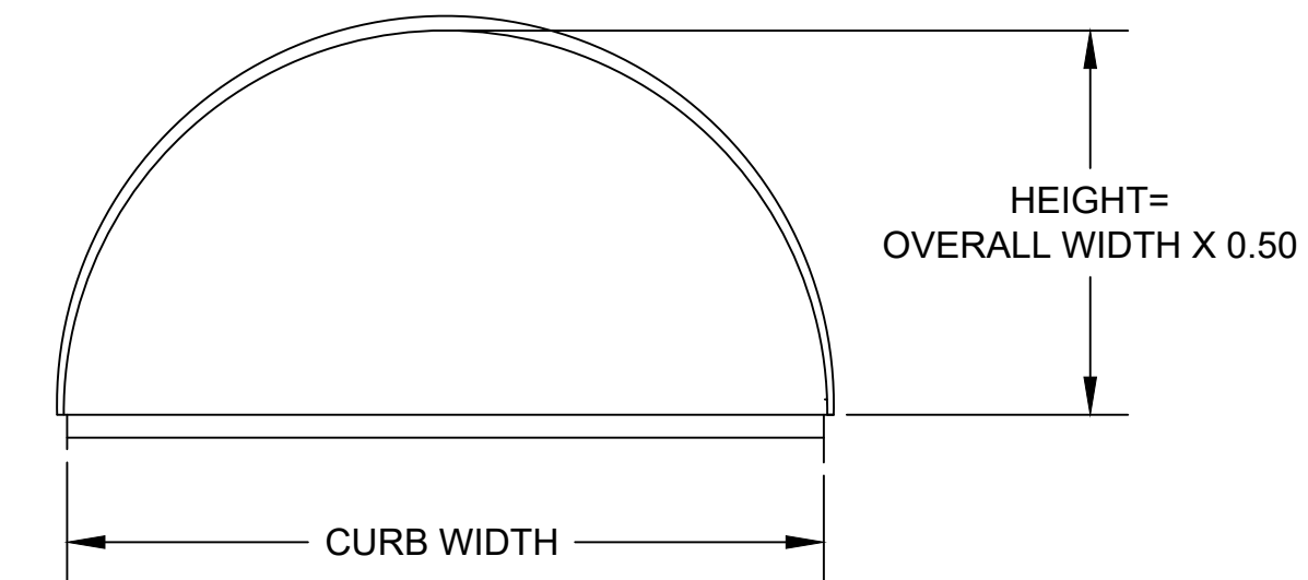
HALF ROUND ELEVATION
