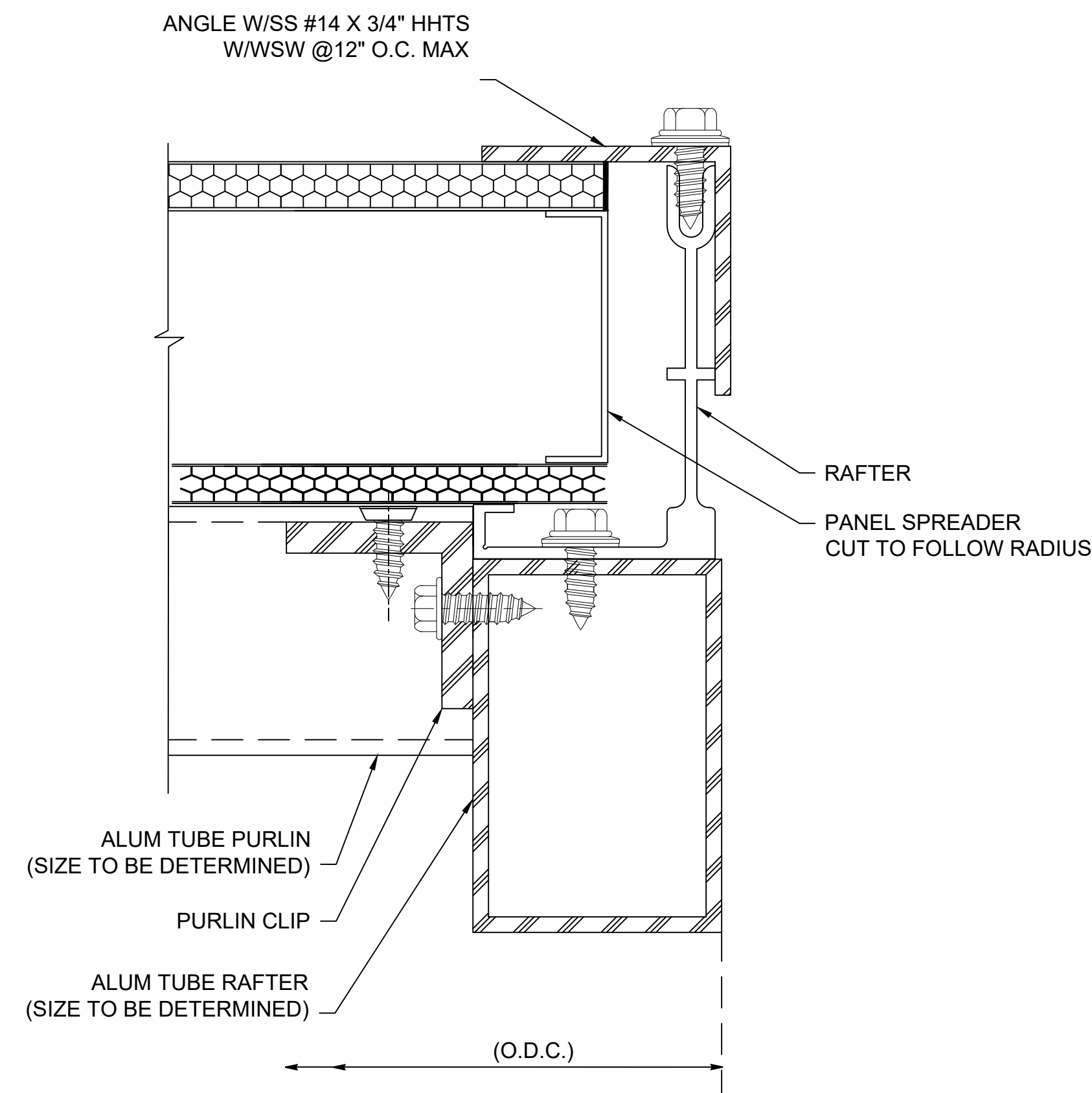
X SECTION @ OPEN END 2.75" QuadSpan™ SYSTEM (4" QuadSpan™ SYSTEM SIMILAR)
