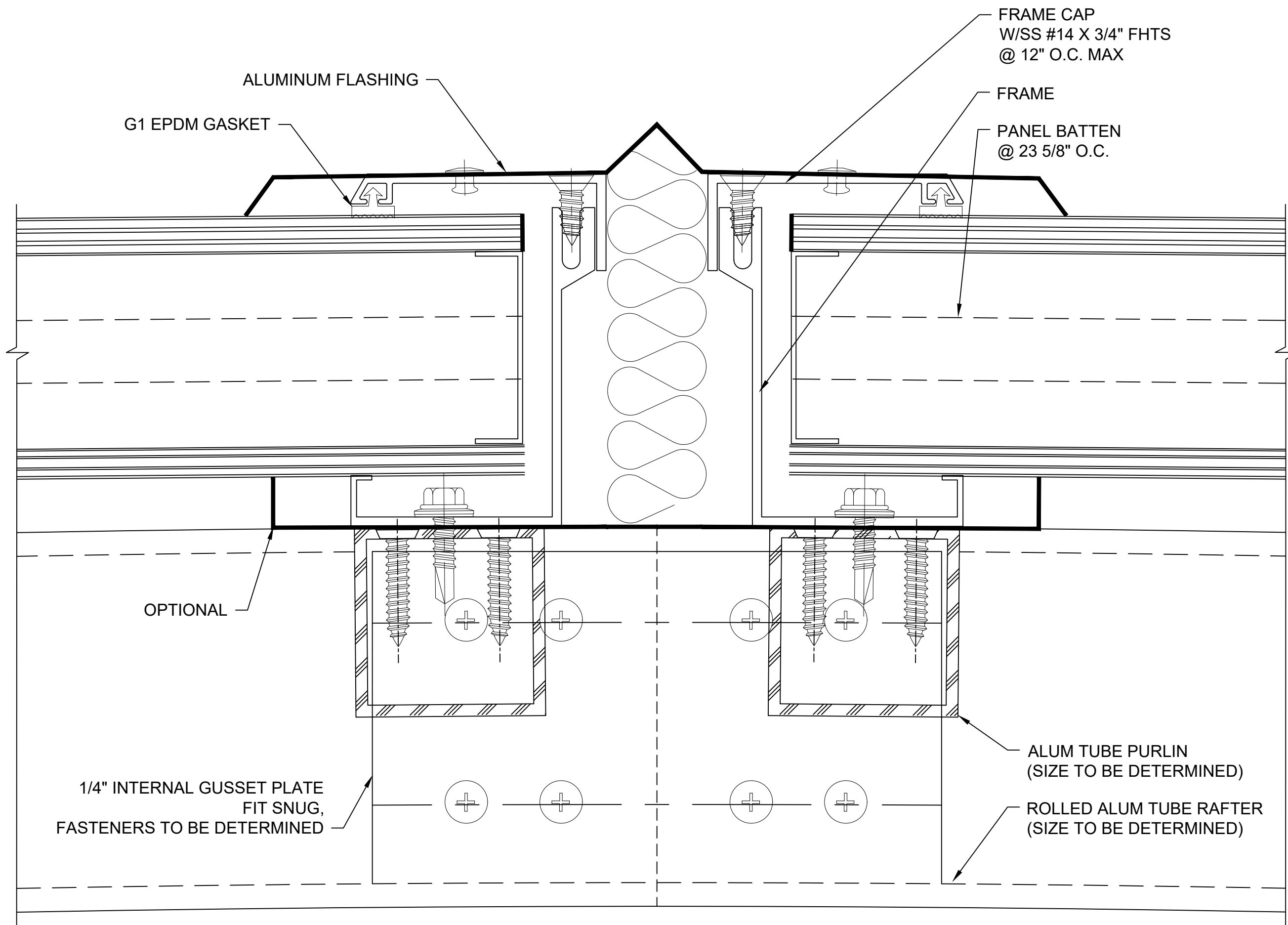
T SECTION @ APEX (W/ GUSSET PLATES) 2.75" QuadSpan™ SYSTEM (4" QuadSpan™ SYSTEM SIMILAR)
