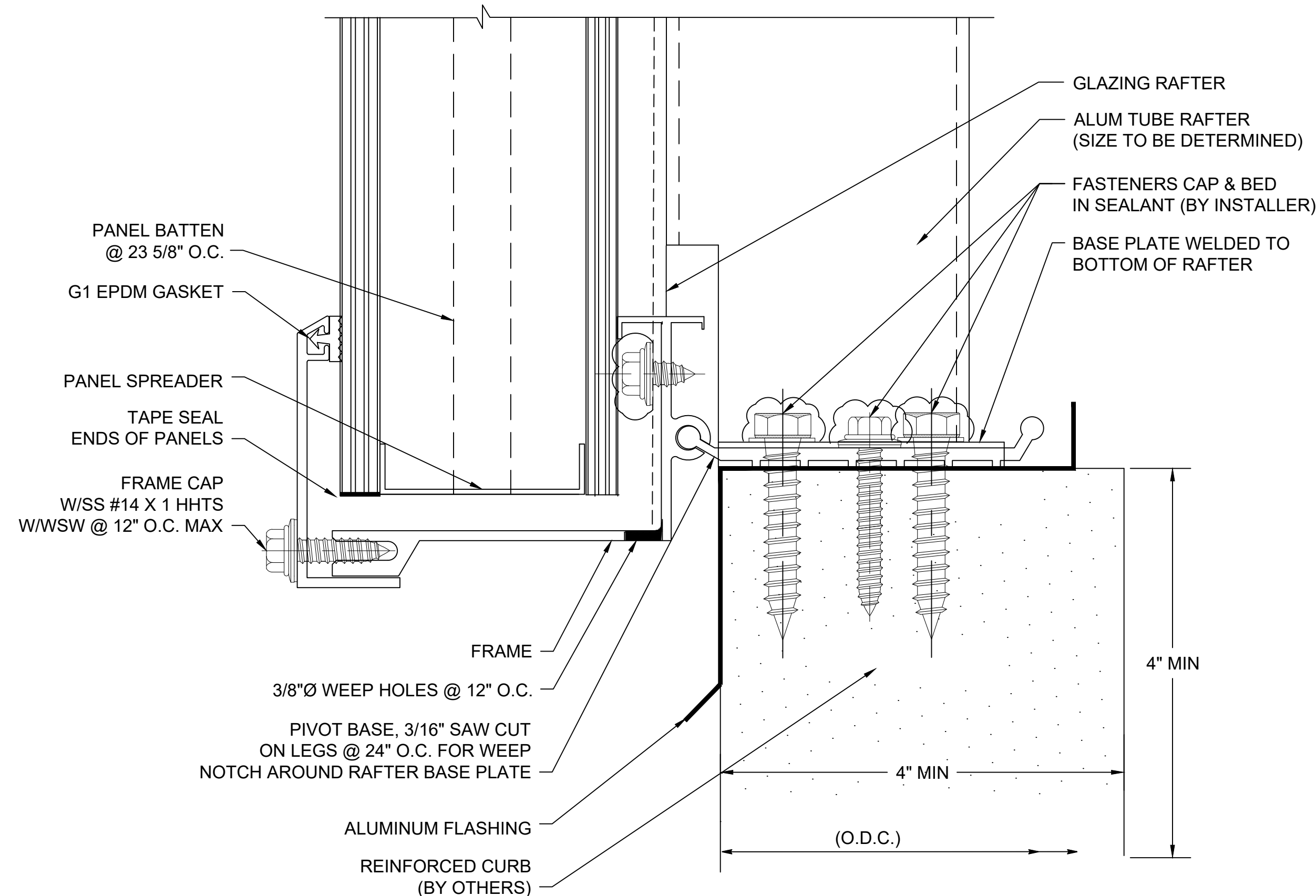
B SECTION @ SILL (HALF ROUND) 2.75" QuadSpan™ SYSTEM (4" QuadSpan™ SYSTEM SIMILAR)
