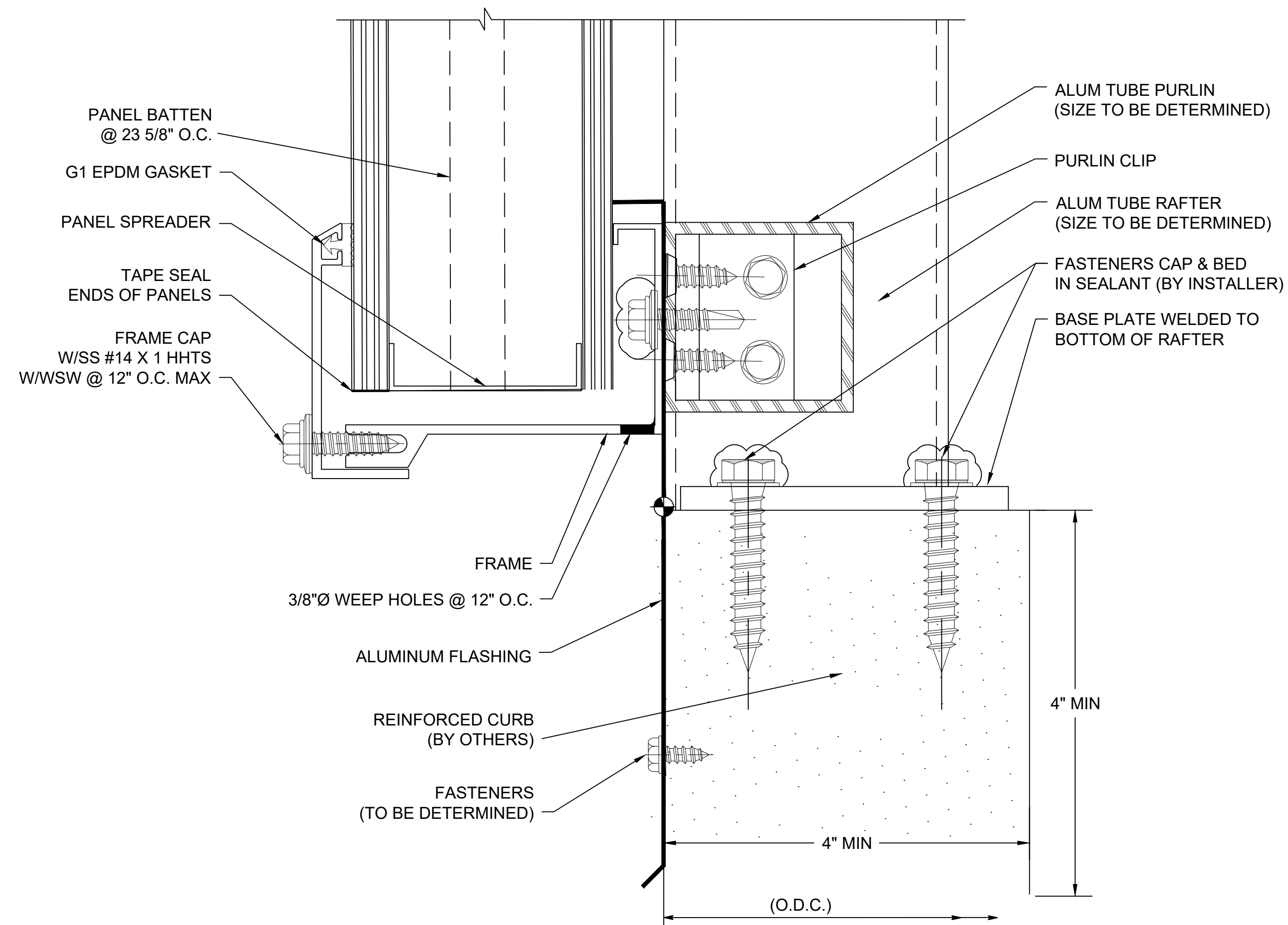
E SECTION @ SILL (HALF ROUND) 2.75" QuadSpan™ SYSTEM (4" QuadSpan™ SYSTEM SIMILAR)
