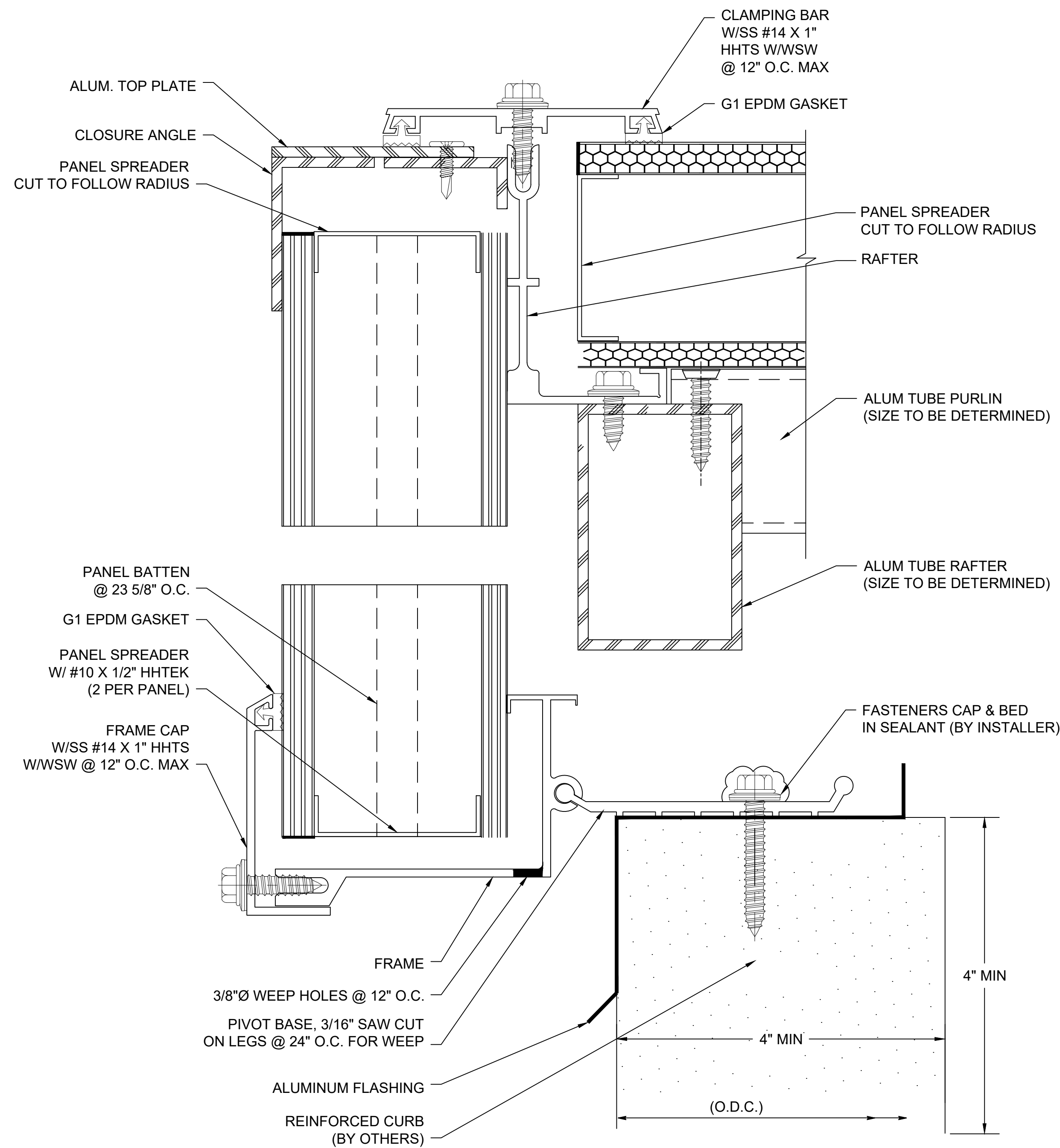
W SECTION @ GABLE END 2.75" QuadSpan™ SYSTEM (4" QuadSpan™ SYSTEM SIMILAR)
