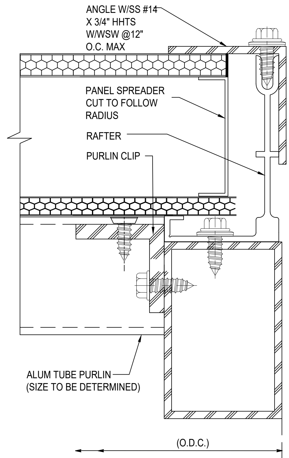
X SECTION @ OPEN END 2.75" QuadSpan™ SYSTEM (4" QuadSpan™ SYSTEM SIMILAR)
