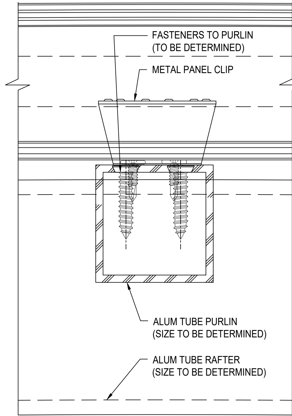
0 SECTION @ PURLINS 2.75" QuadSpan™ SYSTEM (4" QuadSpan™ SYSTEM SIMILAR)
