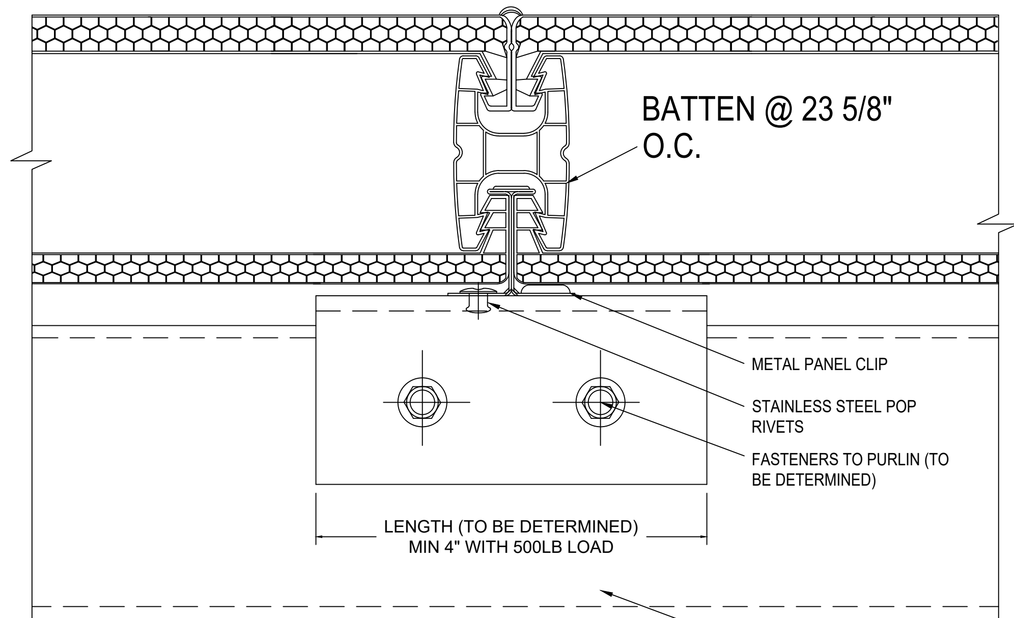
K SECTION @ BATTEN 2.75" QuadSpan™ SYSTEM (4" QuadSpan™ SYSTEM SIMILAR)
