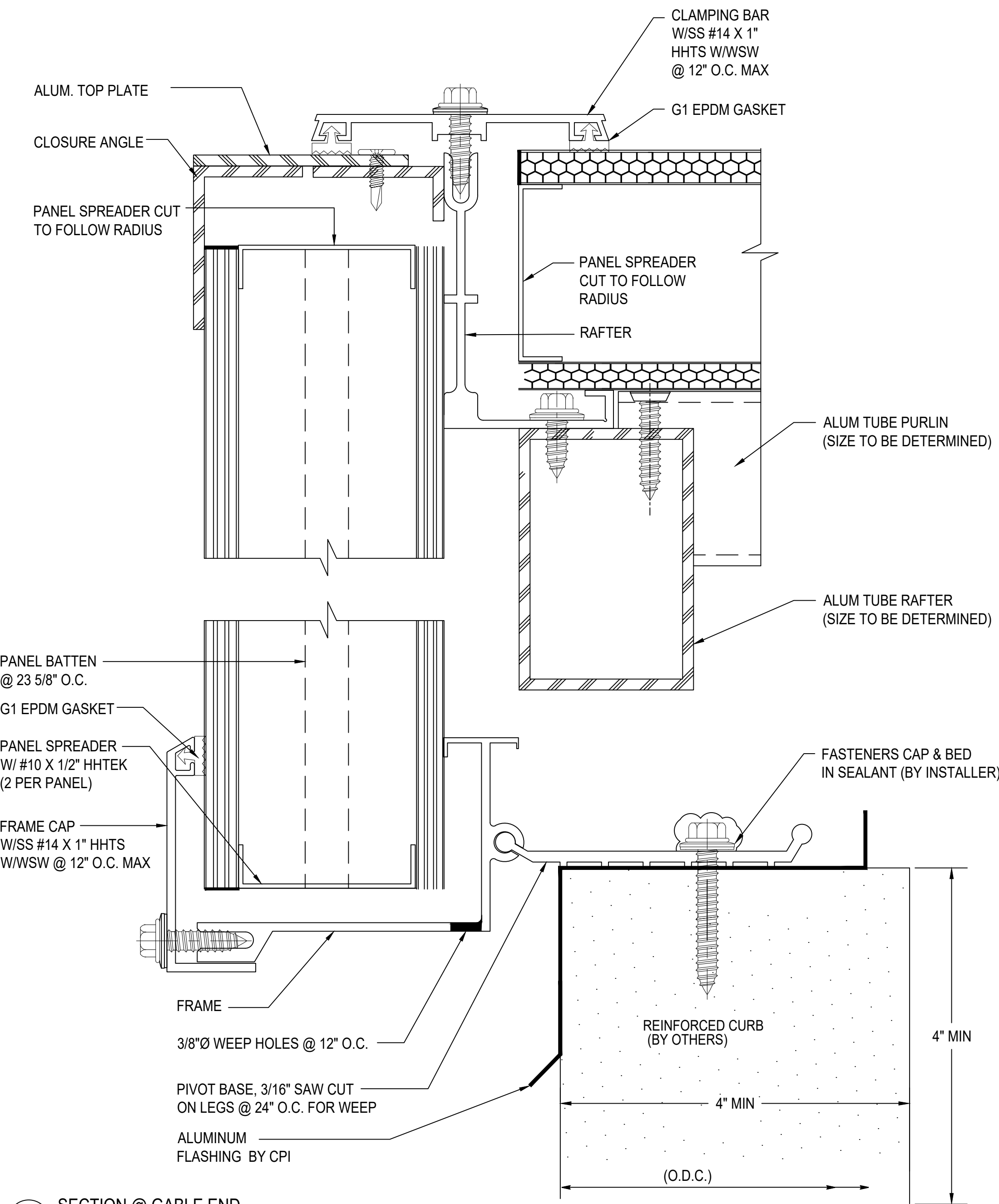
W SECTION @ GABLE END 2.75" QuadSpan™ SYSTEM (4" QuadSpan™ SYSTEM SIMILAR)
