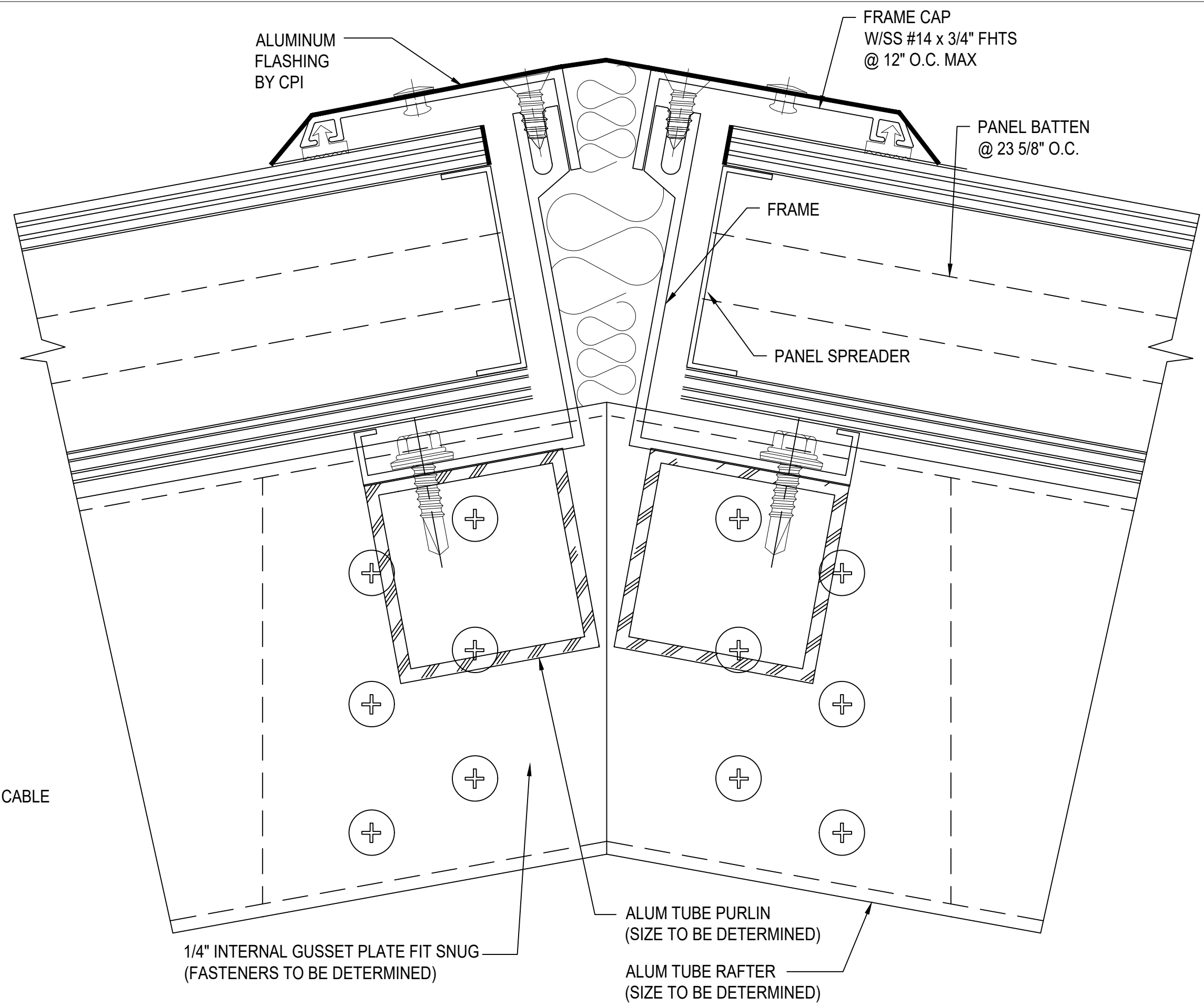
Q SECTION @ RIDGE 2.75" QuadSpan™ SYSTEM (4" QuadSpan™ SYSTEM SIMILAR)
