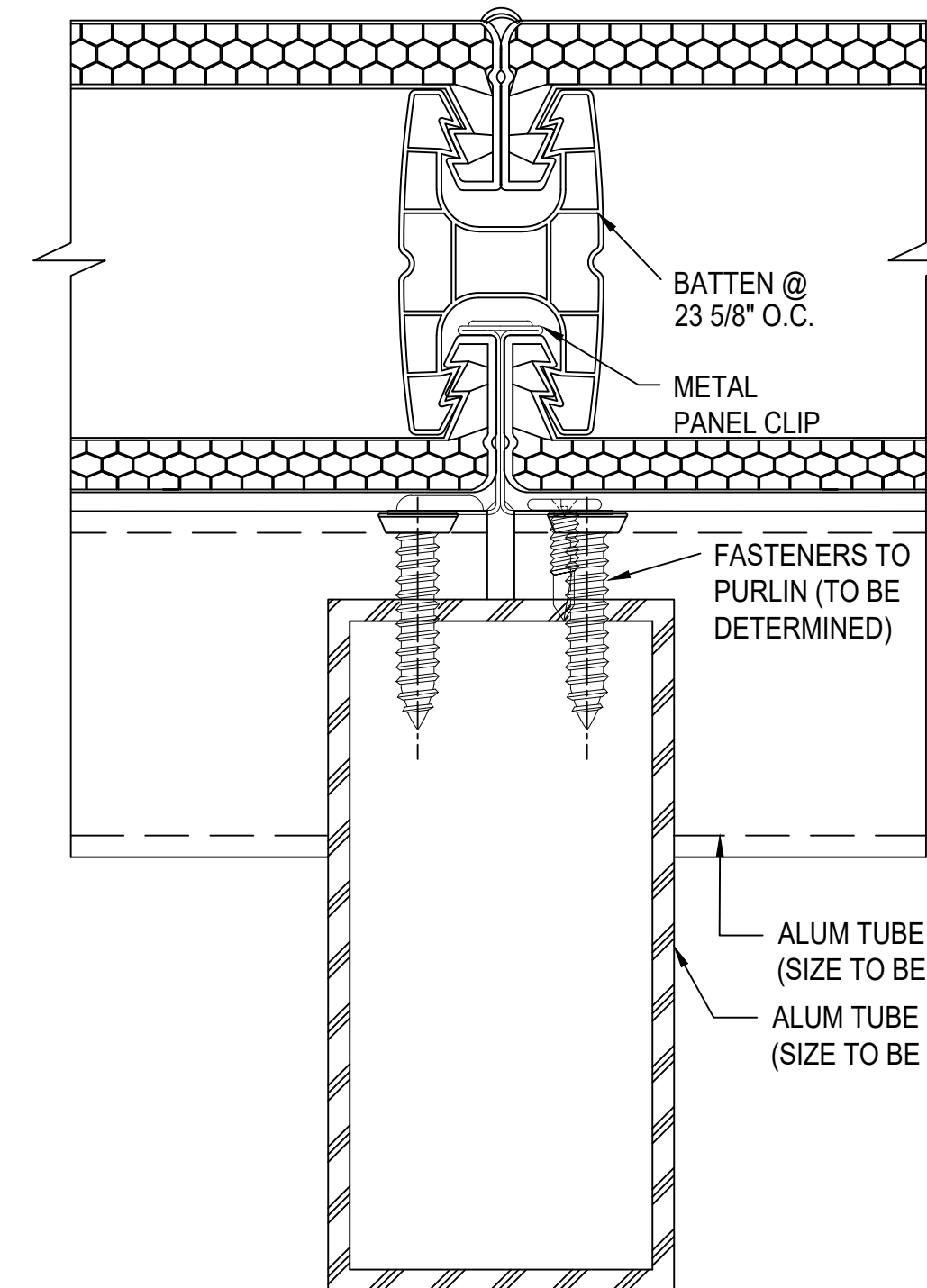
N SECTION @ RAFTER 2.75" QuadSpan™ SYSTEM (4" QuadSpan™ SYSTEM SIMILAR)
