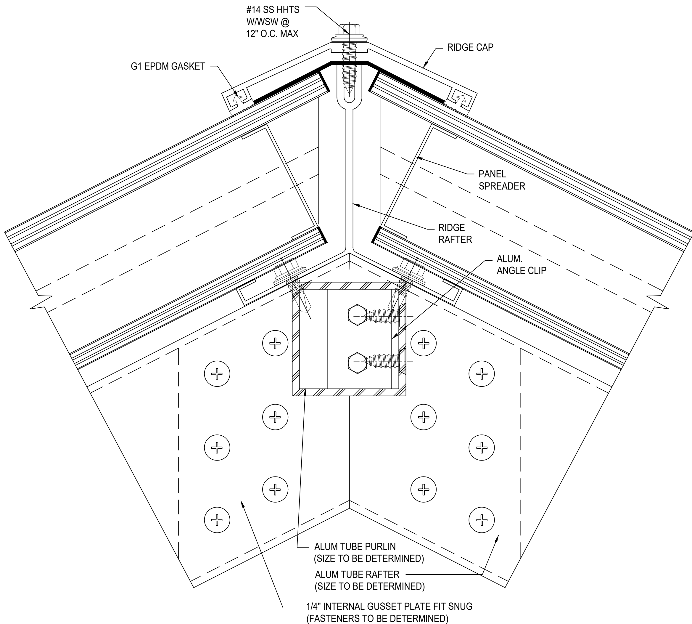
R SECTION @ RIDGE 2.75" QuadSpan™ SYSTEM (4" QuadSpan™ SYSTEM SIMILAR)
