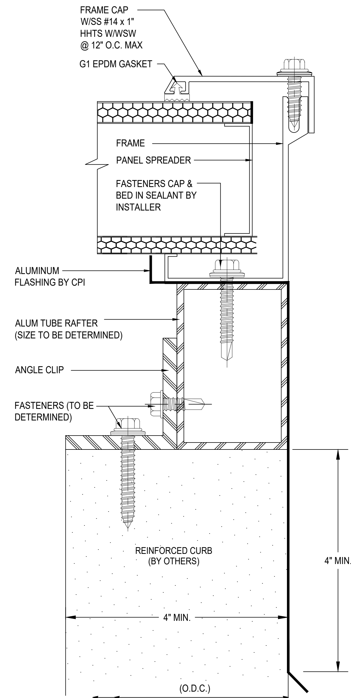
Z SECTION @ SLOPED ENDS 2.75" QuadSpan™ SYSTEM (4" QuadSpan™ SYSTEM SIMILAR) NOTE: FOR SADDLE RIDGE ONLY
