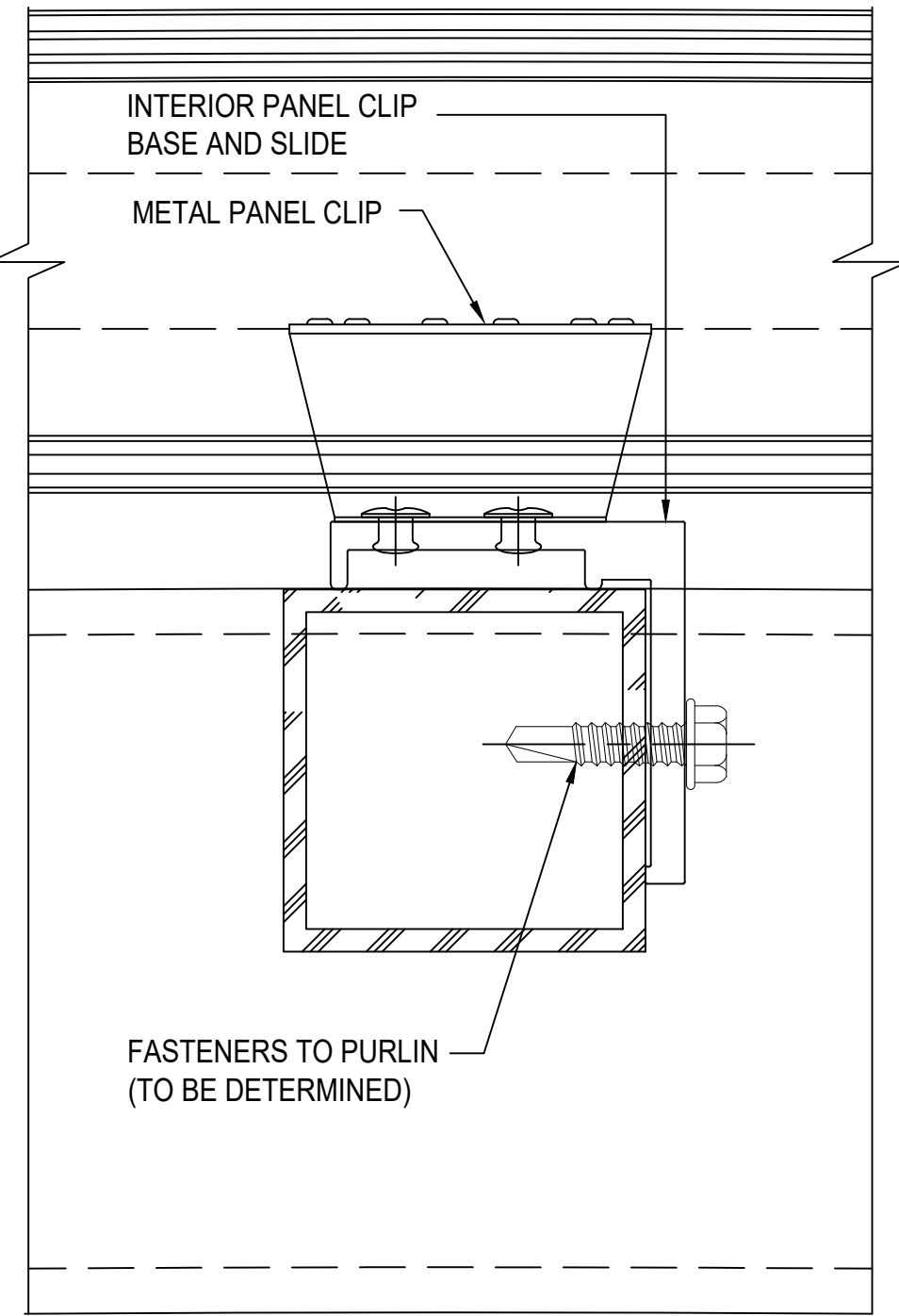
02 SECTION @ PURLINS 2.75" QuadSpan™ SYSTEM (4" QuadSpan™ SYSTEM SIMILAR)
