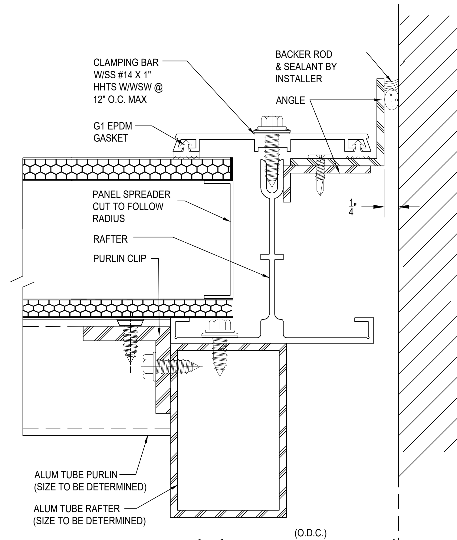
Y SECTION @ WALL END 2.75" QuadSpan™ SYSTEM (4" QuadSpan™ SYSTEM SIMILAR)
