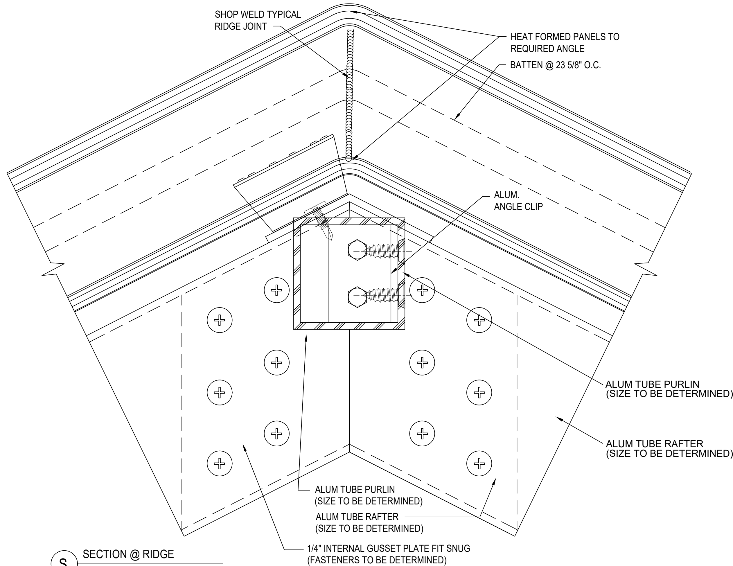
S SECTION @ RIDGE 2.75" QuadSpan™ SYSTEM (4" QuadSpan™ SYSTEM SIMILAR)
