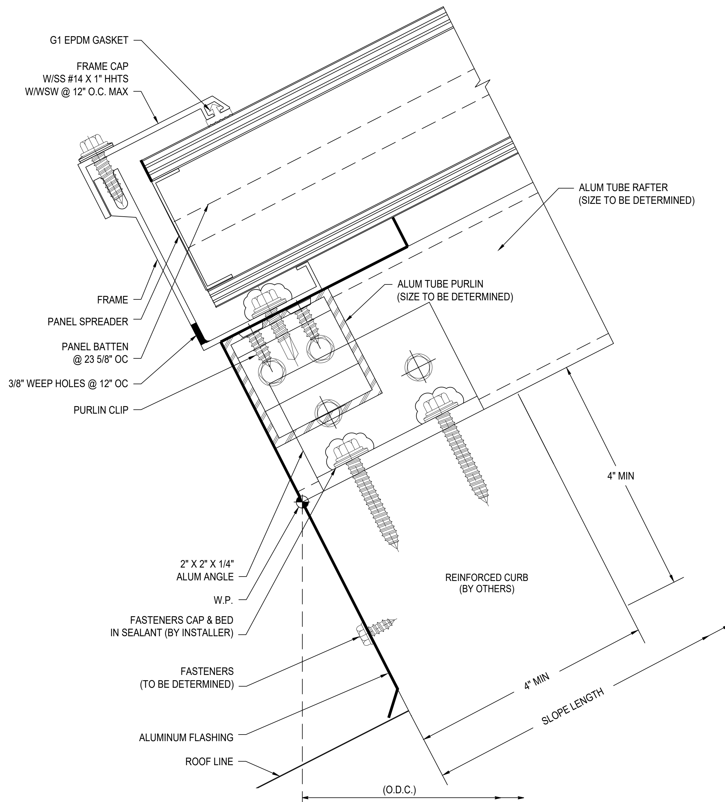
F SECTION @ SILL (TILTED CURB) 2.75" QuadSpan™ SYSTEM (4" QuadSpan™ SYSTEM SIMILAR)
