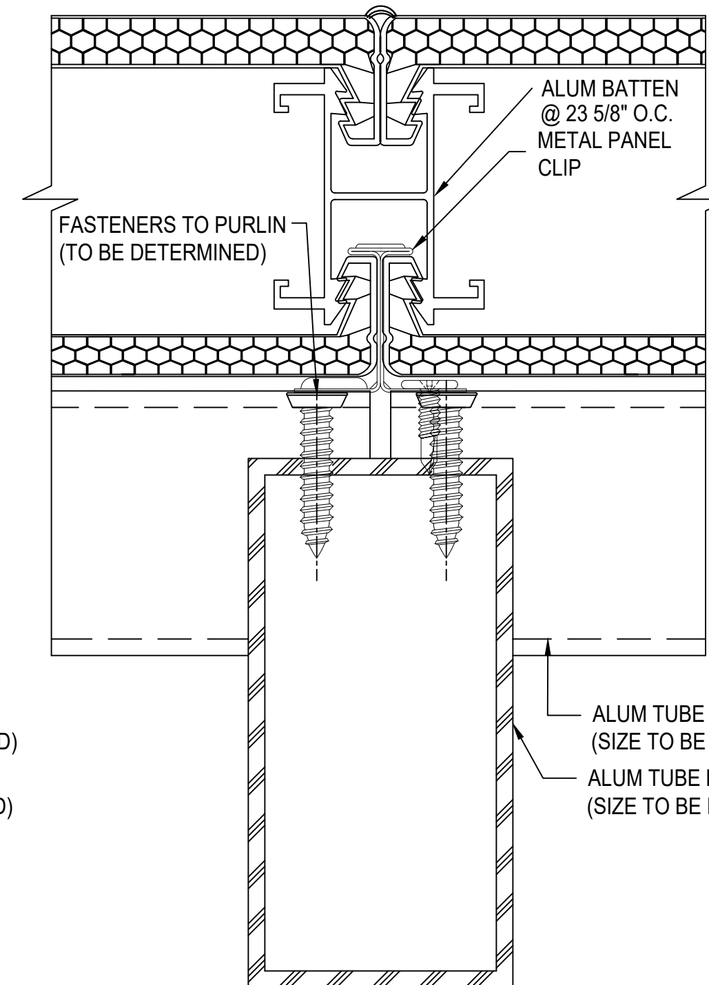
N 2 SECTION @ RAFTER 2.75" QuadSpan™ SYSTEM (4" QuadSpan™ SYSTEM SIMILAR)
