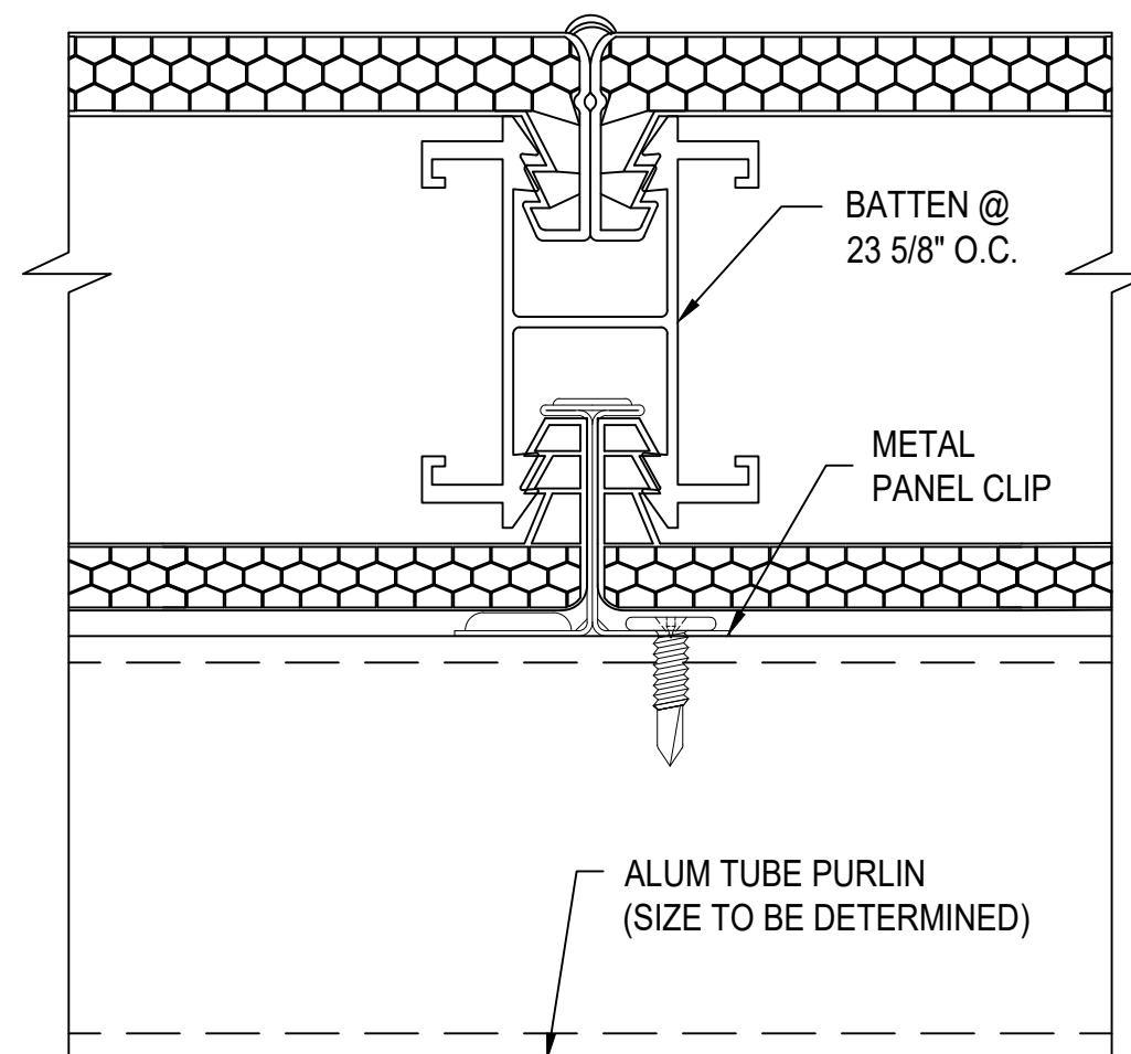
L 2 SECTION @ BATTEN 2.75" QuadSpan™ SYSTEM
