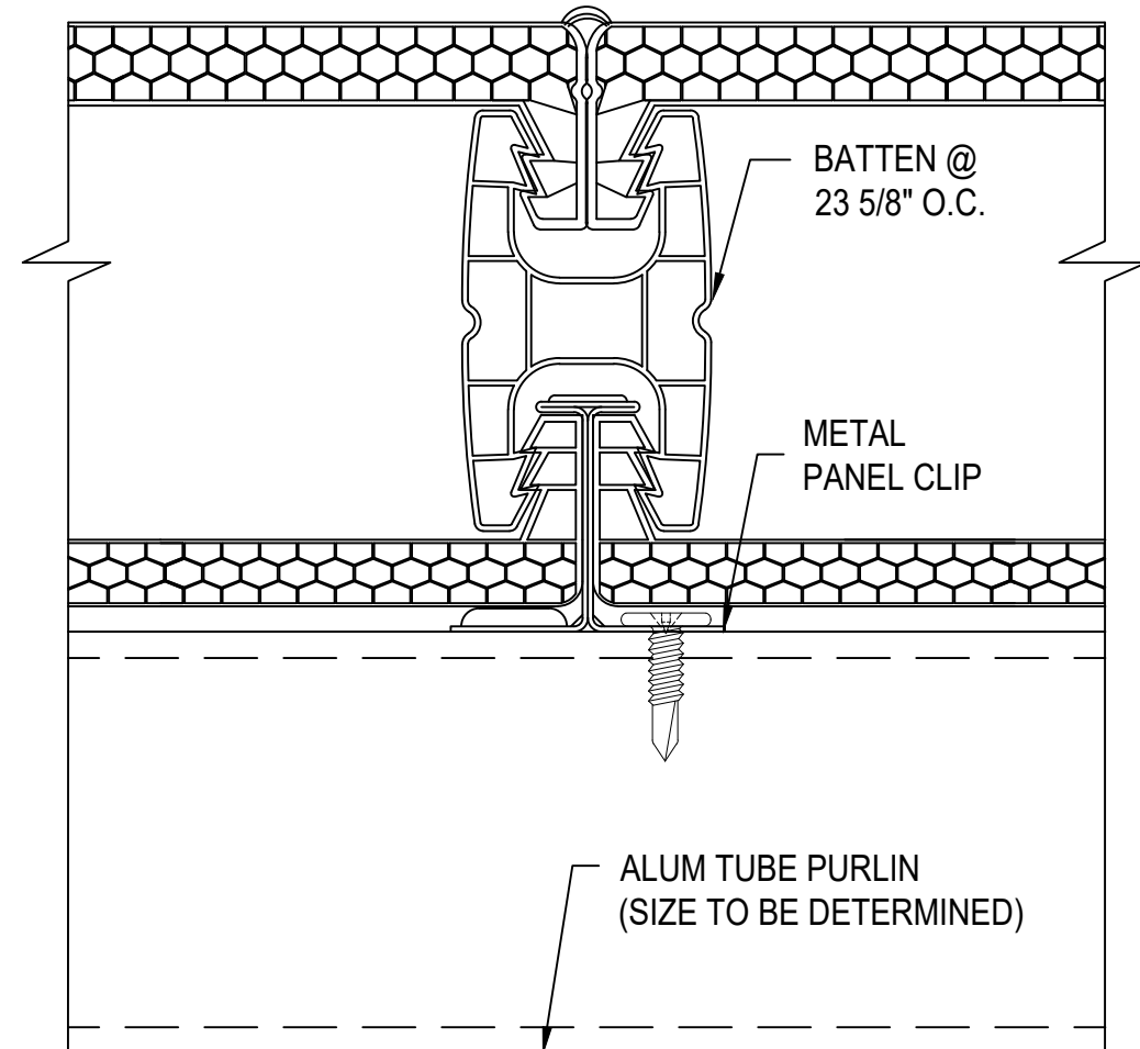
L SECTION @ BATTEN 2.75" QuadSpan™ SYSTEM
