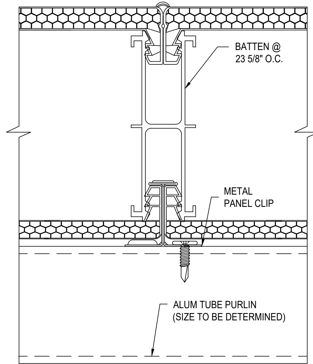
L 3 SECTION @ BATTEN 4" QuadSpan™ SYSTEM NOTE: THESE DETAILS OCCUR WHEN GLAZING IS SHIPPED KNOCKED DOWN.
