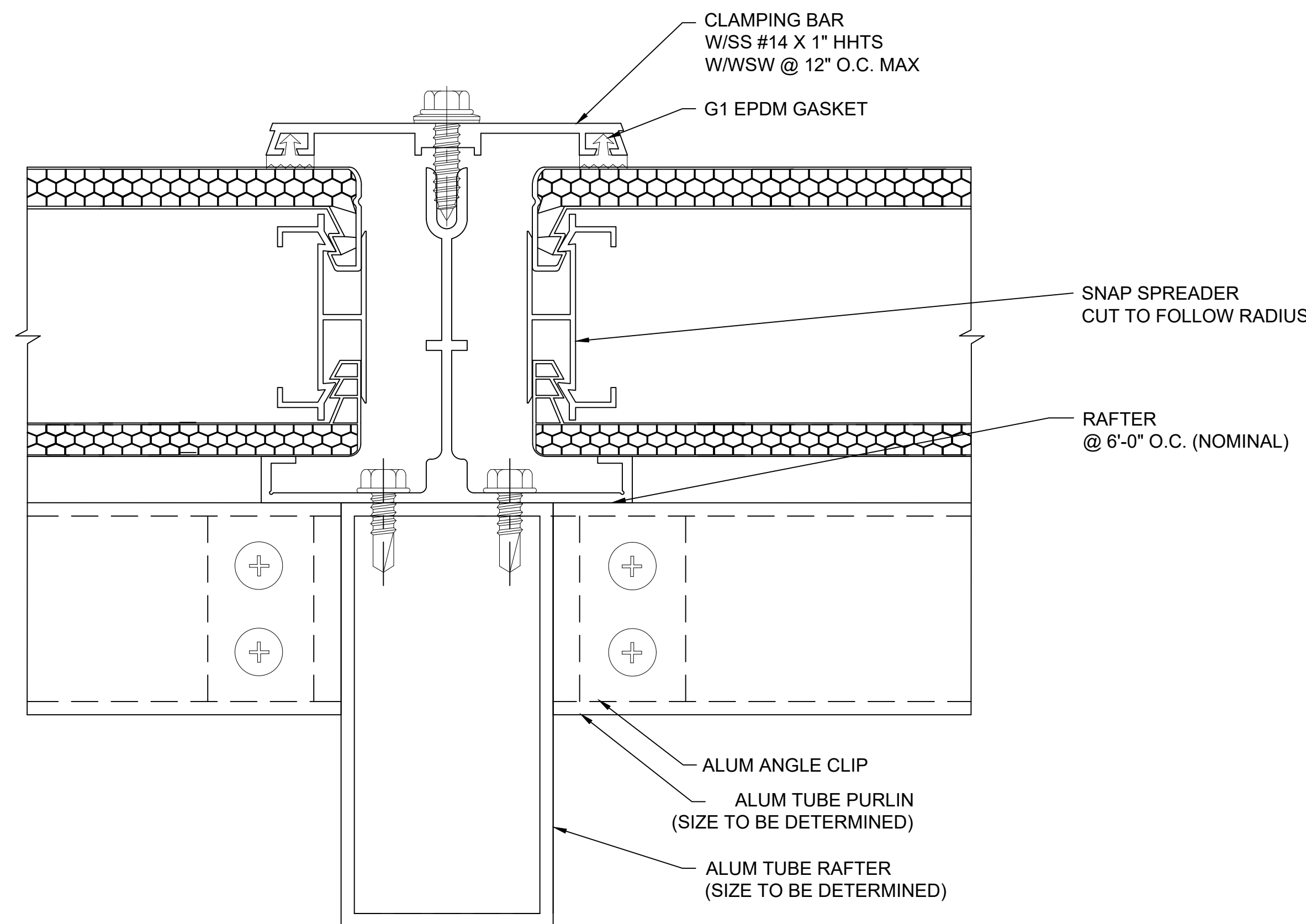
M SECTION @ RAFTER 2.75" QuadSpan™ SYSTEM (4" QuadSpan™ SYSTEM SIMILAR)
