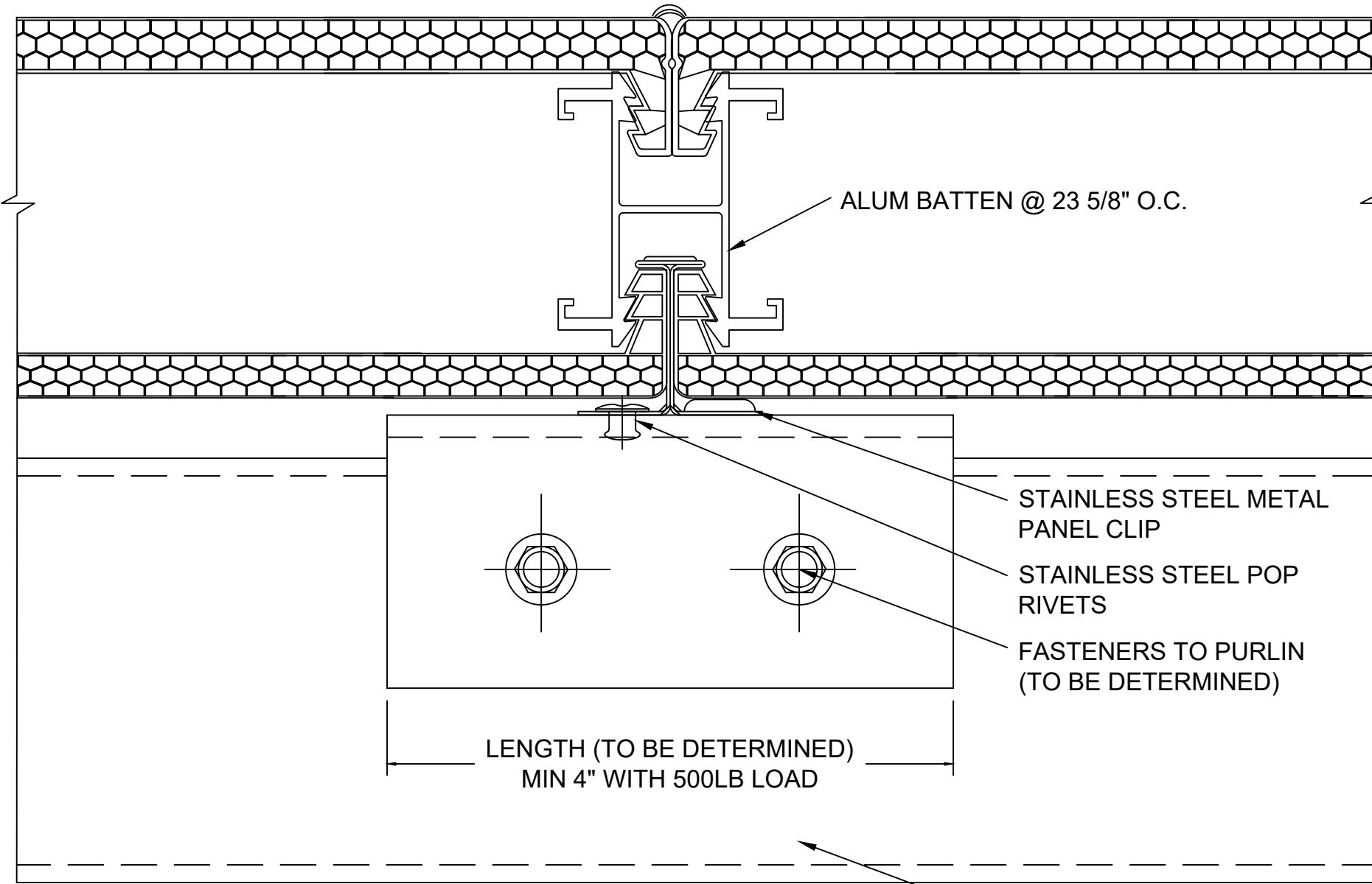
K 2 SECTION @ BATTEN 2.75" QuadSpan™ SYSTEM (4" QuadSpan™ SYSTEM SIMILAR)
