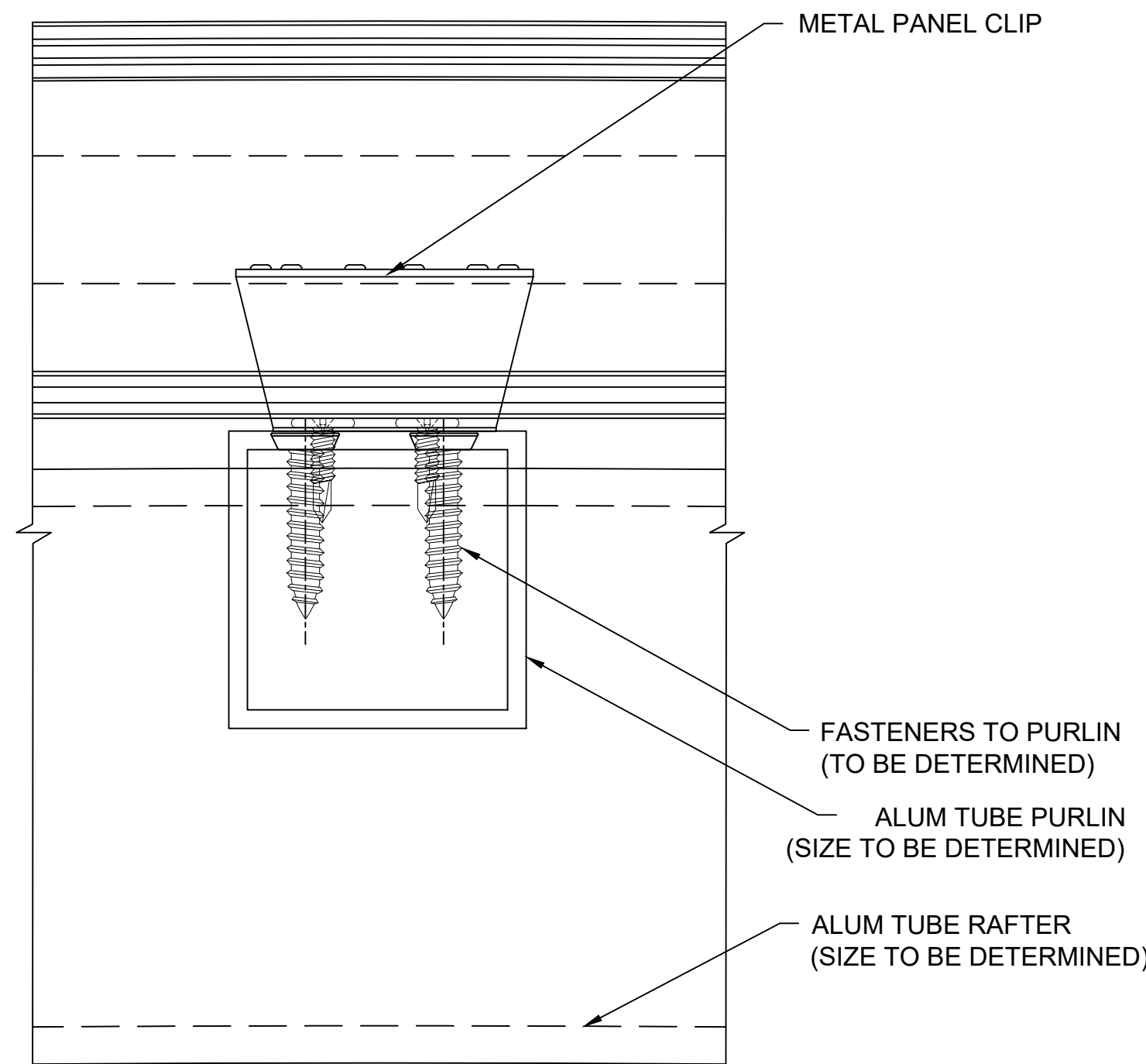
O SECTION @ PURLINS 2.75" QuadSpan™ SYSTEM (4" QuadSpan™ SYSTEM SIMILAR)
