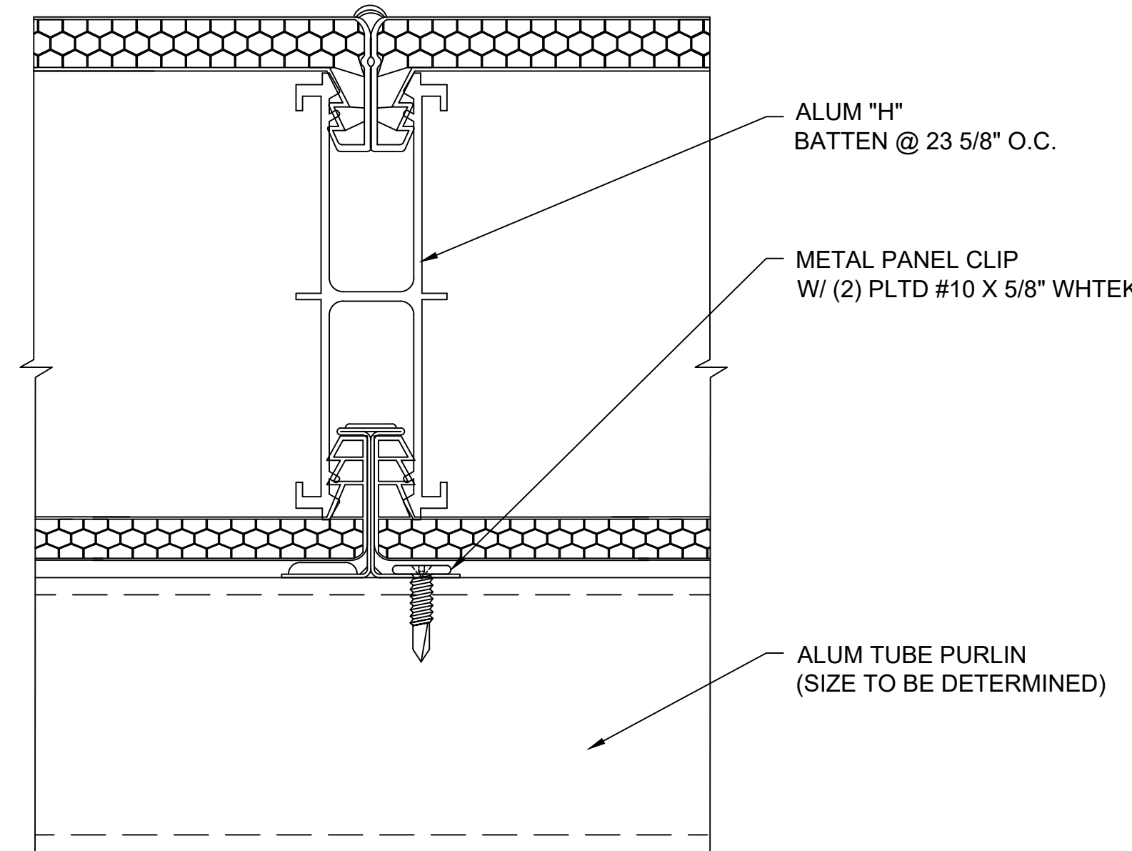
L 3 SECTION @ BATTEN 4" QuadSpan™ SYSTEM
