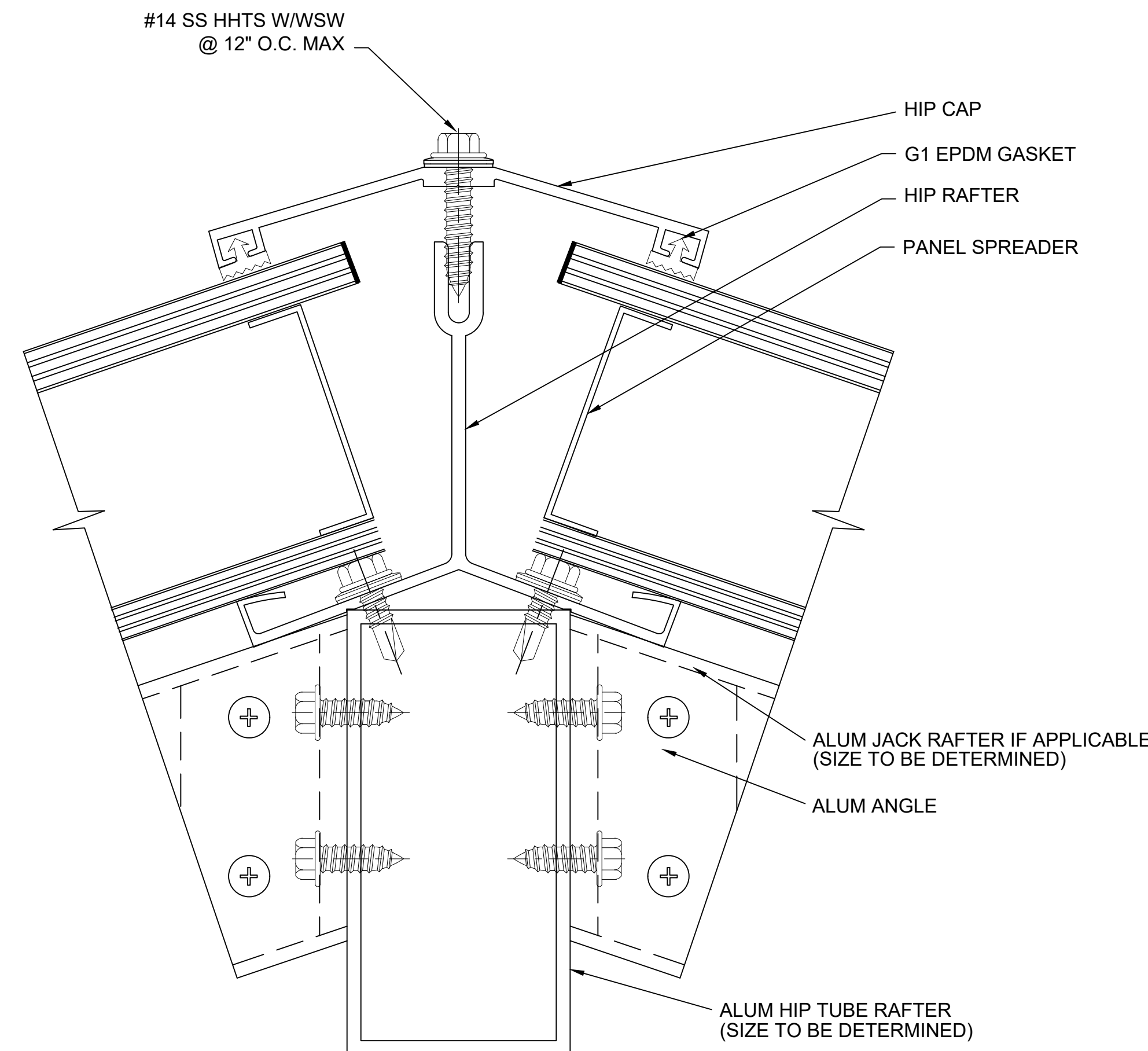
P SECTION @ HIP 2.75" QuadSpan™ SYSTEM (4" QuadSpan™ SYSTEM SIMILAR)
