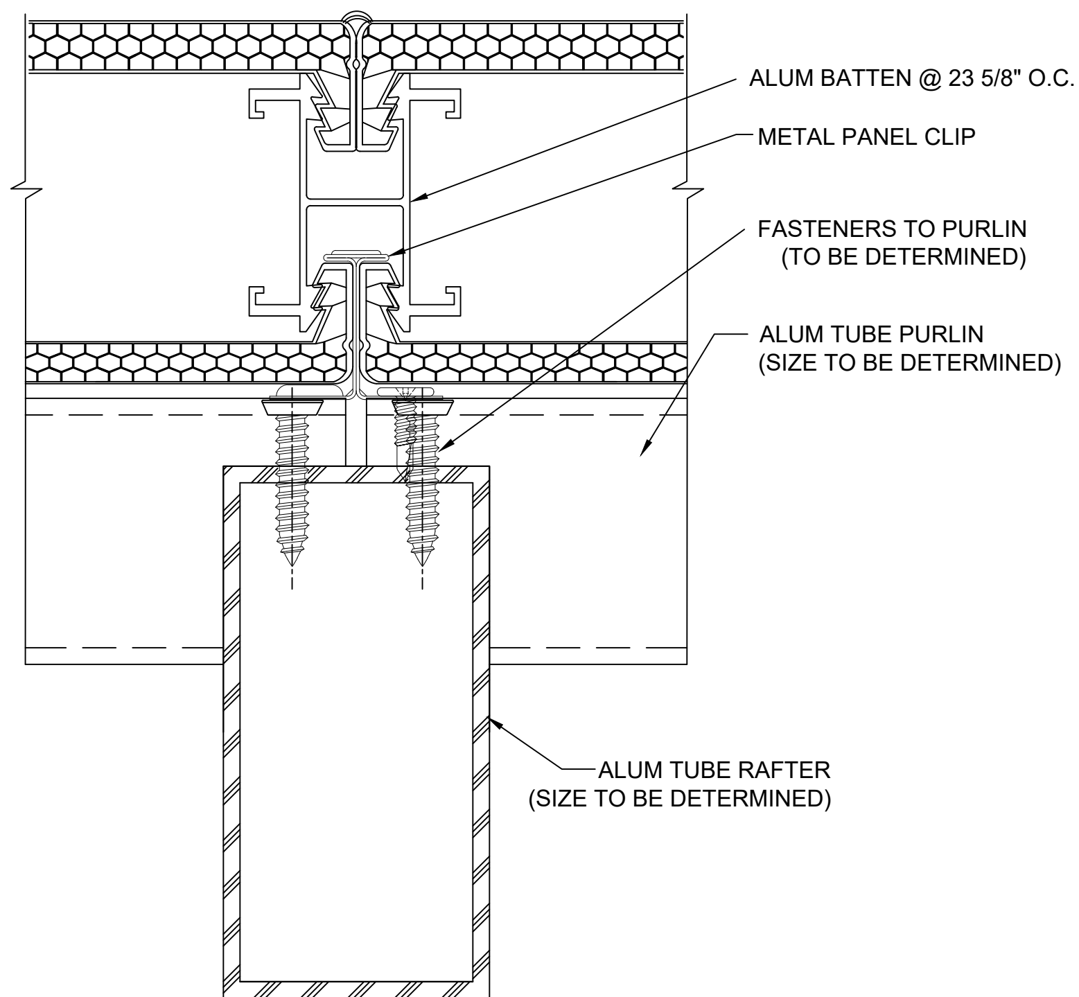
N 2 SECTION @ RAFTER 2.75" QuadSpan™ SYSTEM (4" QuadSpan™ SYSTEM SIMILAR)
