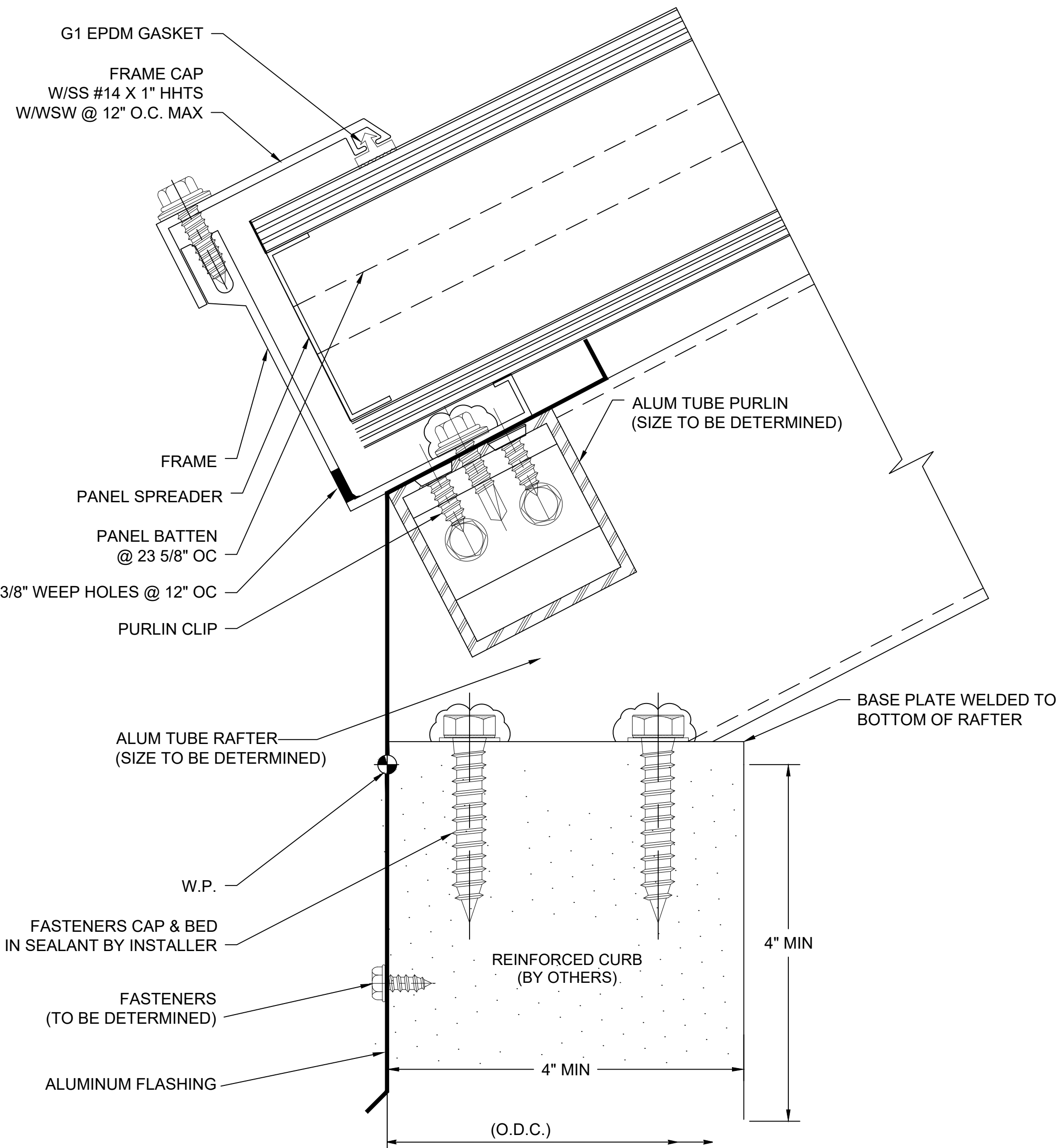
D SECTION @ SILL (FLAT CURB) 2.75" QuadSpan™ SYSTEM (4" QuadSpan™ SYSTEM SIMILAR)
