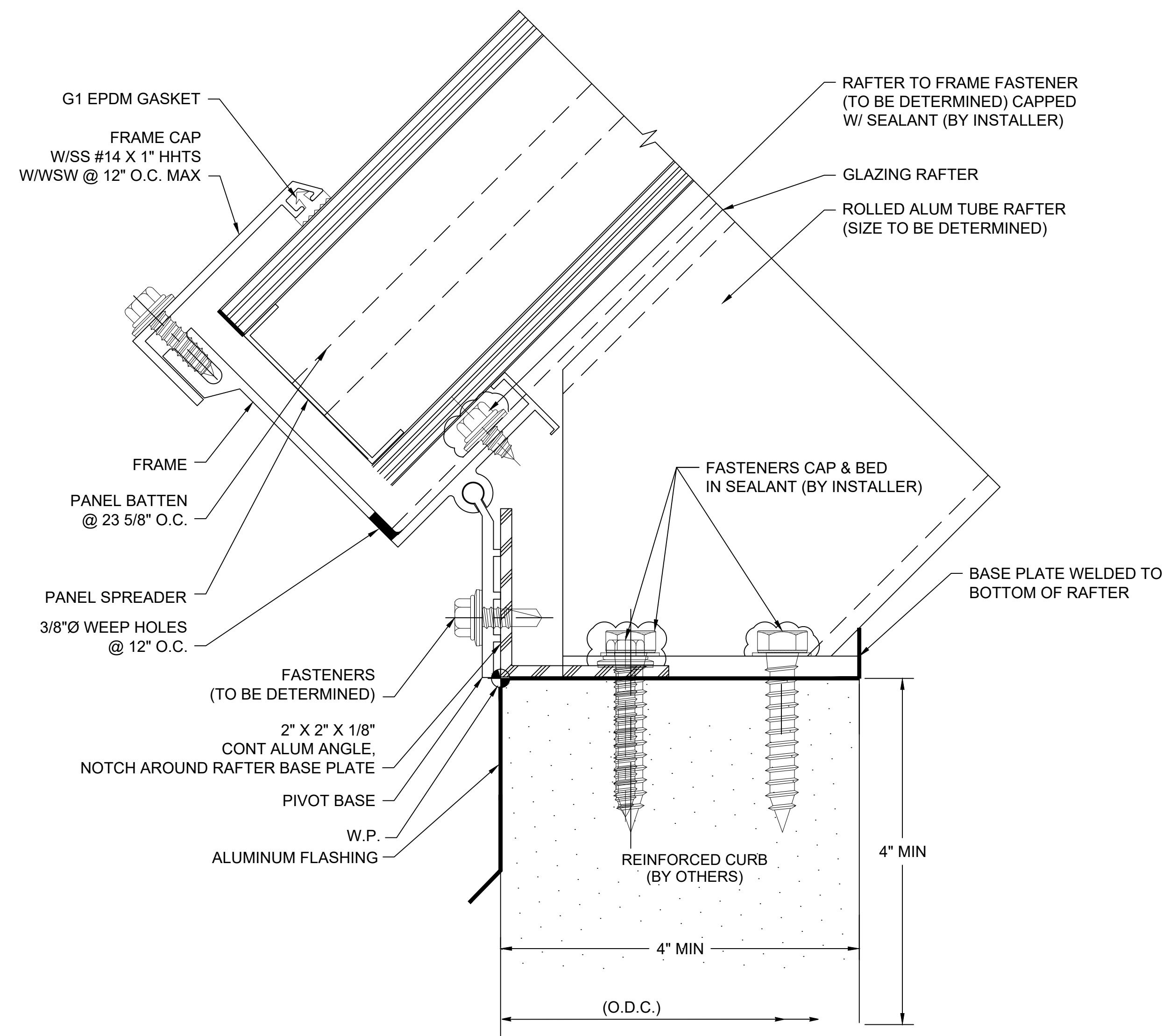
C SECTION @ SILL (FLAT CURB) 2.75" QuadSpan™ SYSTEM (4" QuadSpan™ SYSTEM SIMILAR)
