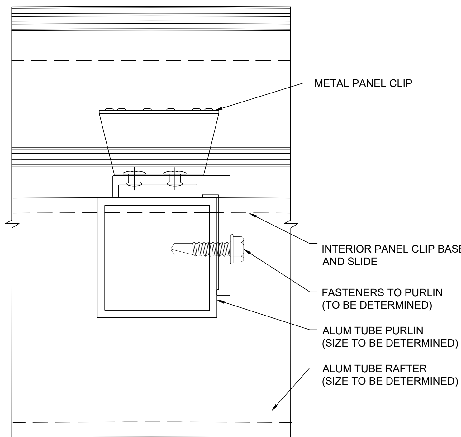
O 2 SECTION @ PURLINS 2.75" QuadSpan™ SYSTEM (4" QuadSpan™ SYSTEM SIMILAR)
