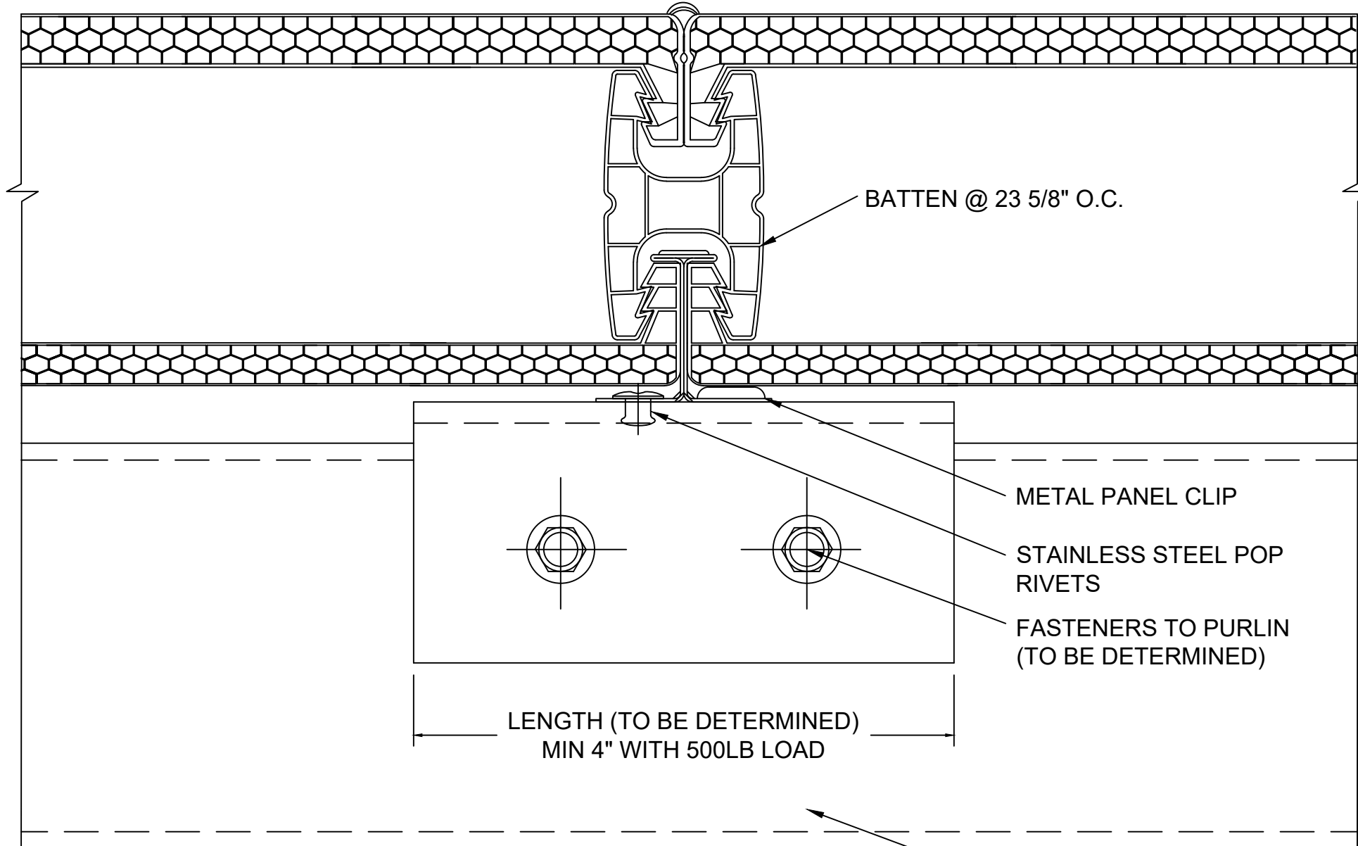
K SECTION @ BATTEN 2.75" QuadSpan™ SYSTEM (4" QuadSpan™ SYSTEM SIMILAR)
