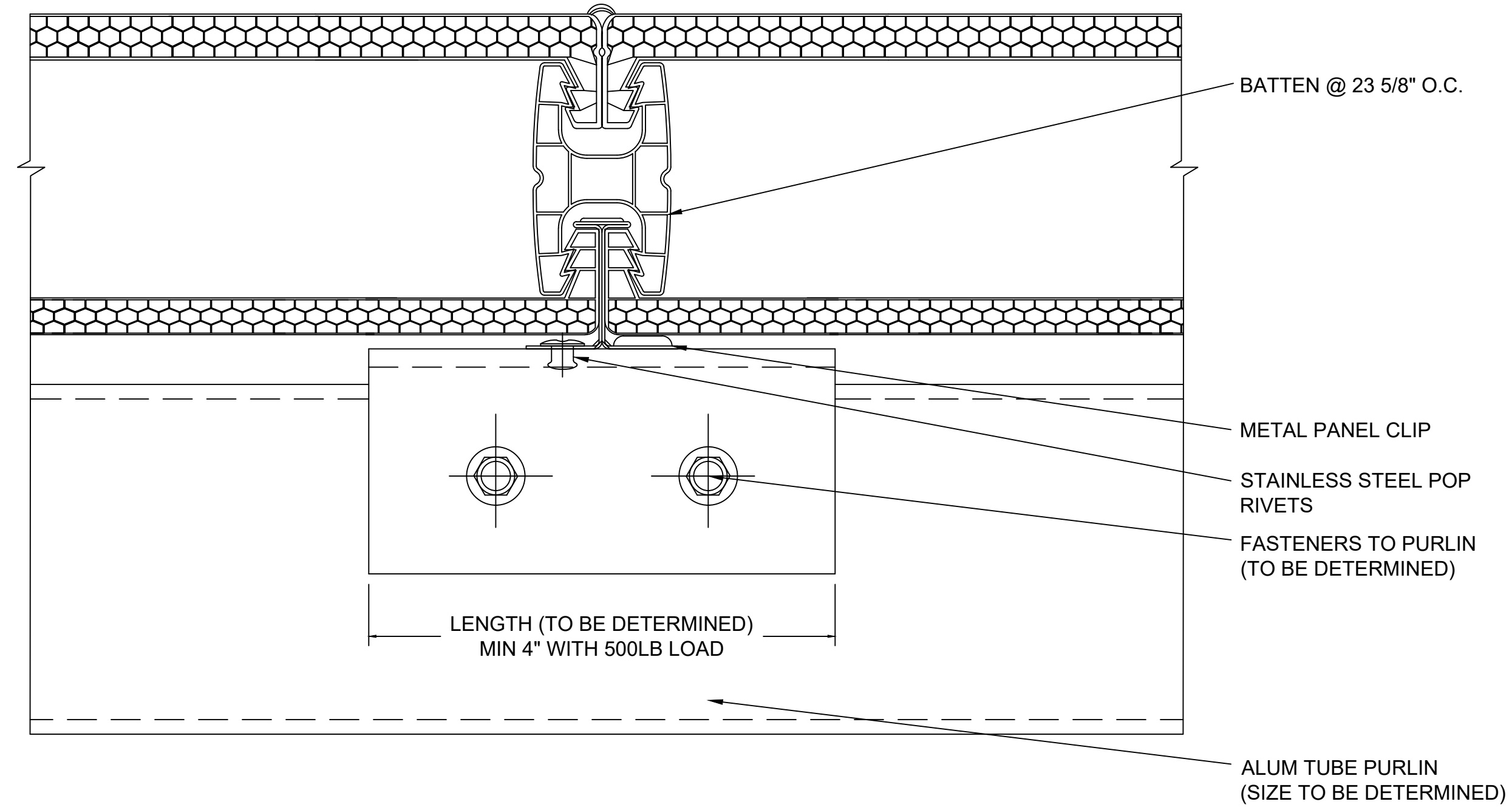
K SECTION @ BATTEN 2.75" QuadSpan™ SYSTEM (4" QuadSpan™ SYSTEM SIMILAR)
