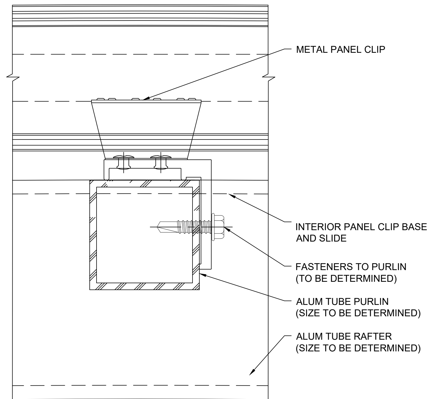
O 2 SECTION @ PURLINS 2.75" QuadSpan™ SYSTEM (4" QuadSpan™ SYSTEM SIMILAR) NOTE: THIS DETAIL OCCURS WHEN GLAZING IS SHIPPED IN PANELIZED SECTIONS.
