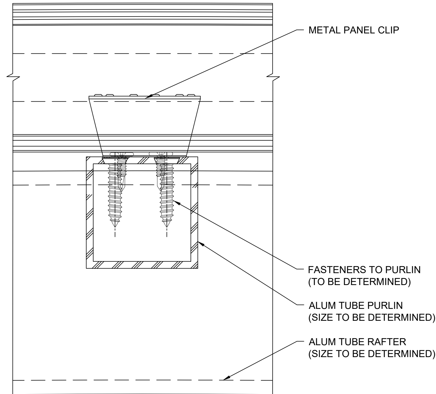
O SECTION @ PURLINS 2.75" QuadSpan™ SYSTEM (4" QuadSpan™ SYSTEM SIMILAR) NOTE: THIS DETAIL OCCURS WHEN GLAZING IS SHIPPED KNOCKED DOWN.
