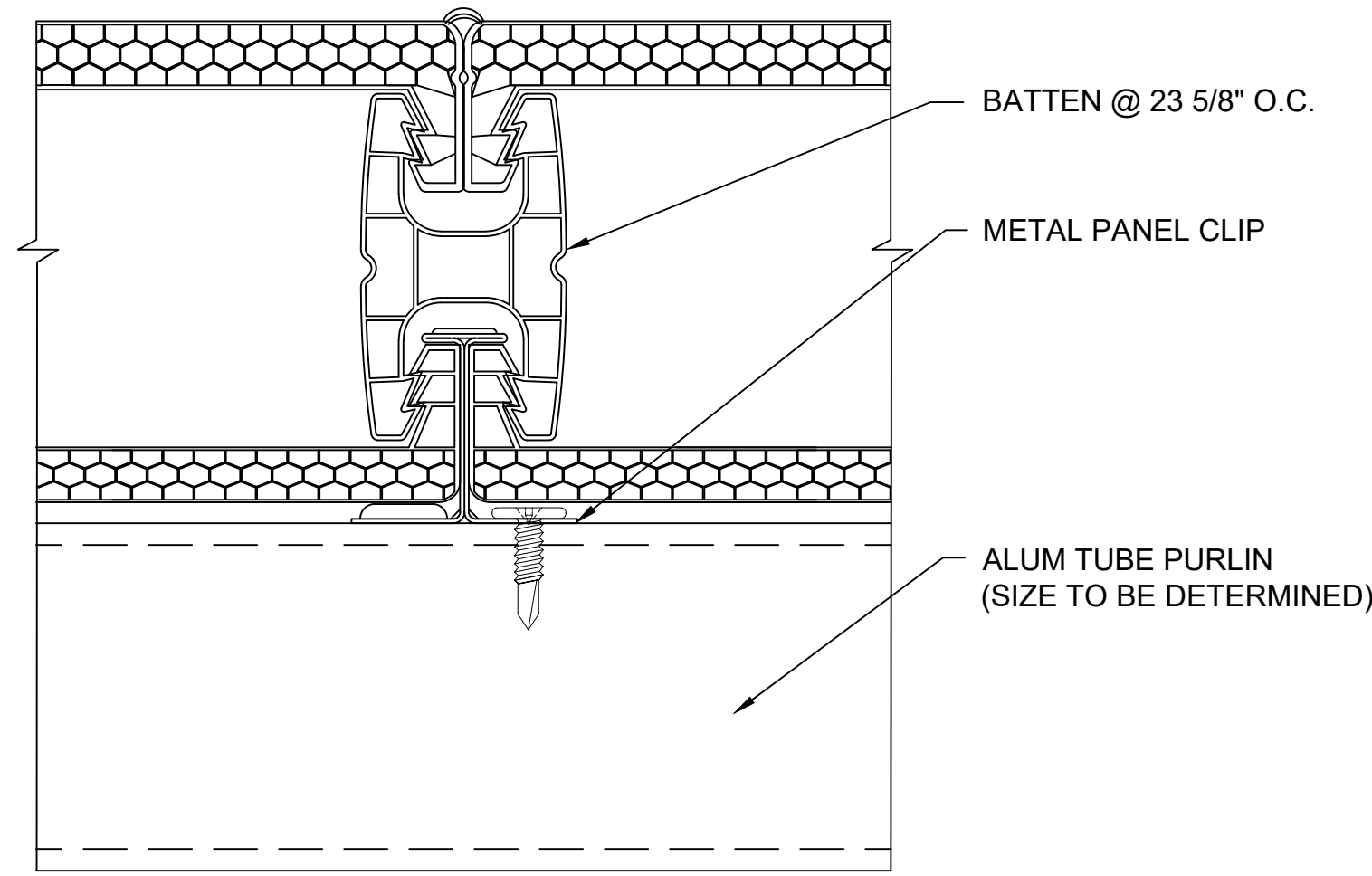
L SECTION @ BATTEN 2.75" QuadSpan™ SYSTEM
