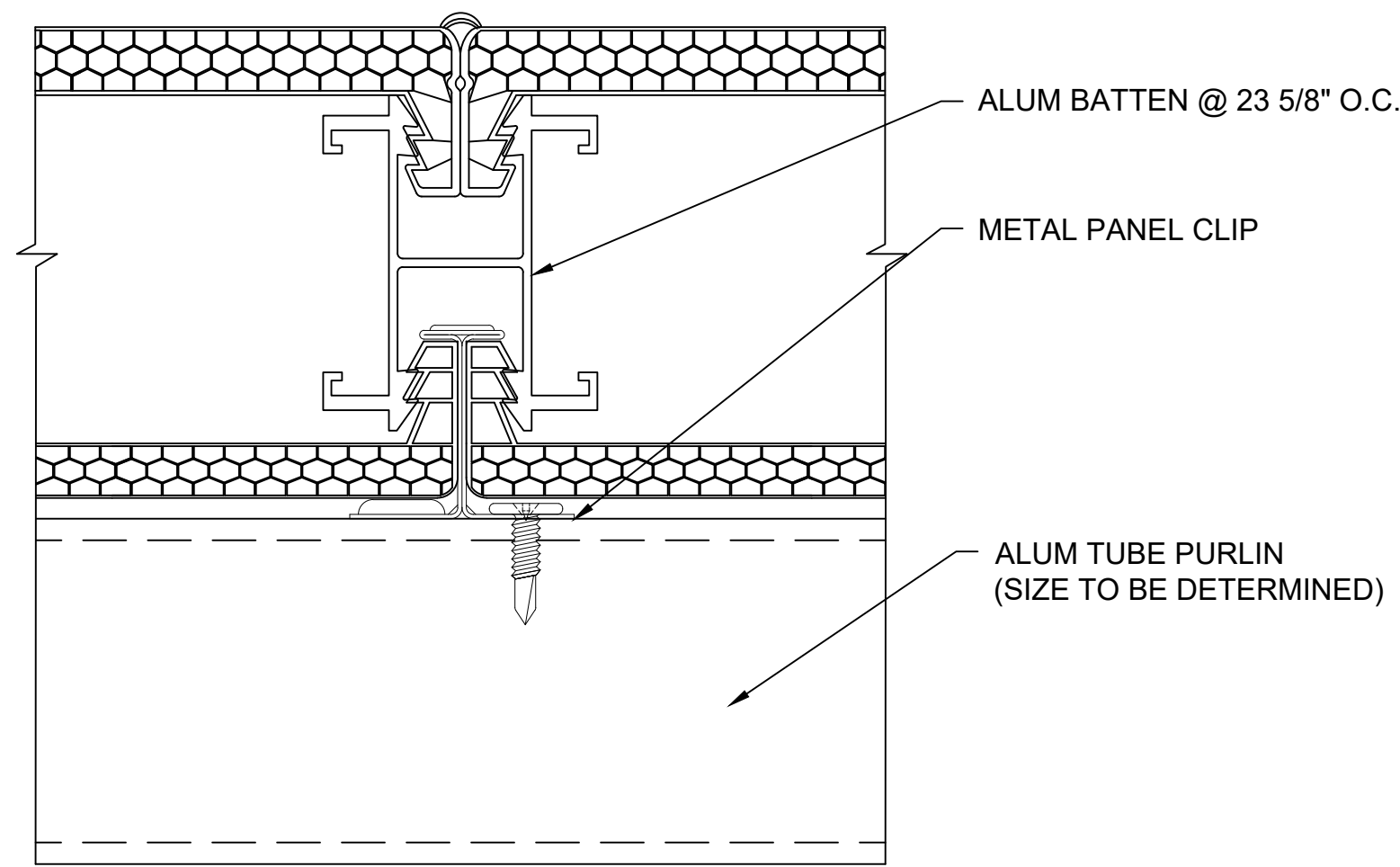
L 2 SECTION @ BATTEN 2.75" QuadSpan™ SYSTEM
