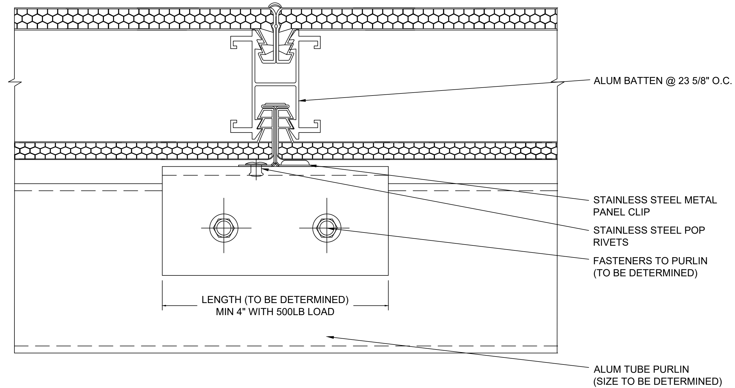
NOTE: THESE DETAILS OCCUR WHEN GLAZING IS SHIPPED IN PANELIZED SECTIONS. K 2 SECTION @ BATTEN 2.75" QuadSpan™ SYSTEM (4" QuadSpan™ SYSTEM SIMILAR)
