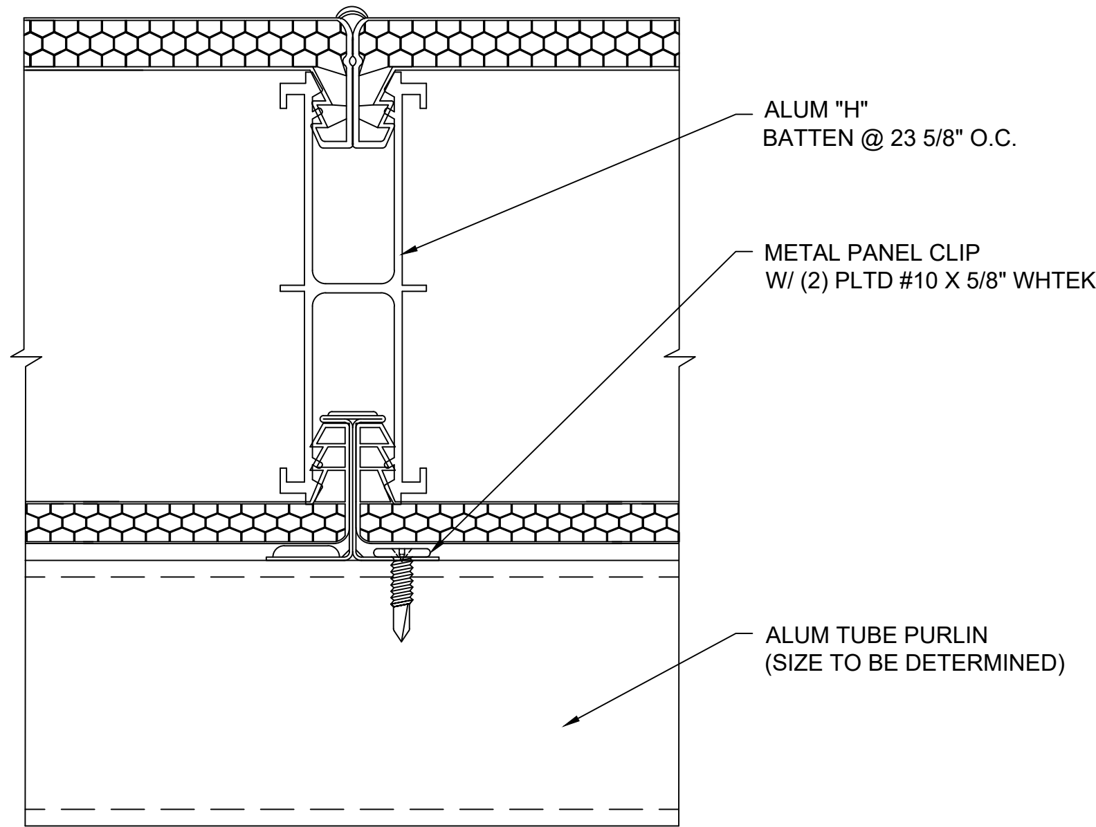
L 3 SECTION @ BATTEN 4" QuadSpan™ SYSTEM NOTE: THESE DETAILS OCCUR WHEN GLAZING IS SHIPPED KNOCKED DOWN.
