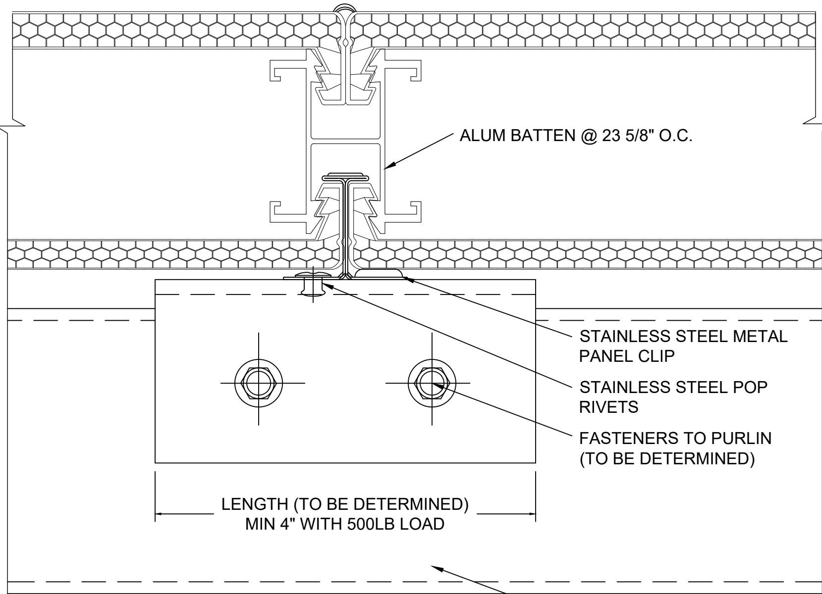
K 2 SECTION @ BATTEN 2.75" QuadSpan™ SYSTEM (4" QuadSpan™ SYSTEM SIMILAR) NOTE: DETAILS K-K2 OCCUR WHEN GLAZING IS SHIPPED IN PANELIZED SECTIONS.
