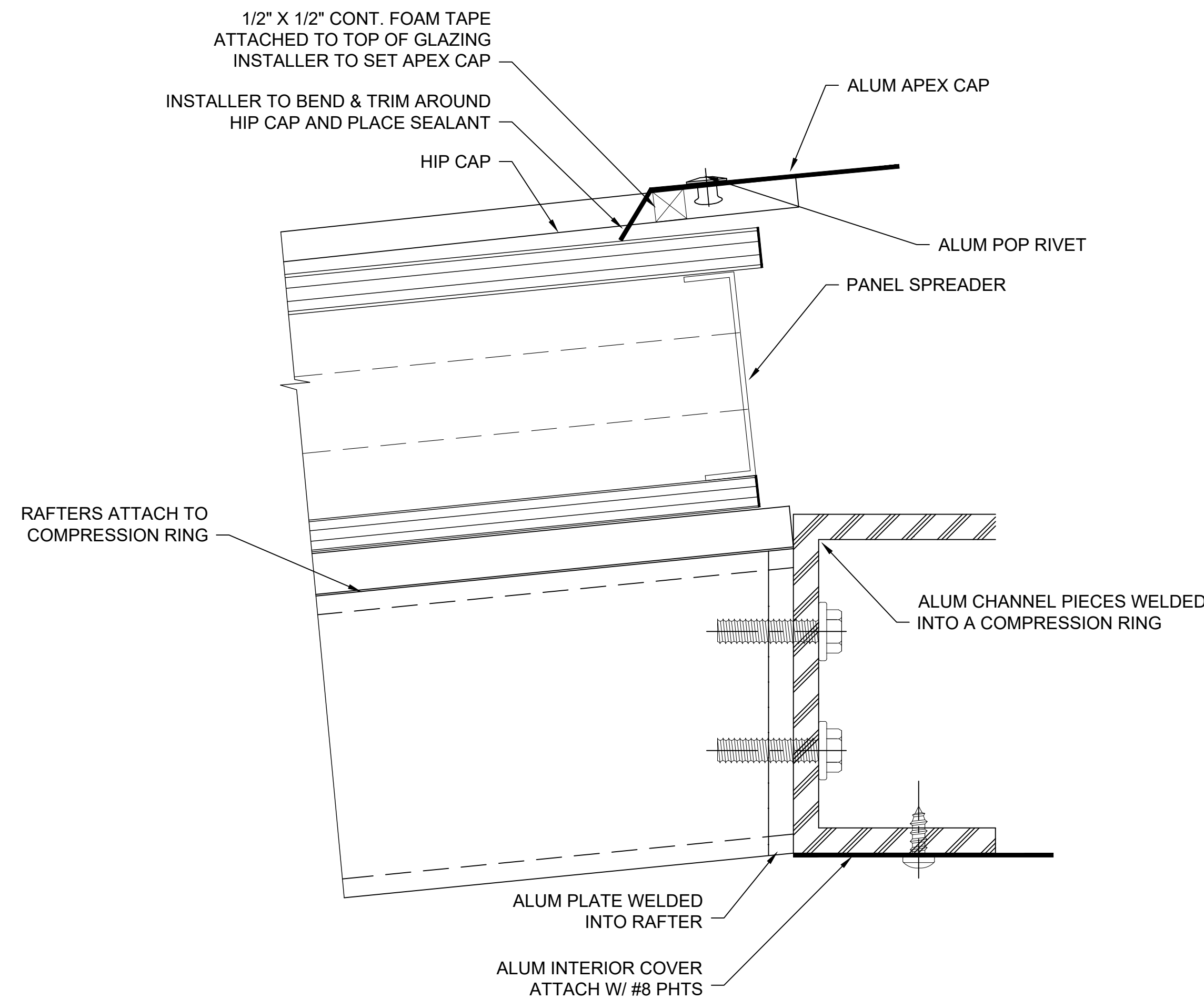
V SECTION @ APEX 2.75" QuadSpan™ SYSTEM
