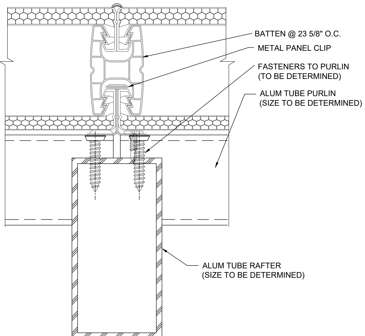
N SECTION @ RAFTER 2.75" QuadSpan™ SYSTEM (4" QuadSpan™ SYSTEM SIMILAR)
