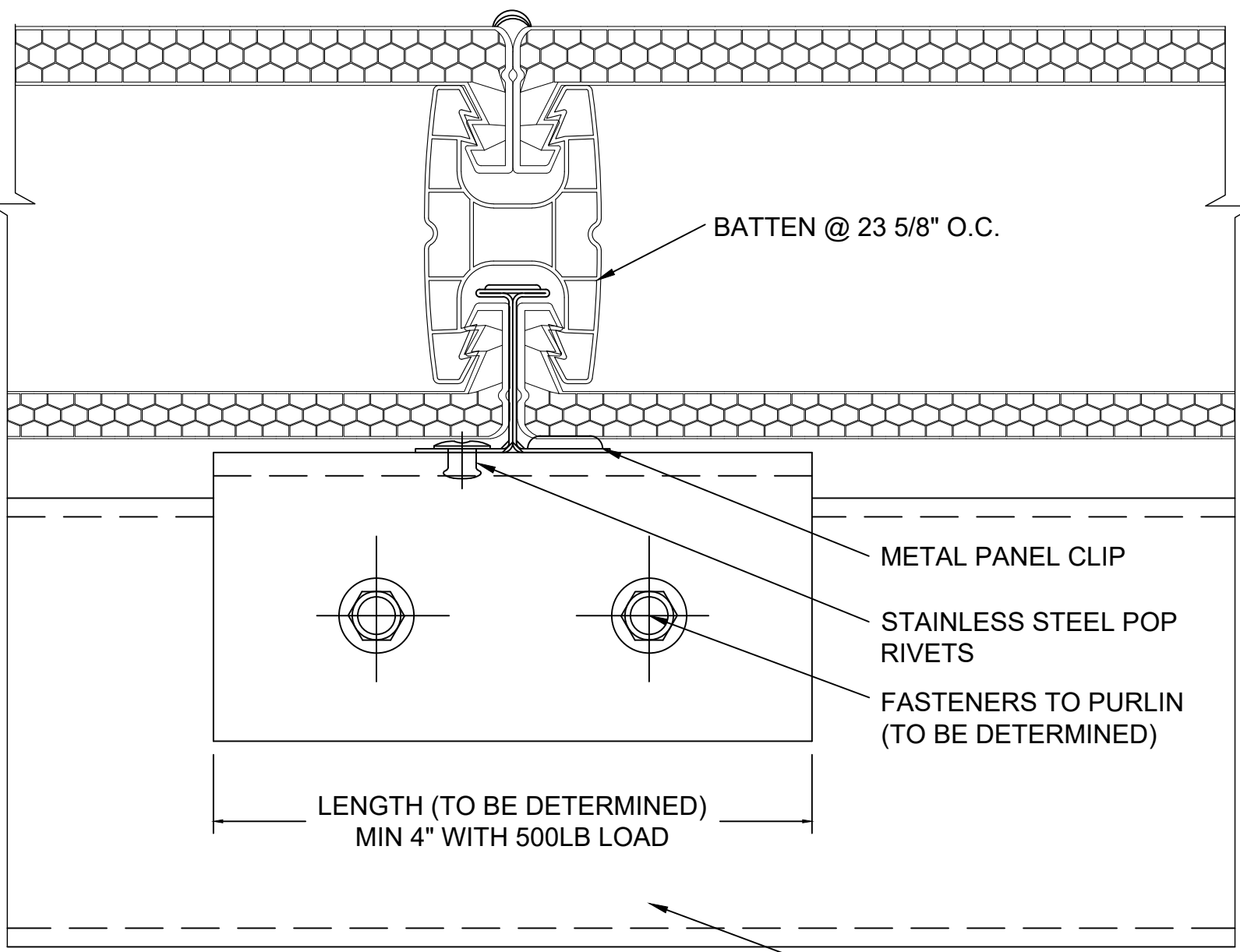
K SECTION @ BATTEN 2.75" QuadSpan™ SYSTEM (4" QuadSpan™ SYSTEM SIMILAR)
