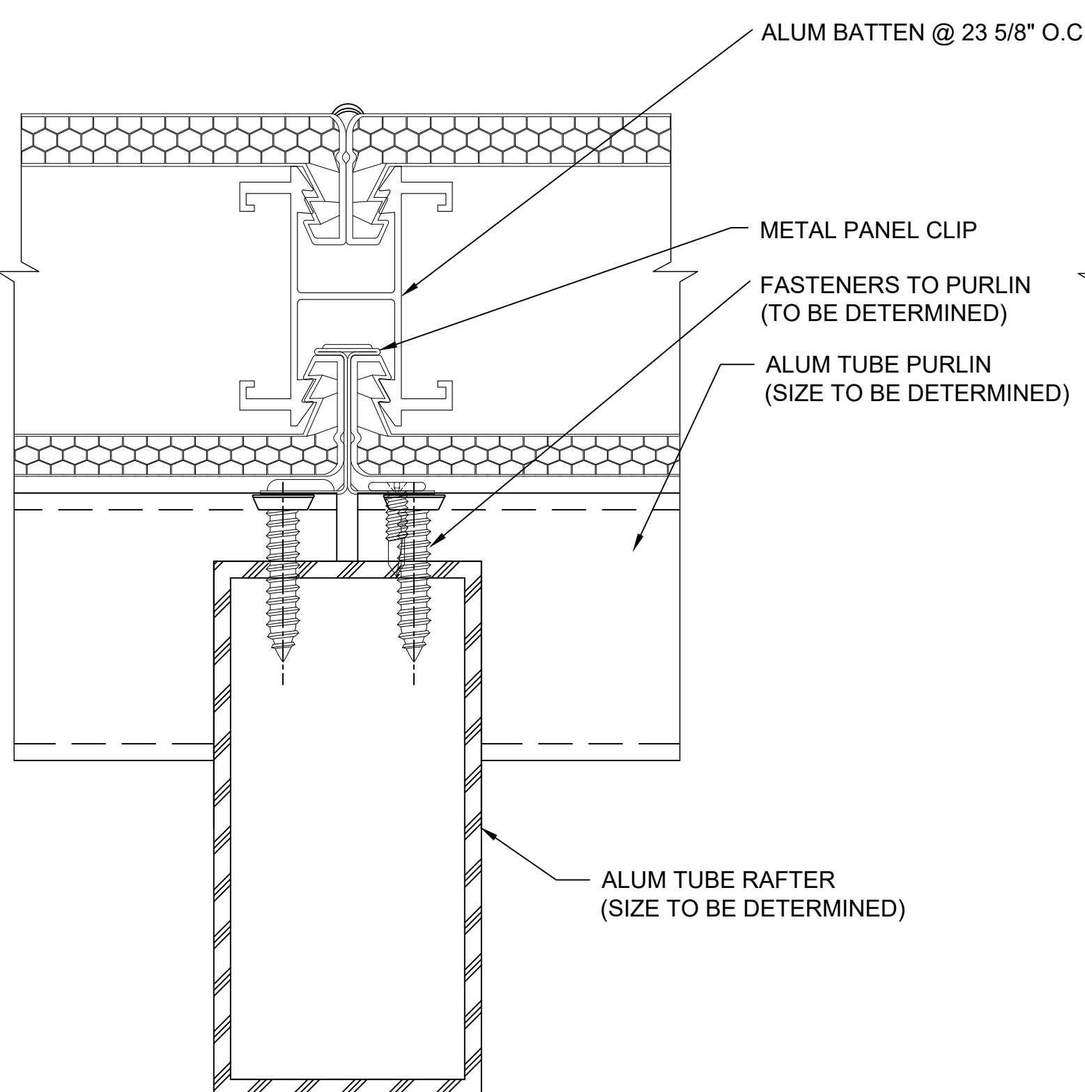
N 2 SECTION @ RAFTER 2.75" QuadSpan™ SYSTEM (4" QuadSpan™ SYSTEM SIMILAR) NOTE: DETAILS N-N2 OCCUR WHEN GLAZING IS SHIPPED KNOCKED DOWN.
