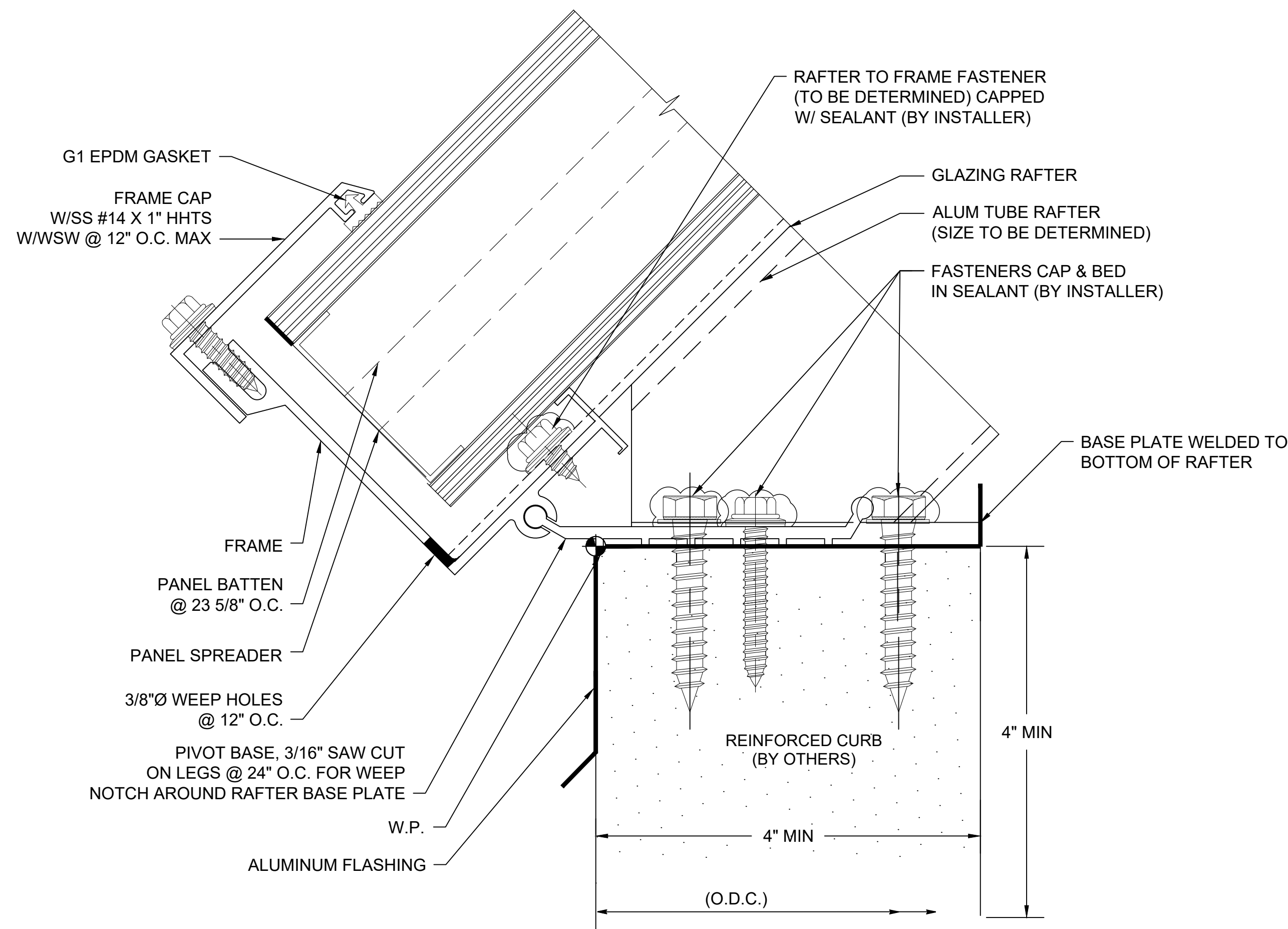
A SECTION @ SILL (FLAT CURB) 2.75" QuadSpan™ SYSTEM (4" QuadSpan™ SYSTEM SIMILAR)
