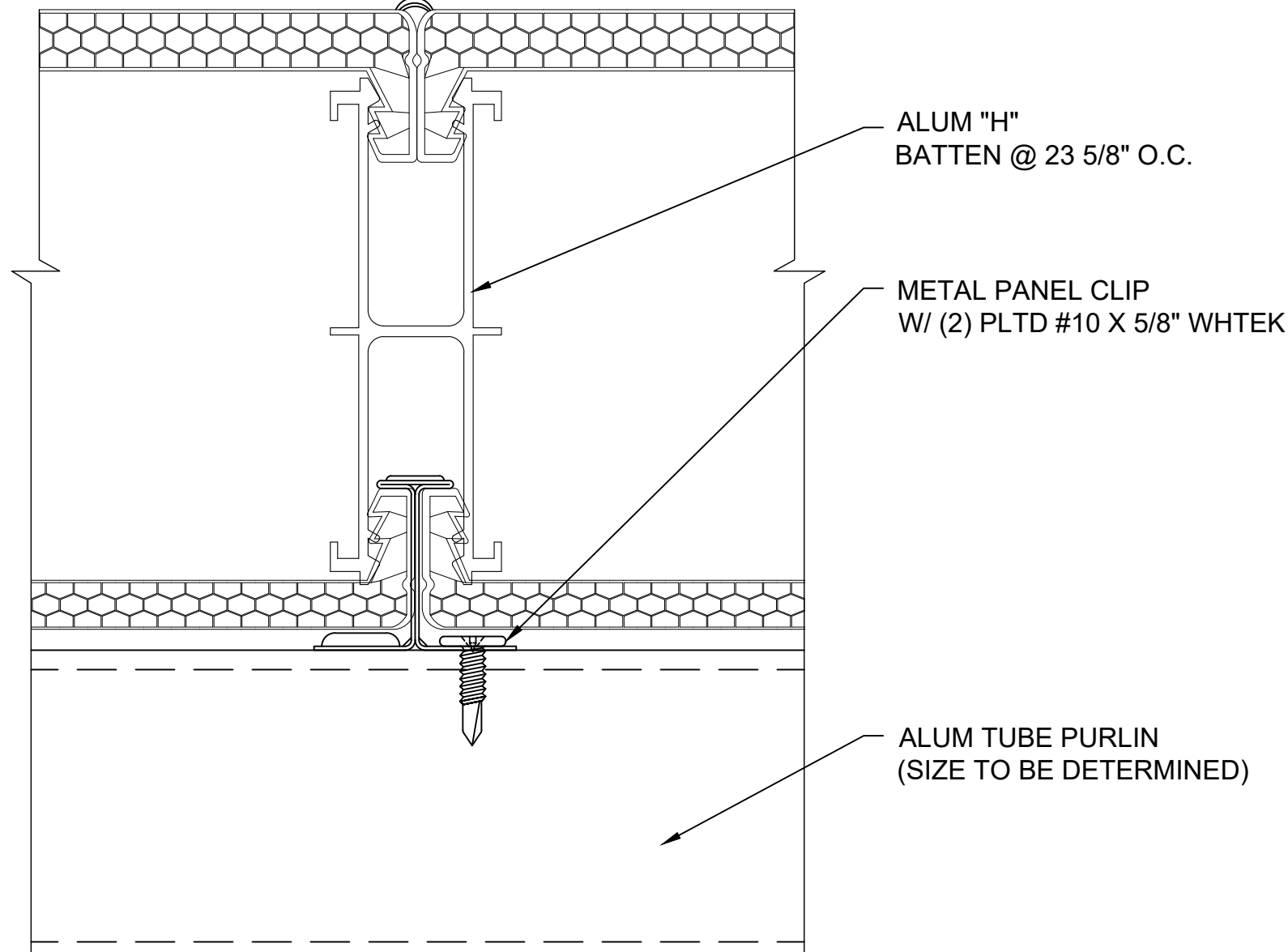
L 3 SECTION @ BATTEN 4" QuadSpan™ SYSTEM NOTE: DETAILS L-L3 OCCUR WHEN GLAZING IS SHIPPED KNOCKED DOWN.
