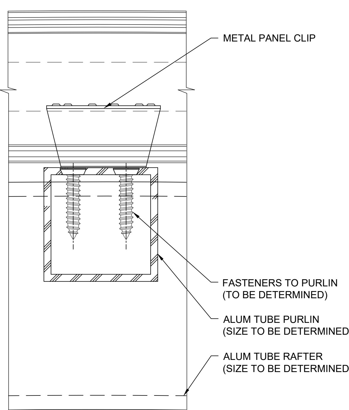
O SECTION @ PURLINS 2.75" QuadSpan™ SYSTEM (4" QuadSpan™ SYSTEM SIMILAR) NOTE: THIS DETAIL OCCURS WHEN GLAZING IS SHIPPED KNOCKED DOWN.
