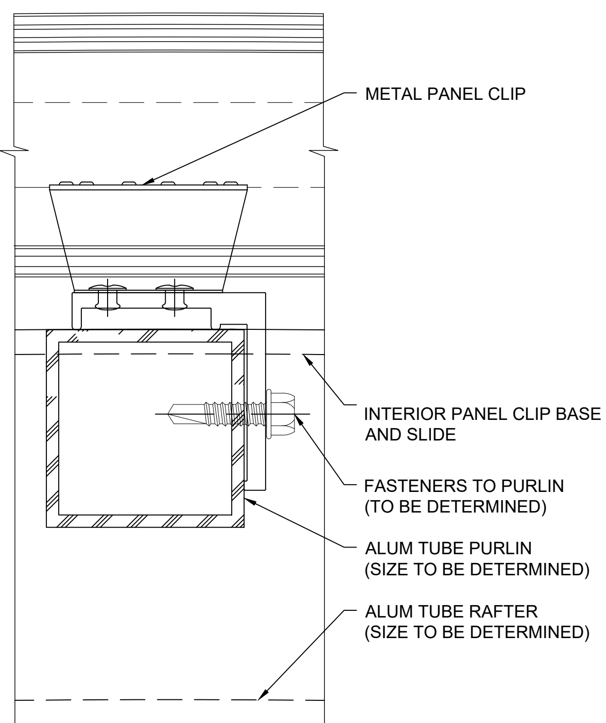
O 2 SECTION @ PURLINS 2.75" QuadSpan™ SYSTEM (4" QuadSpan™ SYSTEM SIMILAR) NOTE: THIS DETAIL OCCURS WHEN GLAZING IS SHIPPED IN PANELIZED SECTIONS.
