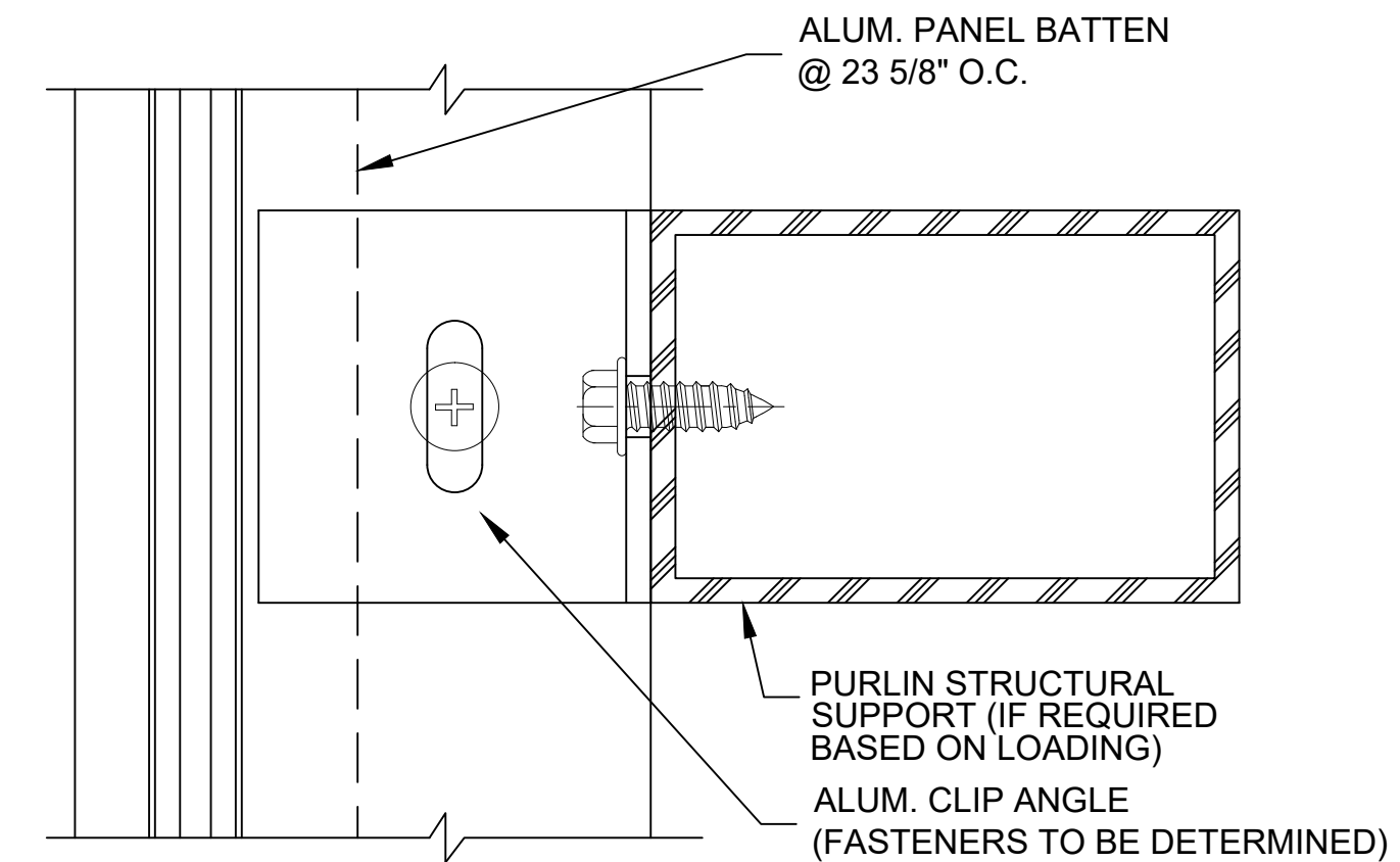
B 2 SECTION @ HEAD - ALUM BATTEN SINGLE PANEL - FLUSH
