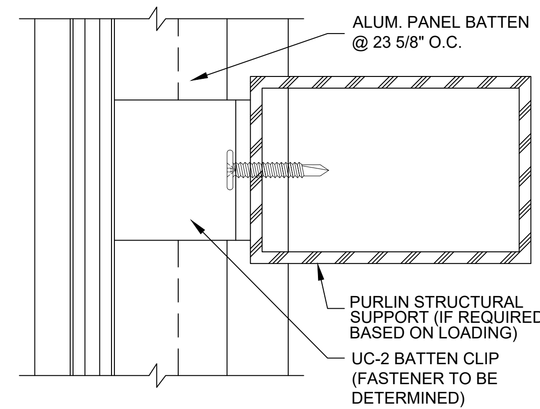
E 1 SECTION @ PURLIN - POLY BATTEN SINGLE PANEL - FLUSH
