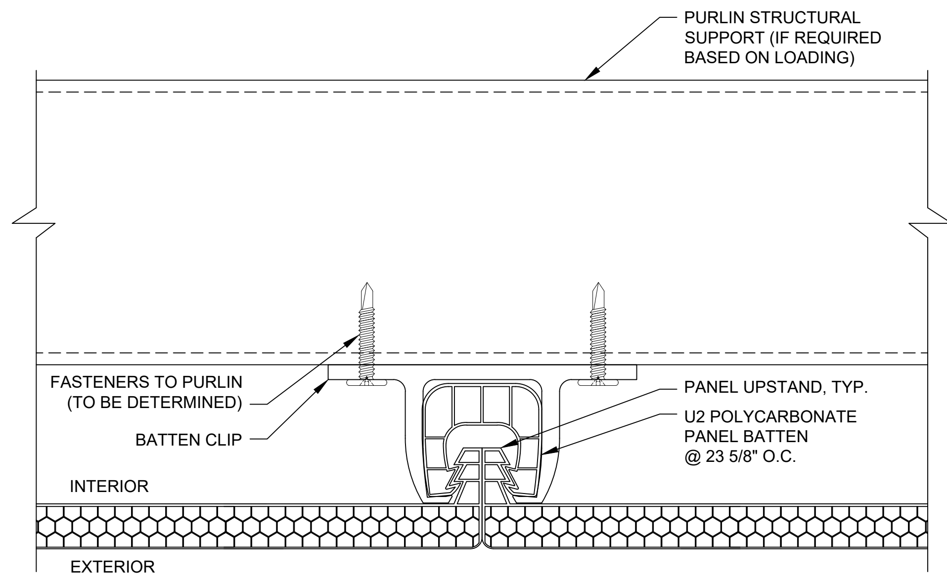
D1 SECTION @ BATTEN SINGLE PANEL - FLUSH
