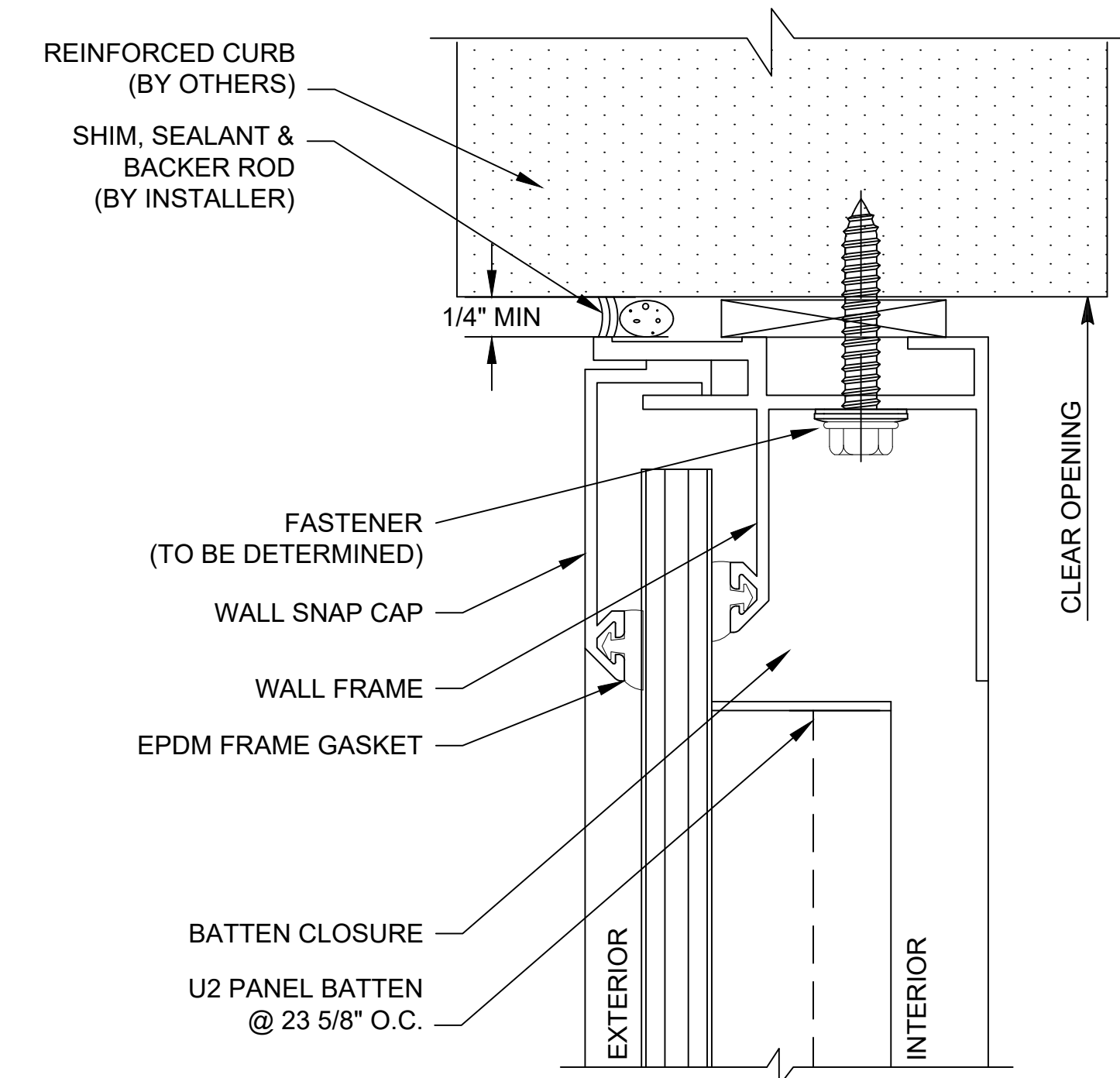
B 1 SECTION @ HEAD - POLY BATTEN SINGLE PANEL - FLUSH
