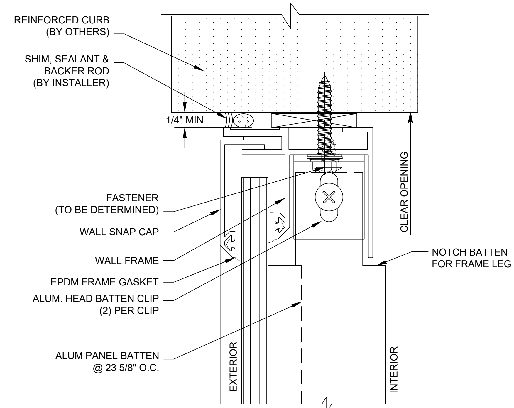
B 2 SECTION @ HEAD - ALUM BATTEN SINGLE PANEL - FLUSH
