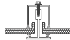
U-Lite™ Rafter
