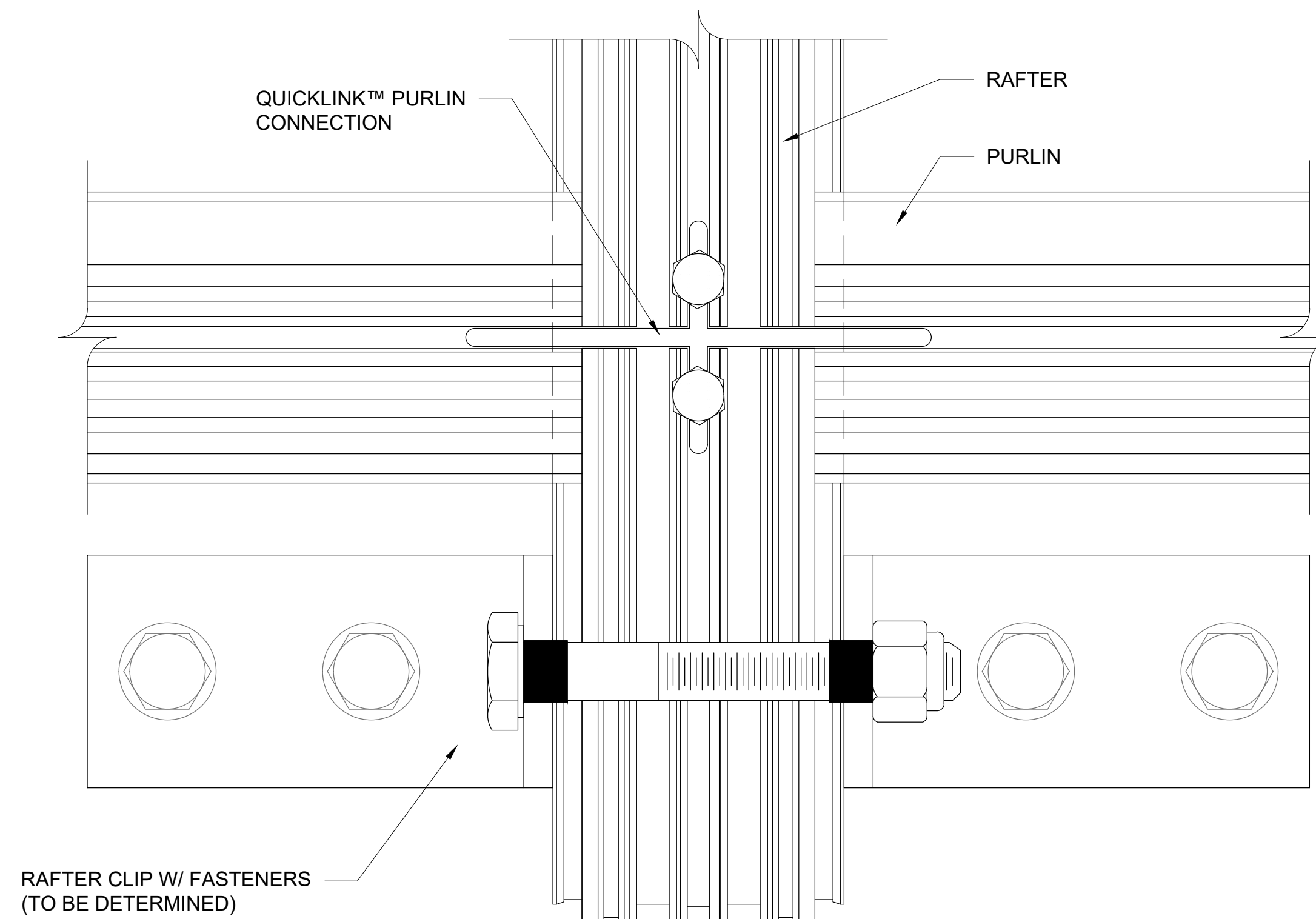
2 5 RAFTER & PURLIN CONNECTION - - SCALE: 6" = 1'-0"
