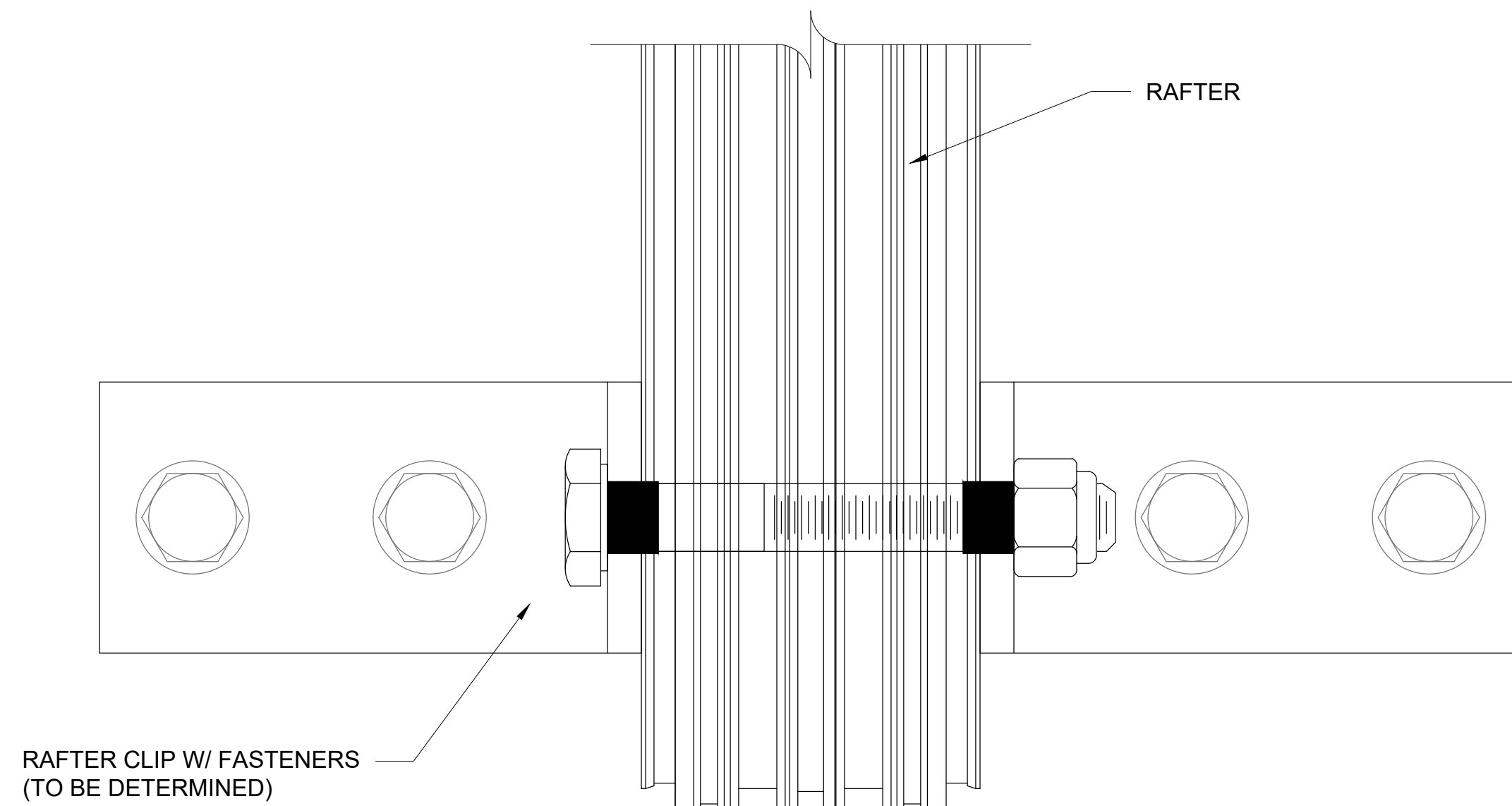
3 2 - - RAFTER & PURLIN CONNECTION SCALE: 6" = 1'-0"
