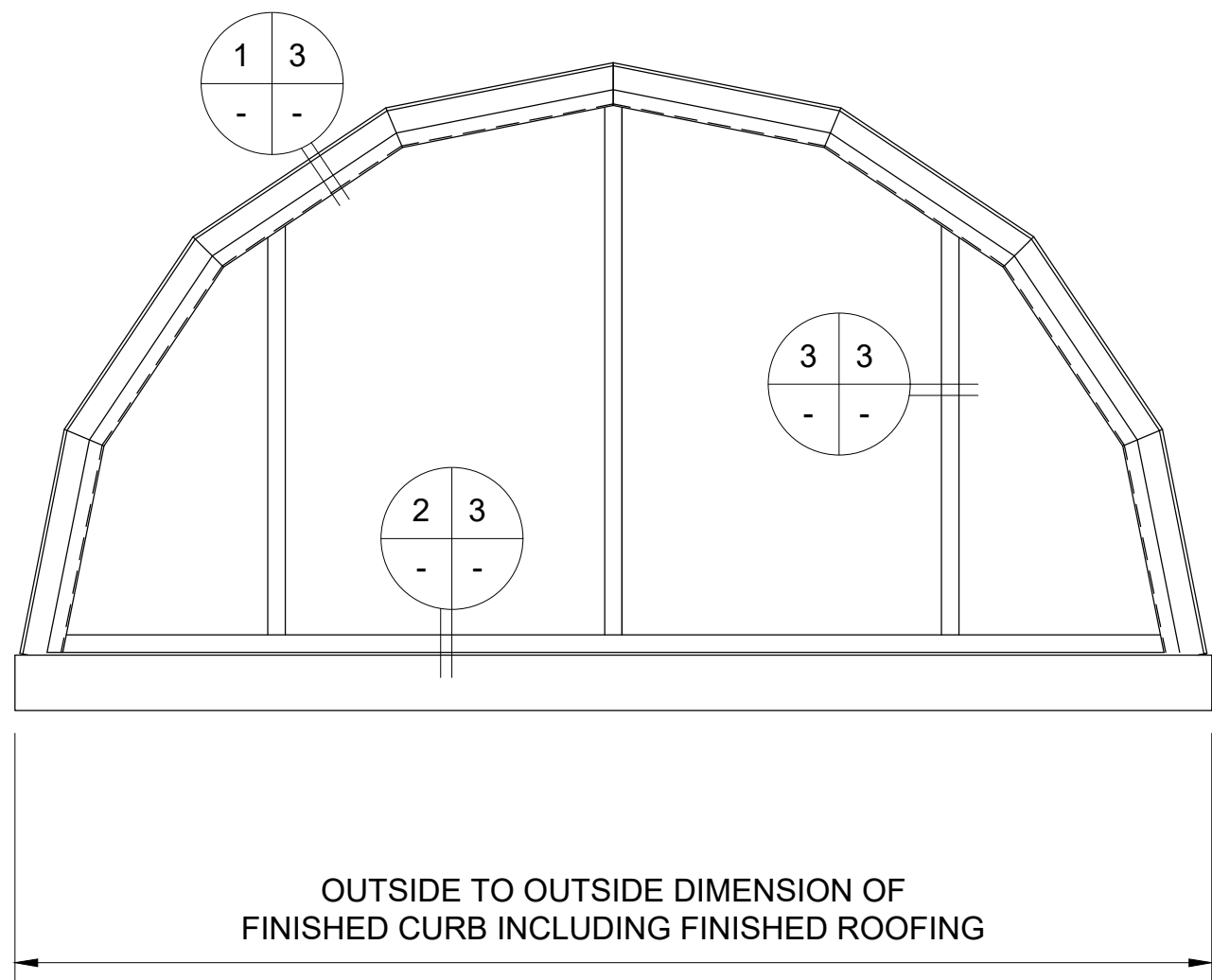
GABLE ELEVATION
