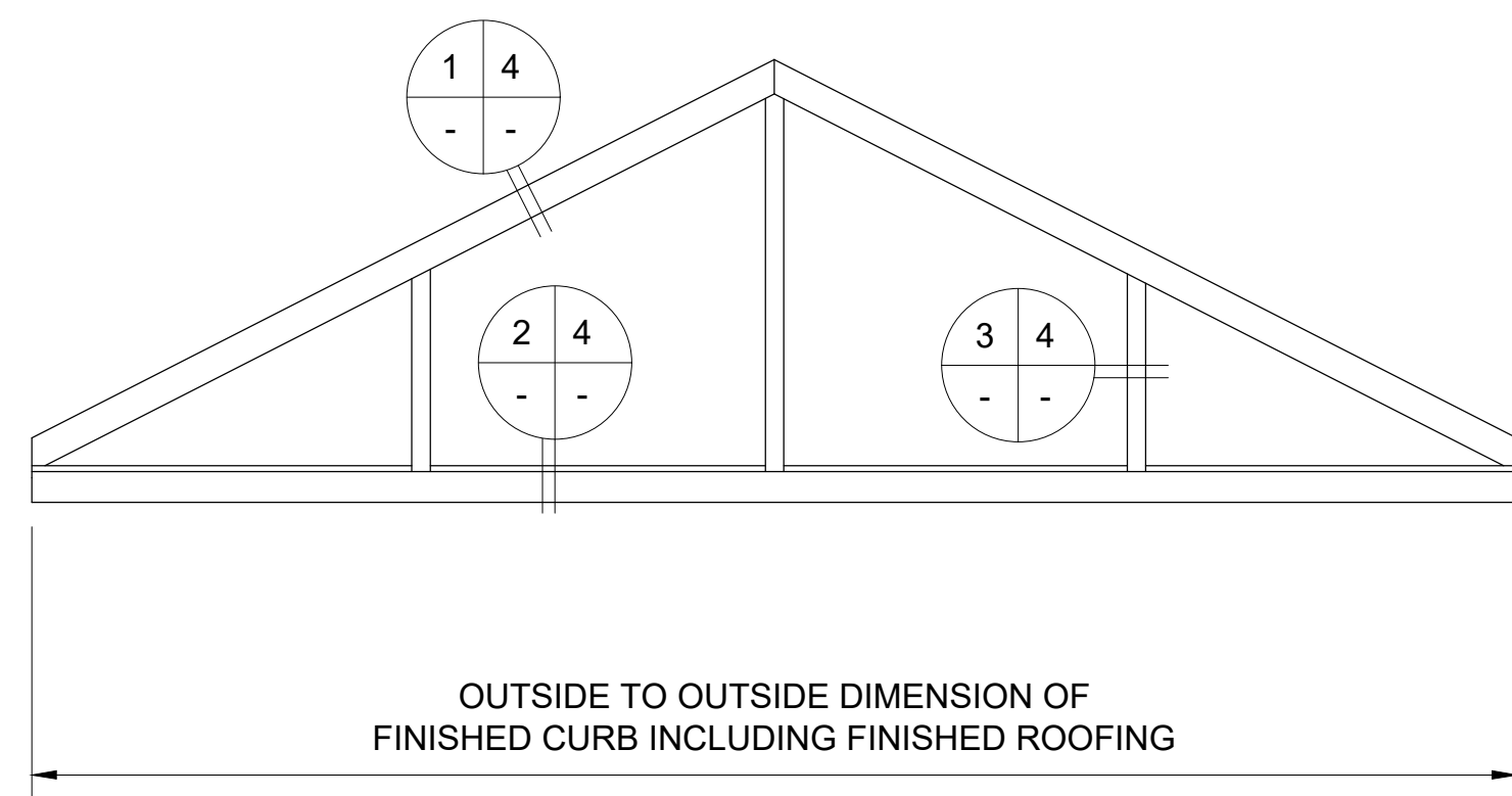
GABLE ELEVATION
