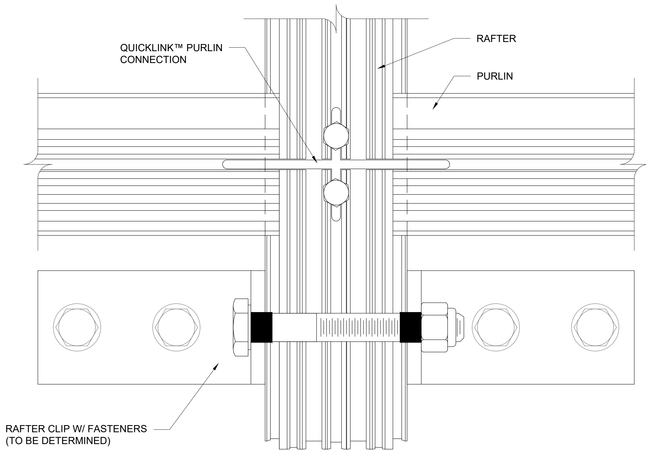
4 2 - - RAFTER & PURLIN CONNECTION SCALE: 6" = 1'-0"
