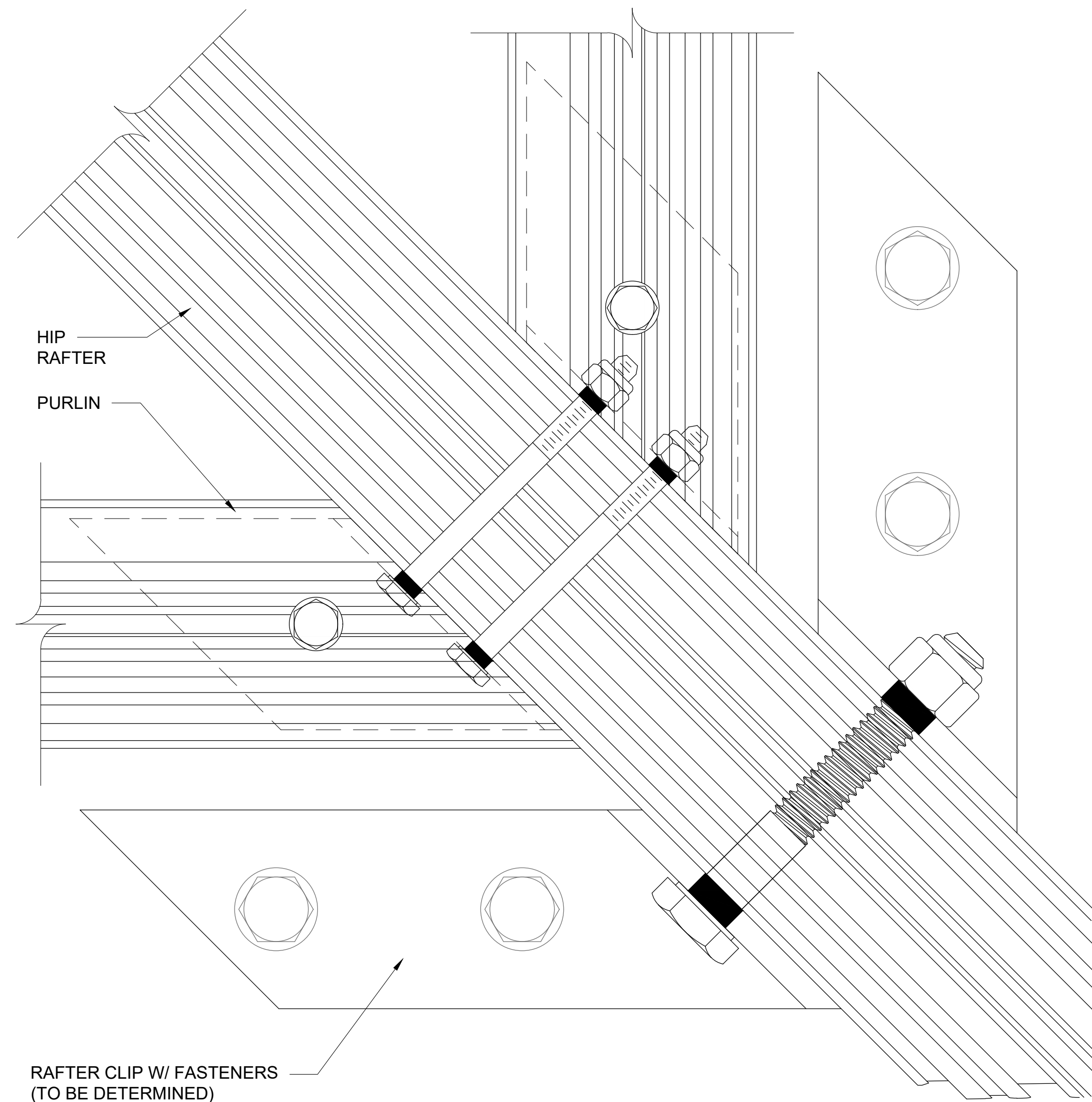
5 2 - - HIP TO CURB CONNECTION SCALE: 6" = 1'-0"
