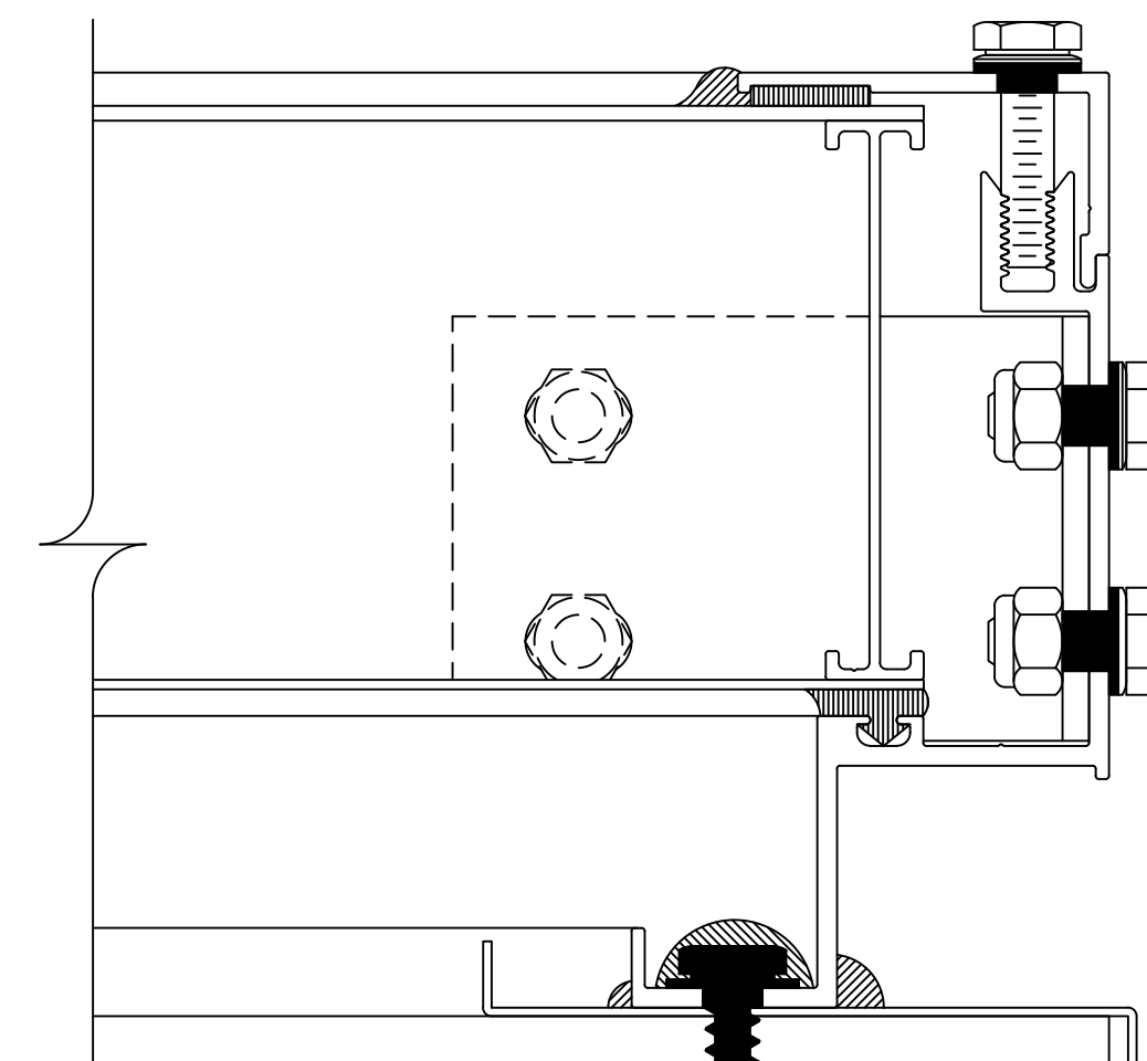
2 2 JAMB DETAIL - - SCALE: FULL
