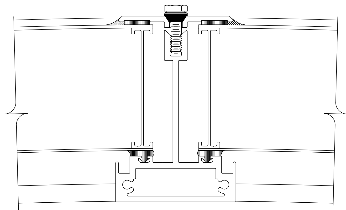
3 2 PURLIN DETAIL - - SCALE: FULL
