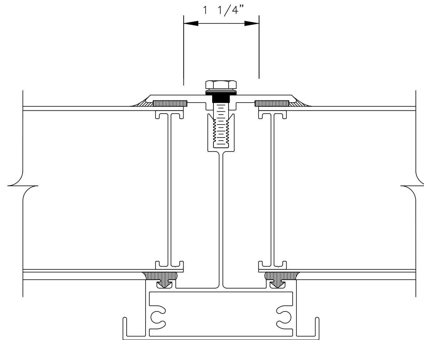
1 2 RAFTER DETAIL - - SCALE: FULL
