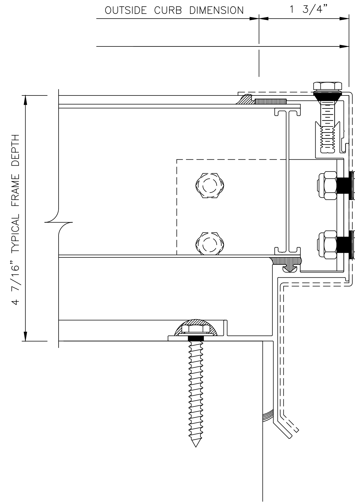
2 2 JAMB DETAIL - - SCALE: FULL
