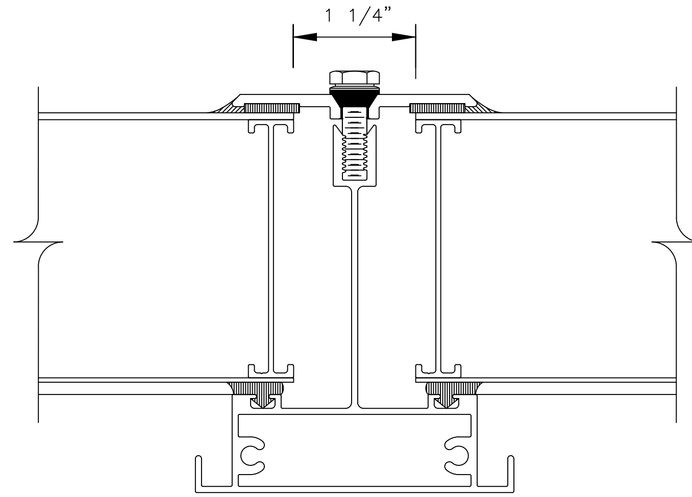
1 2 RAFTER DETAIL - - SCALE: FULL
