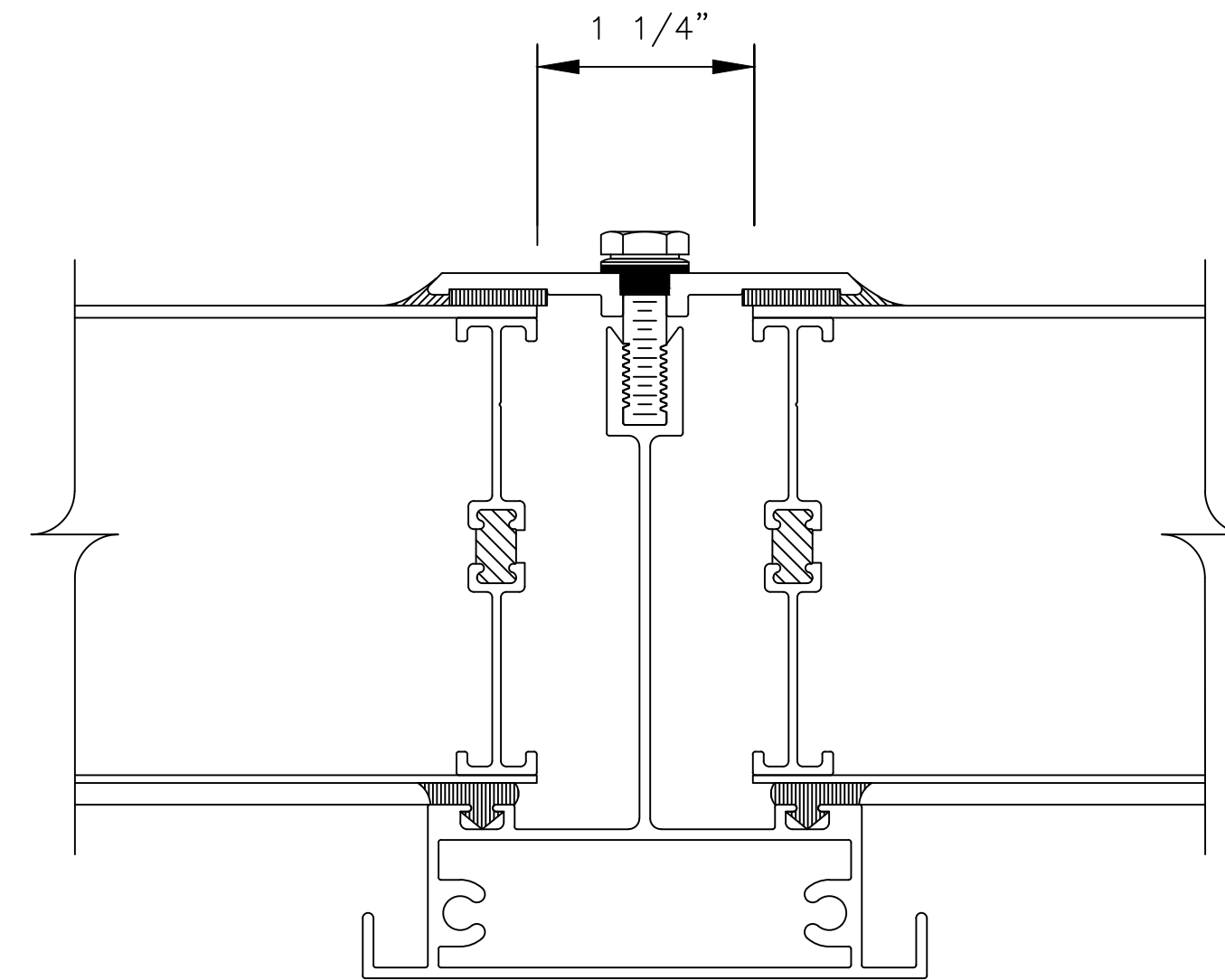
1 2 RAFTER DETAIL — — SCALE: FULL
