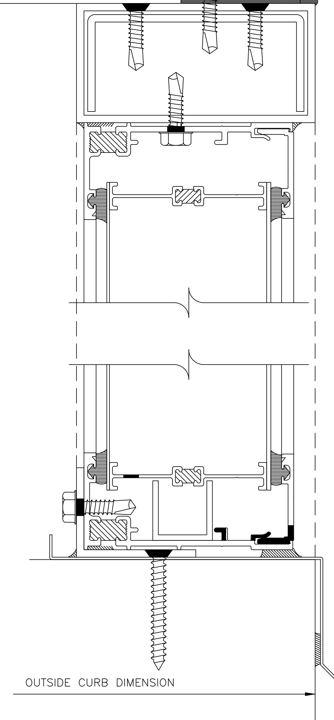
5 2 SILL DETAIL — — SCALE: FULL
