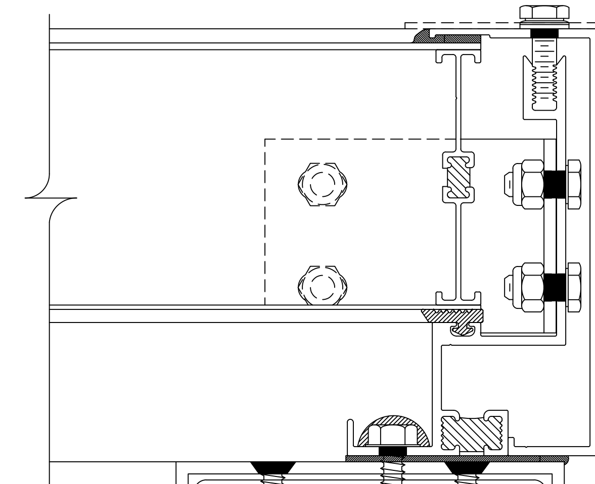
2 2 JAMB DETAIL — — SCALE: FULL
