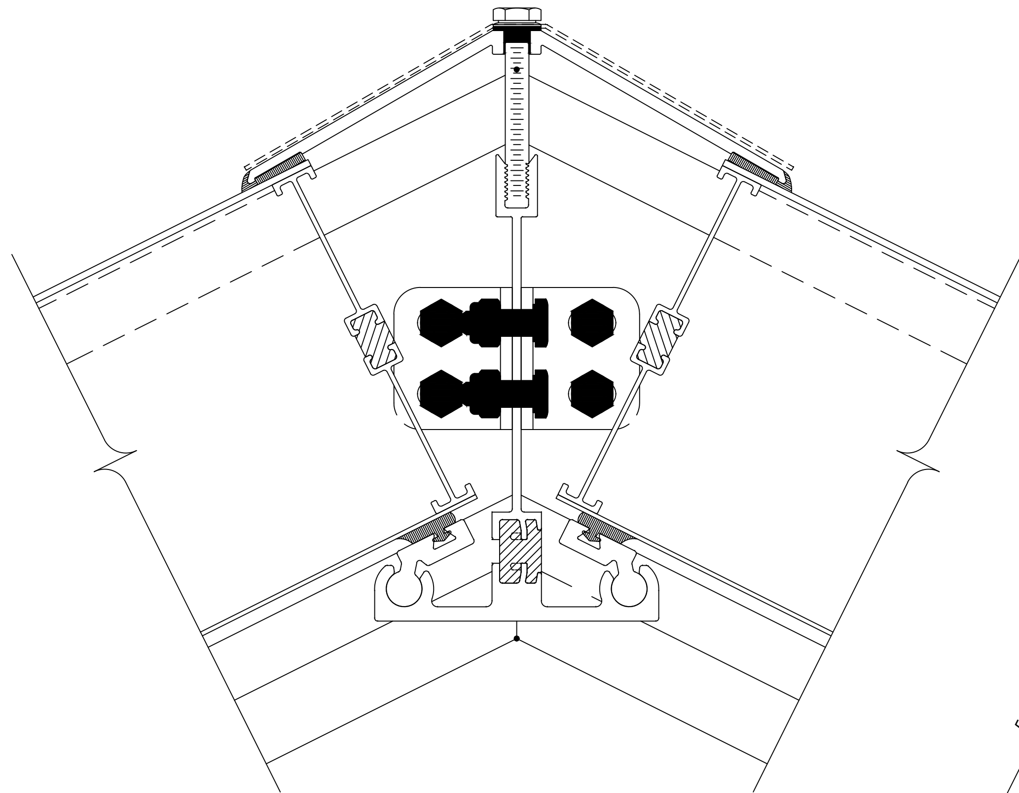
3 2 - - RIDGE DETAIL SCALE: FULL
