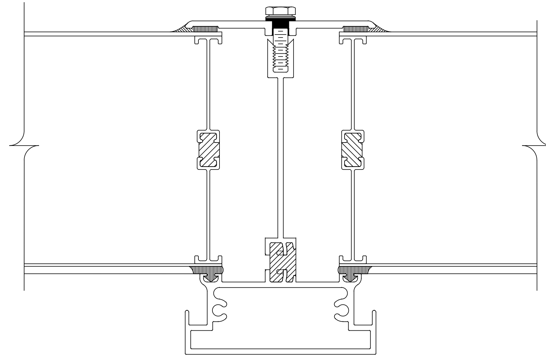
1 2 - - RAFTER DETAIL SCALE: FULL
