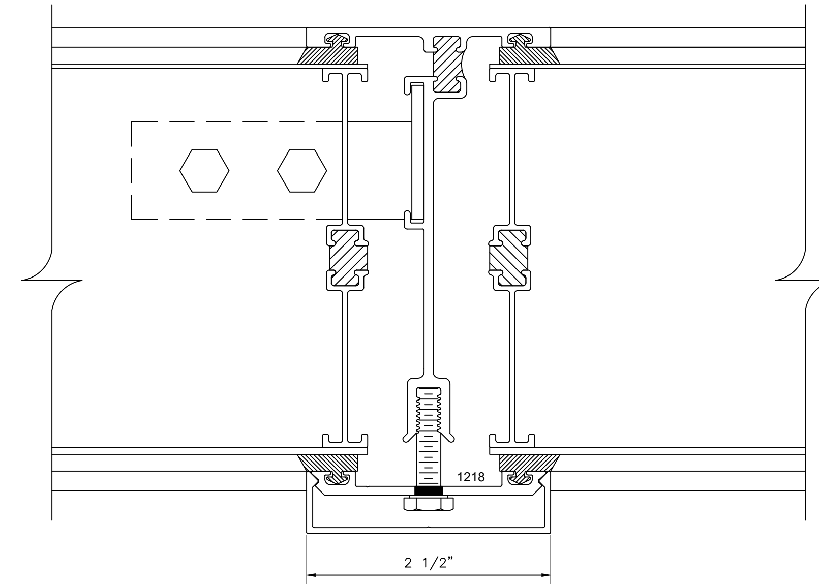
4 3 MULLION DETAIL — — SCALE: FULL
