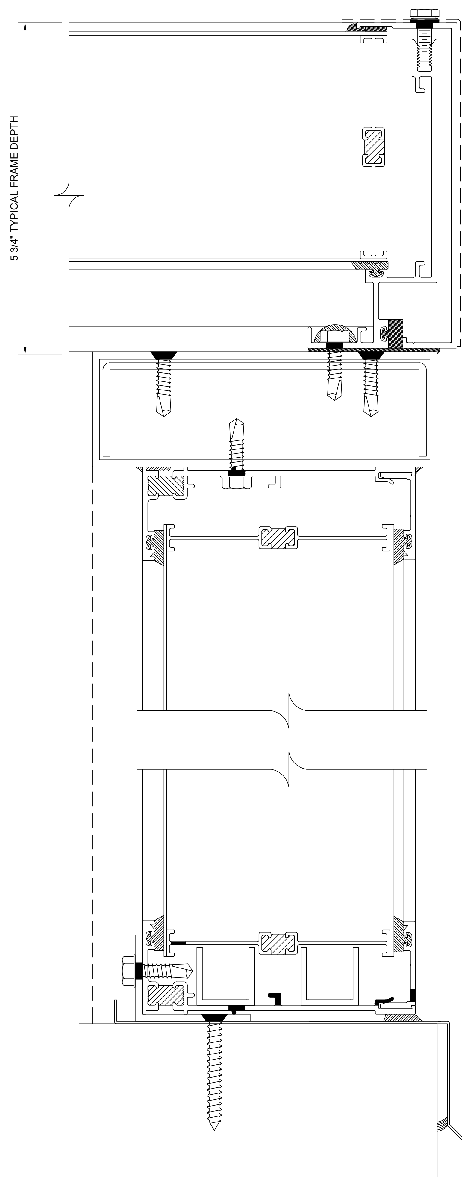
3 3 SILL DETAIL — — SCALE: FULL
