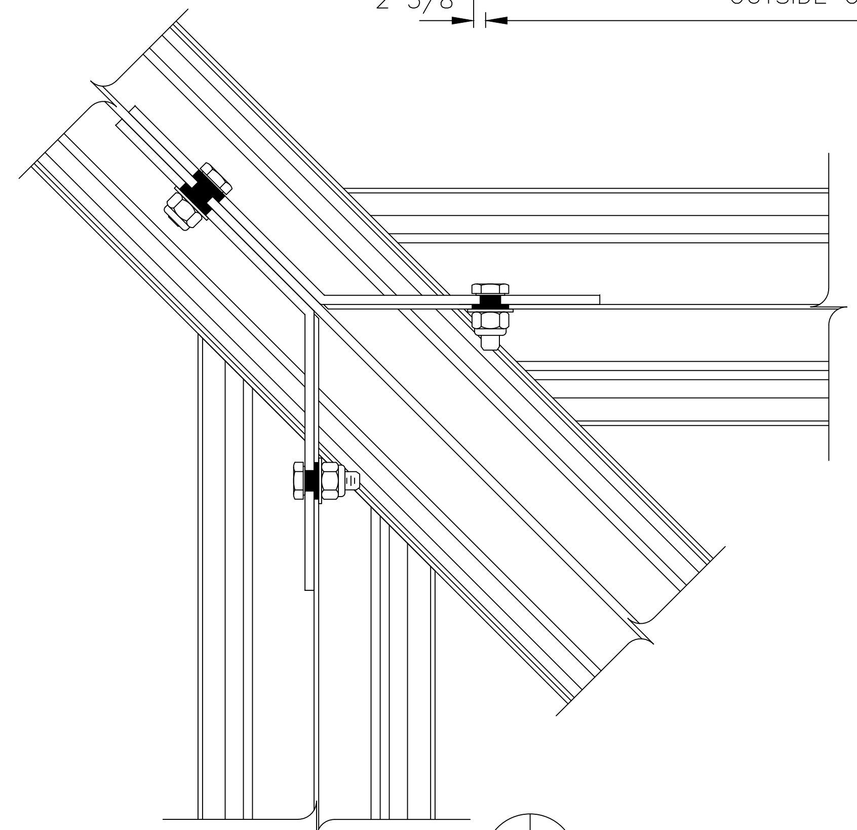
JACK RAFTER CONNECTION SCALE: 3/4" = 1"
