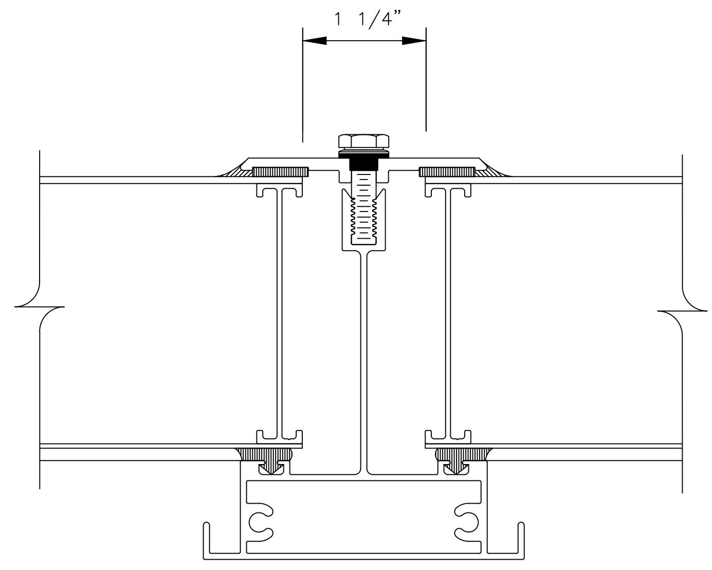
RAFTER DETAIL SCALE: FULL
