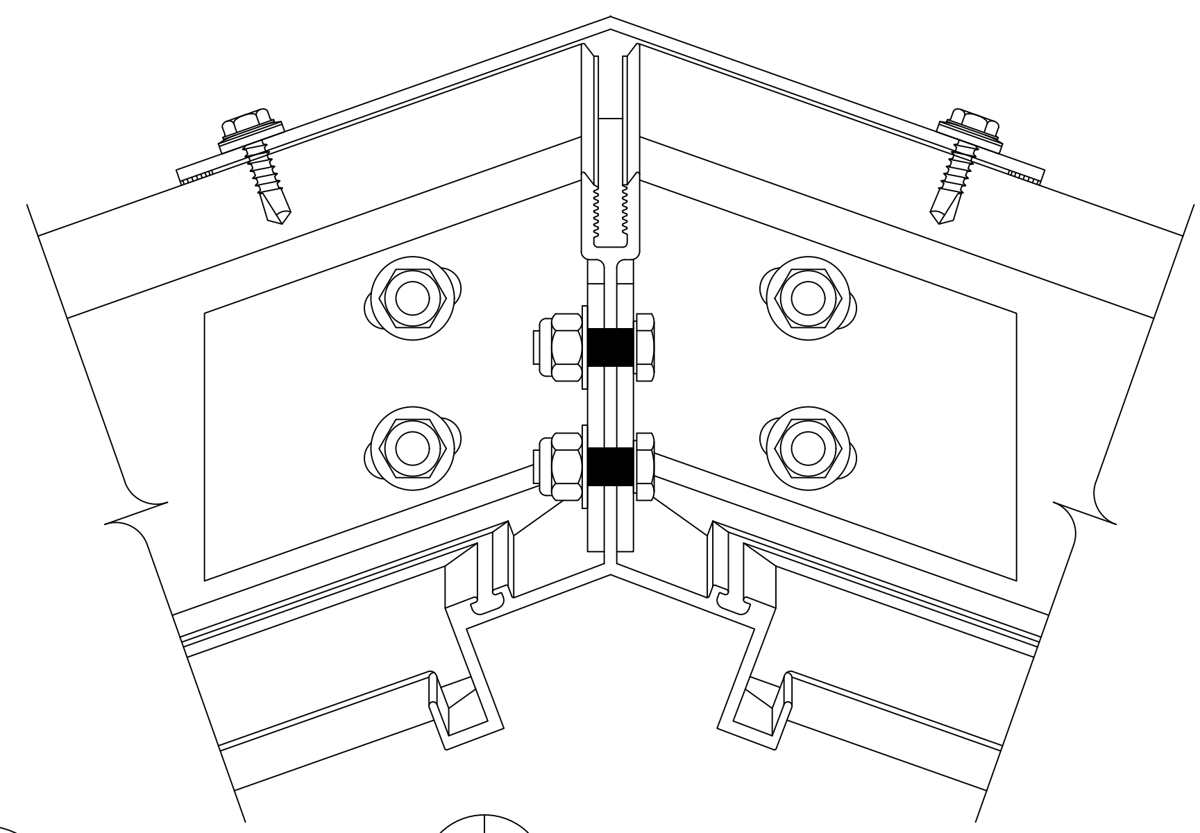
COMPRESSION STAR SCALE: 3/4" = 1"
