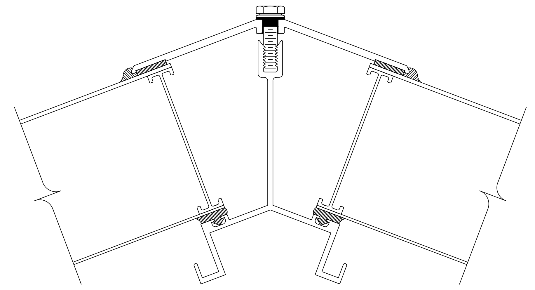
HIP DETAIL SCALE: FULL
