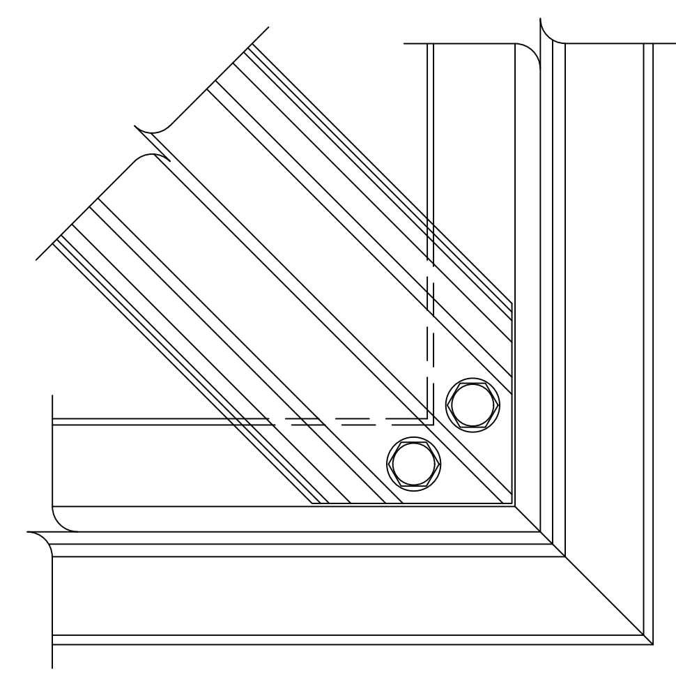
HIP CONNECTION DETAIL SCALE: 3/4" = 1"
