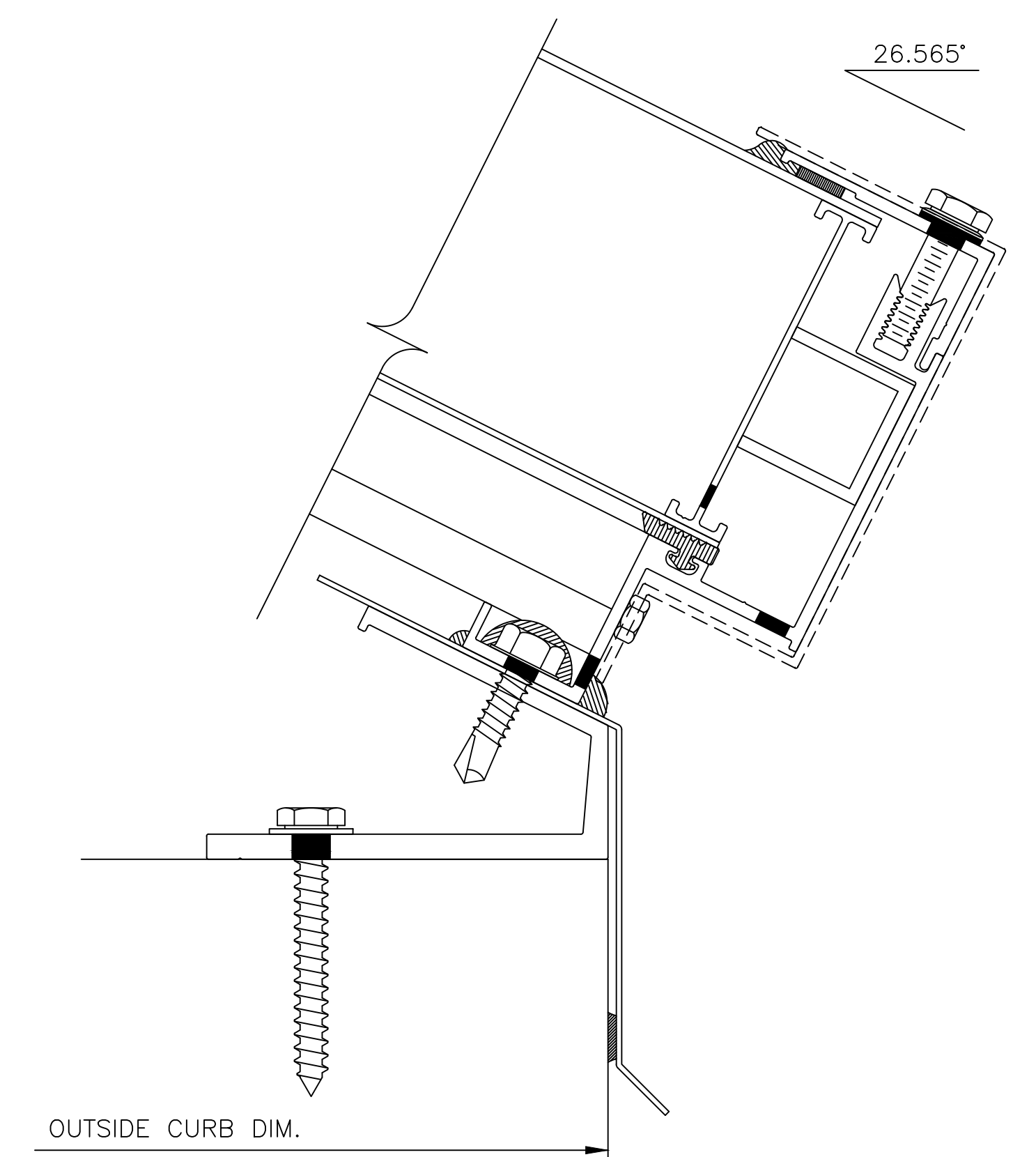
CURB DETAIL SCALE: FULL
