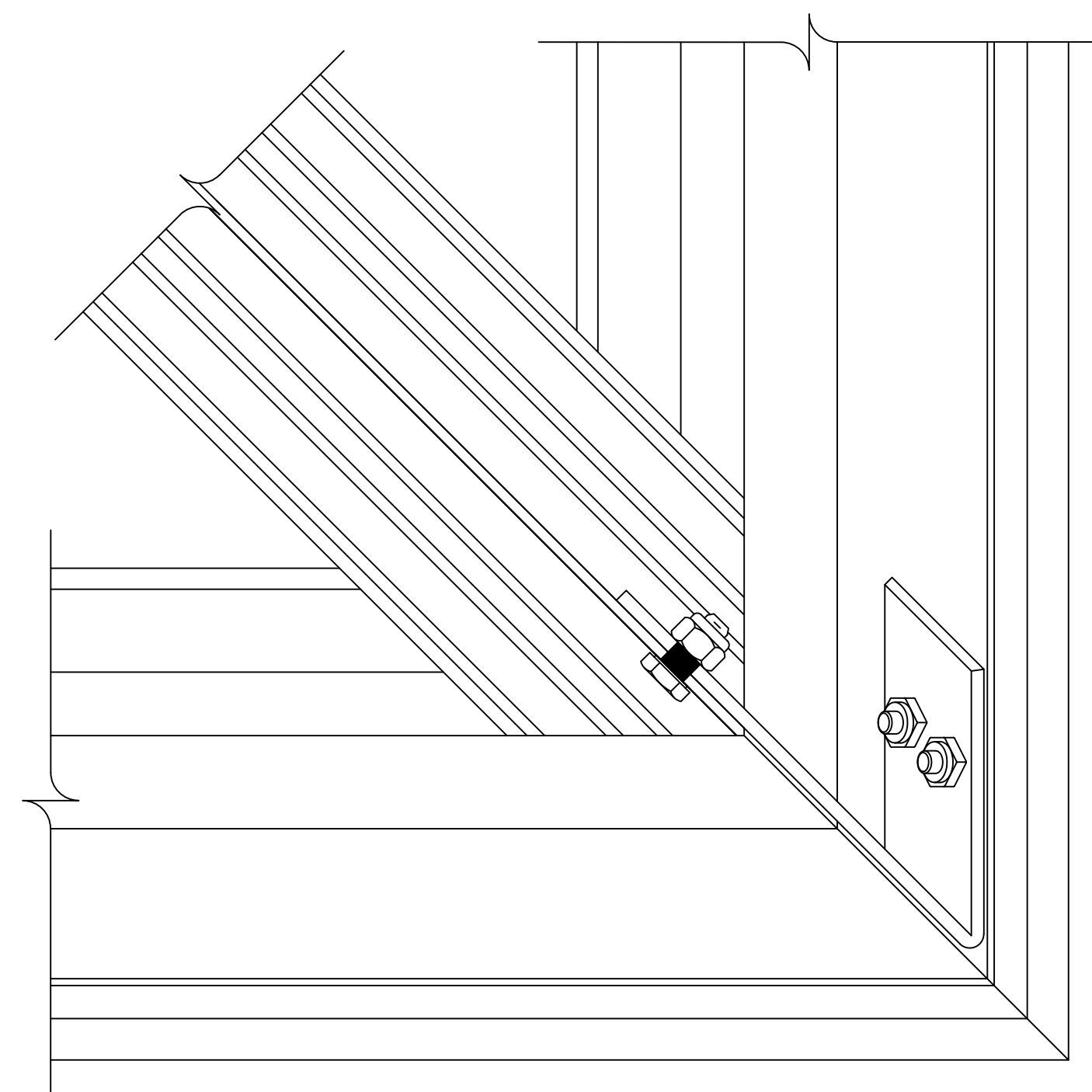
3 3 HIP CONNECTION DETAIL - - SCALE: 3/4" = 1"
