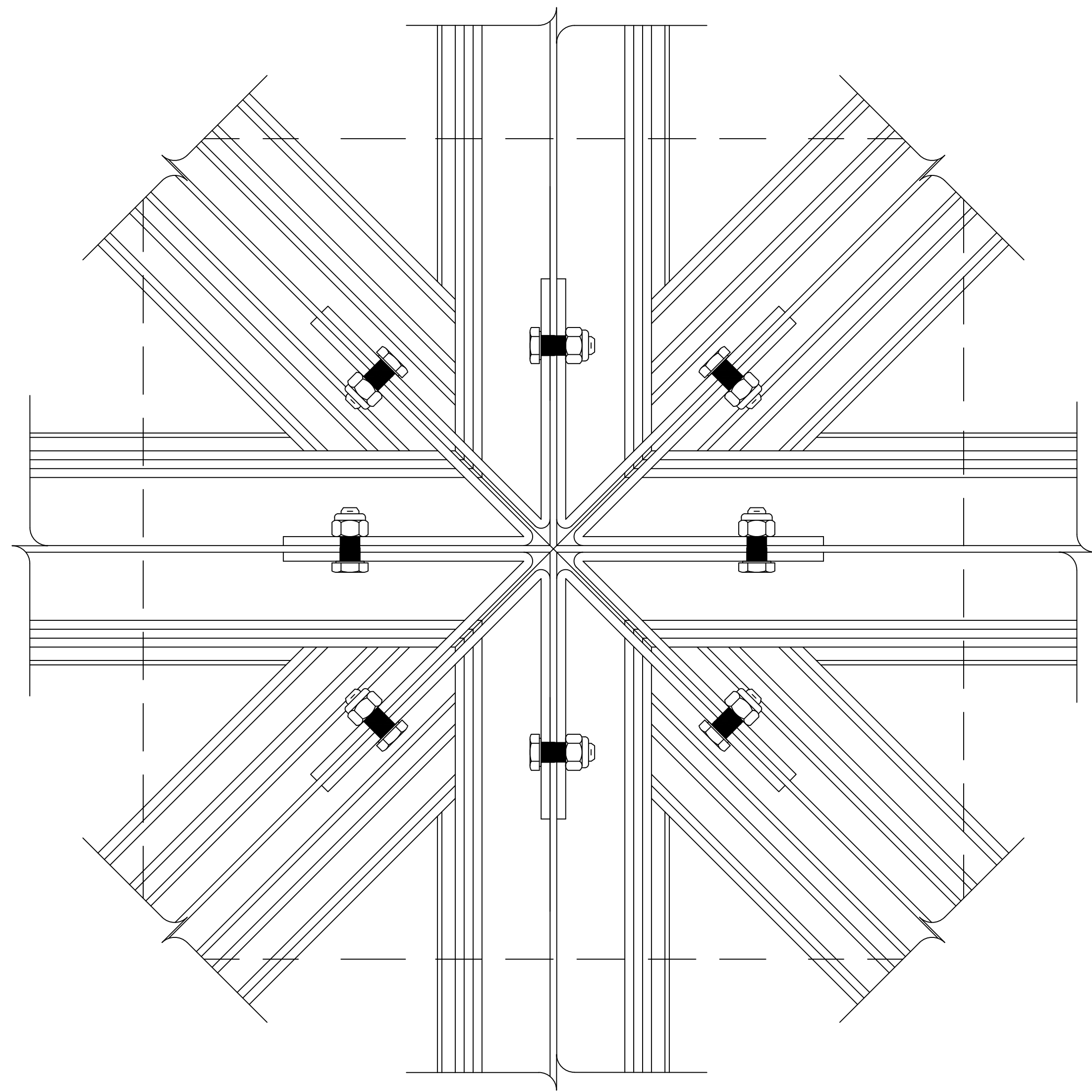
1 2 CONNECTION AT PEAK — — SCALE: 3/4" = 1"
