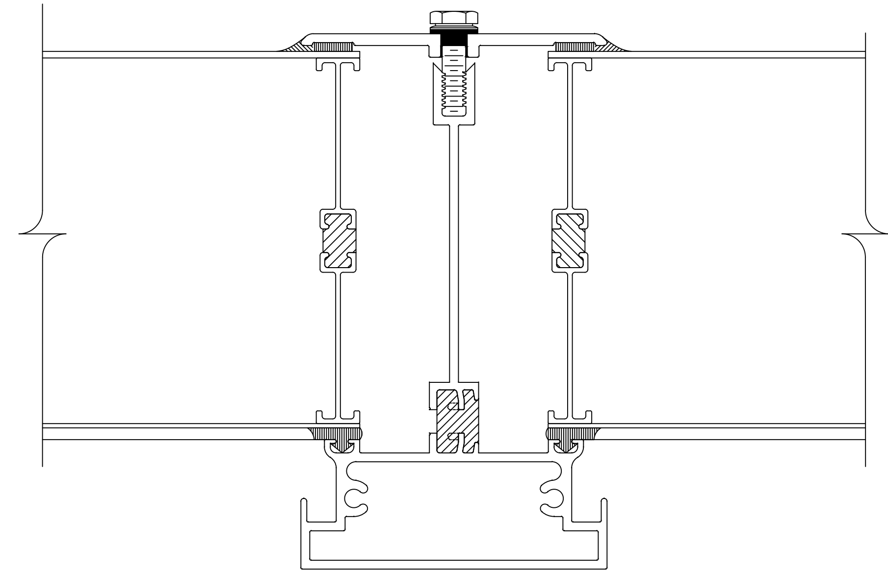
3 2 RAFTER DETAIL — — SCALE: FULL
