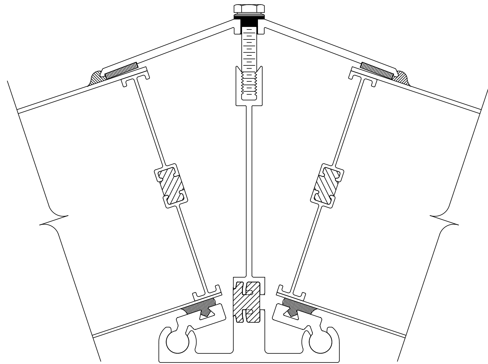
2 2 HIP DETAIL — — SCALE: FULL
