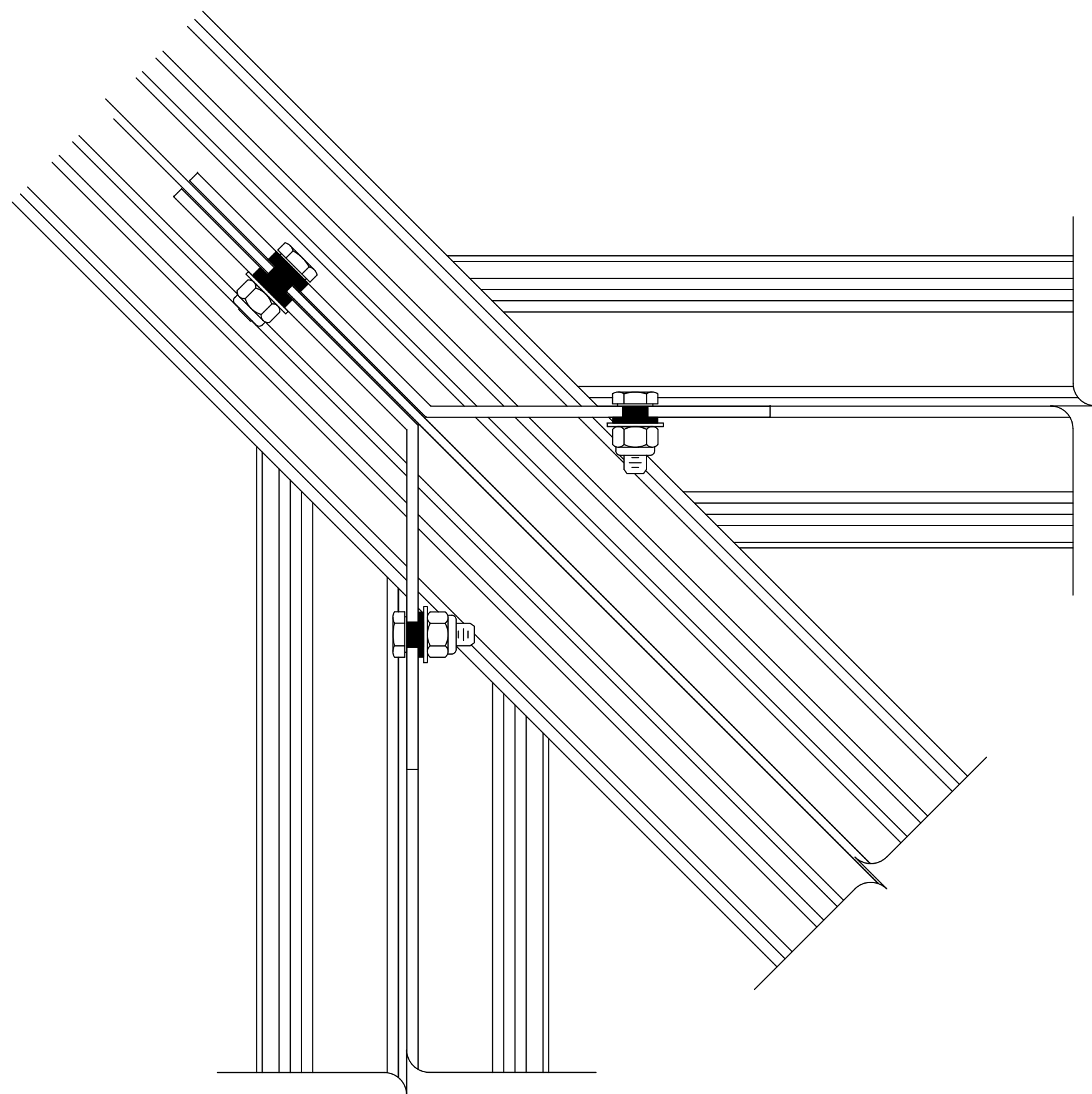
2 3 JACK RAFTER CONNECTION - - SCALE: 3/4" = 1"
