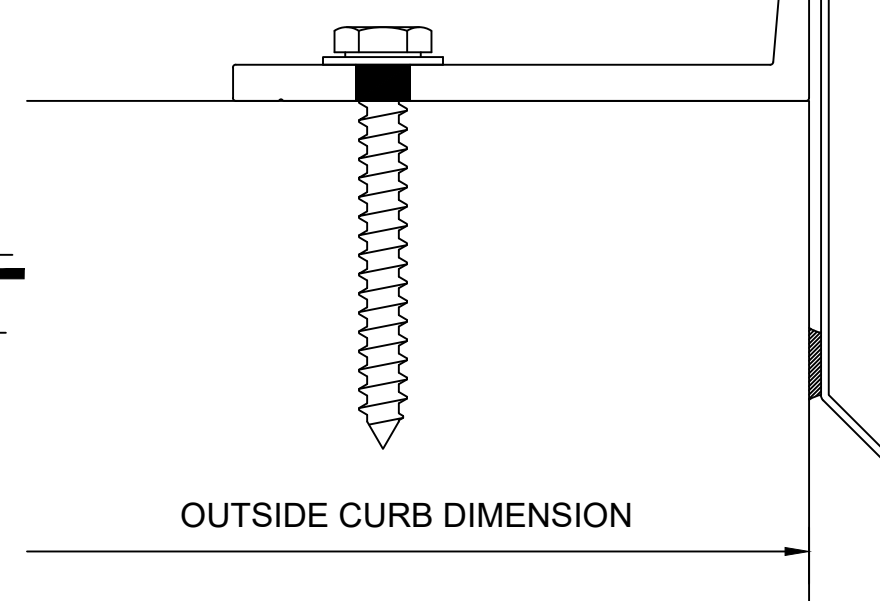
4 2 CURB DETAIL — — SCALE: FULL
