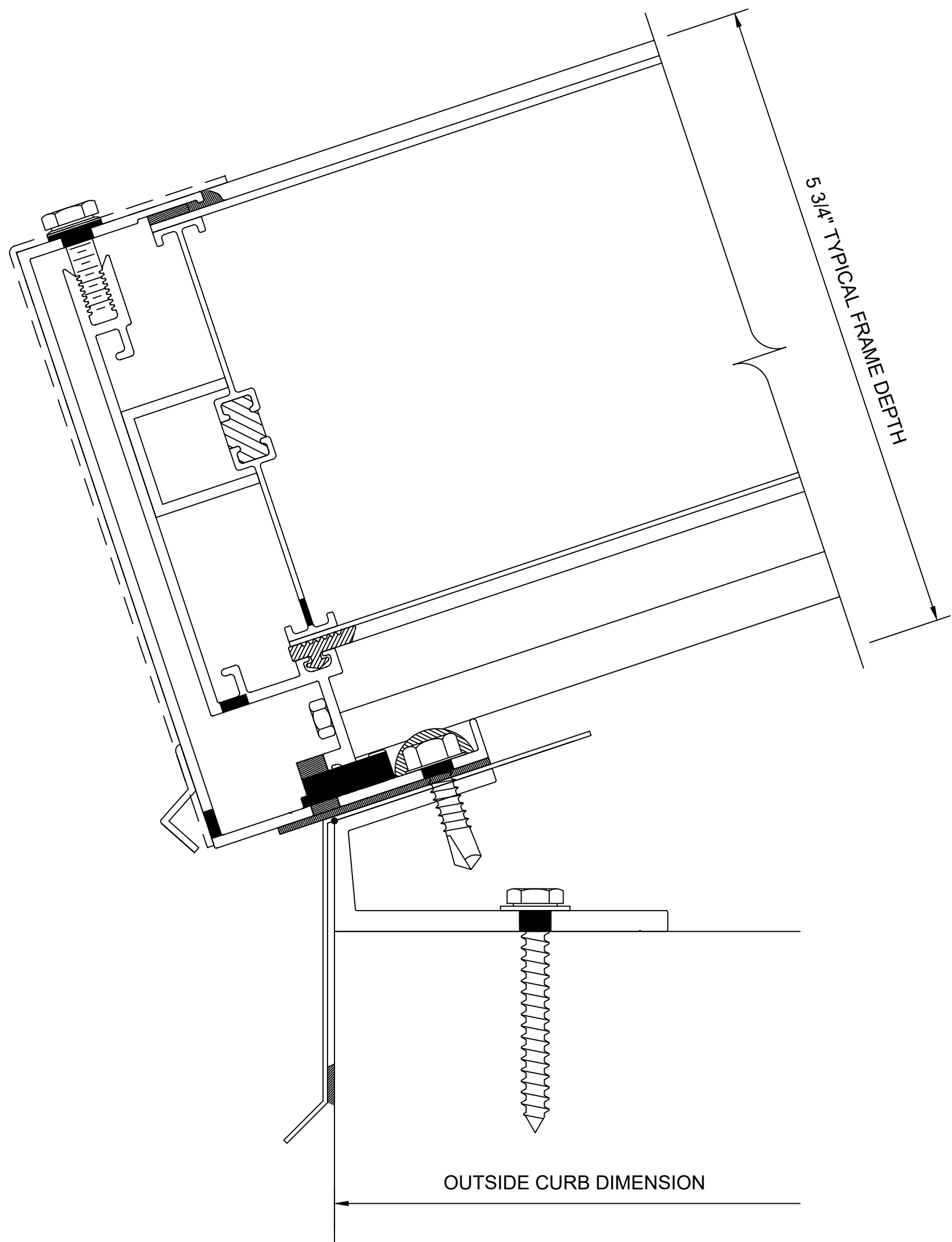
1 2 CURB DETAIL — — SCALE: FULL
