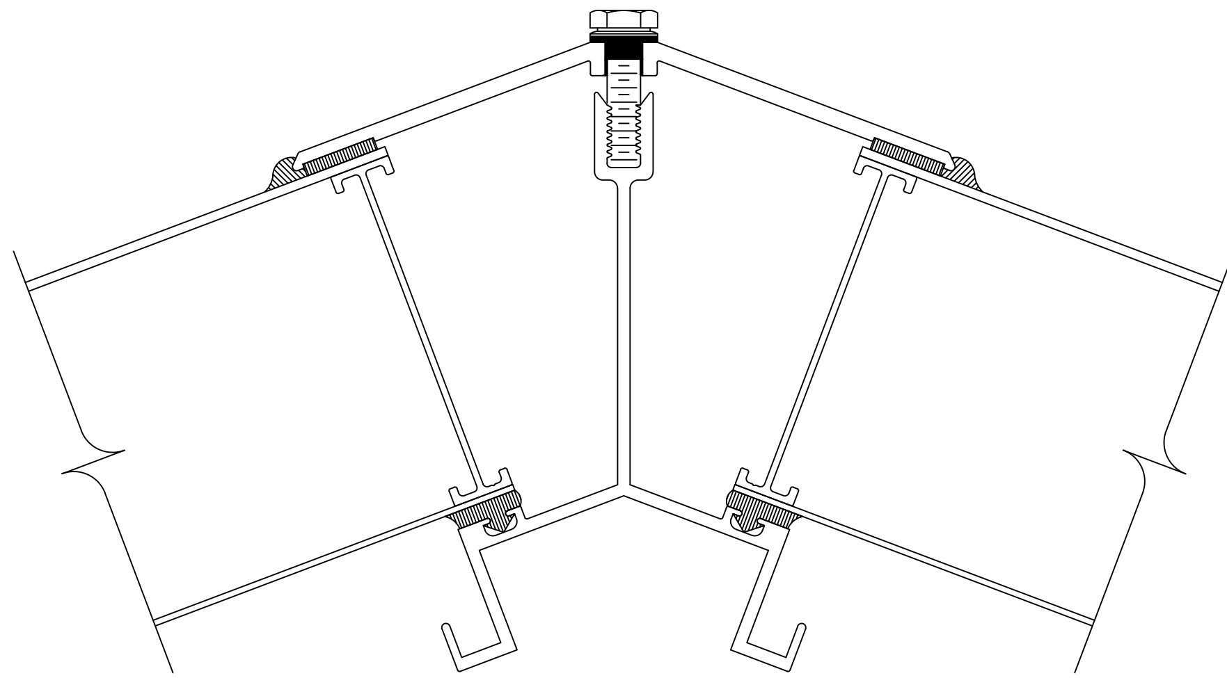
1 2 HIP DETAIL — — SCALE: FULL
