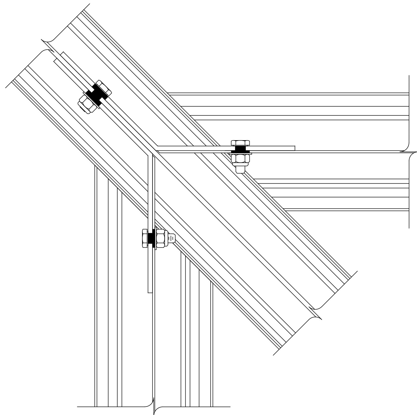
5 2 JACK RAFTER CONNECTION — — SCALE: 3/4" = 1"
