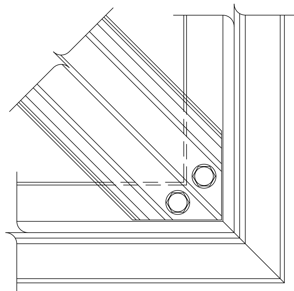
6 2 HIP CONNECTION DETAIL — — SCALE: 3/4" = 1"
