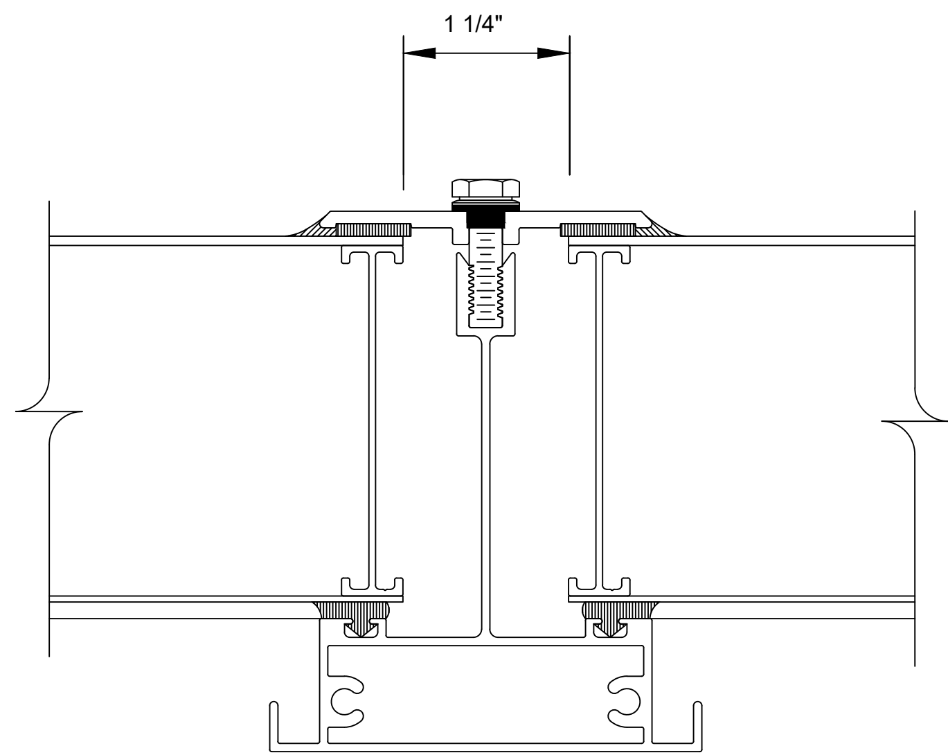
4 2 RAFTER DETAIL — — SCALE: FULL
