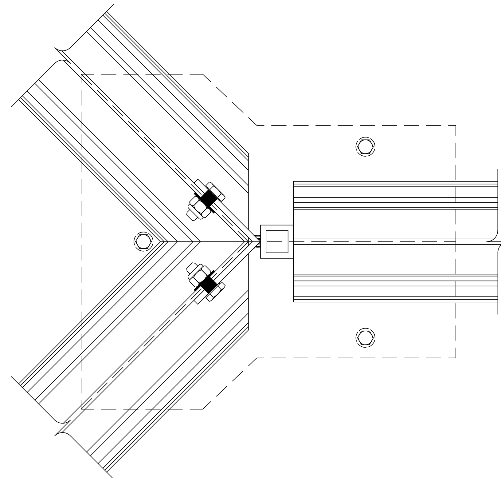
7 2 SECTION @ COMPRESSION RING — — SCALE: 3/4" = 1"
