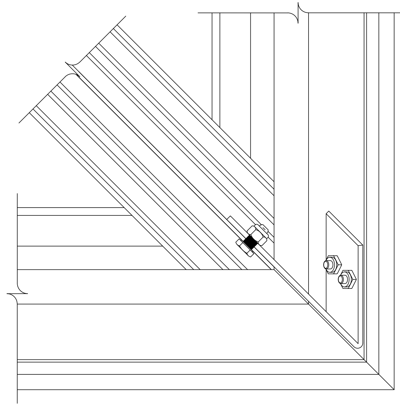
3 3 HIP CONNECTION DETAIL — — SCALE: 3/4" = 1"
