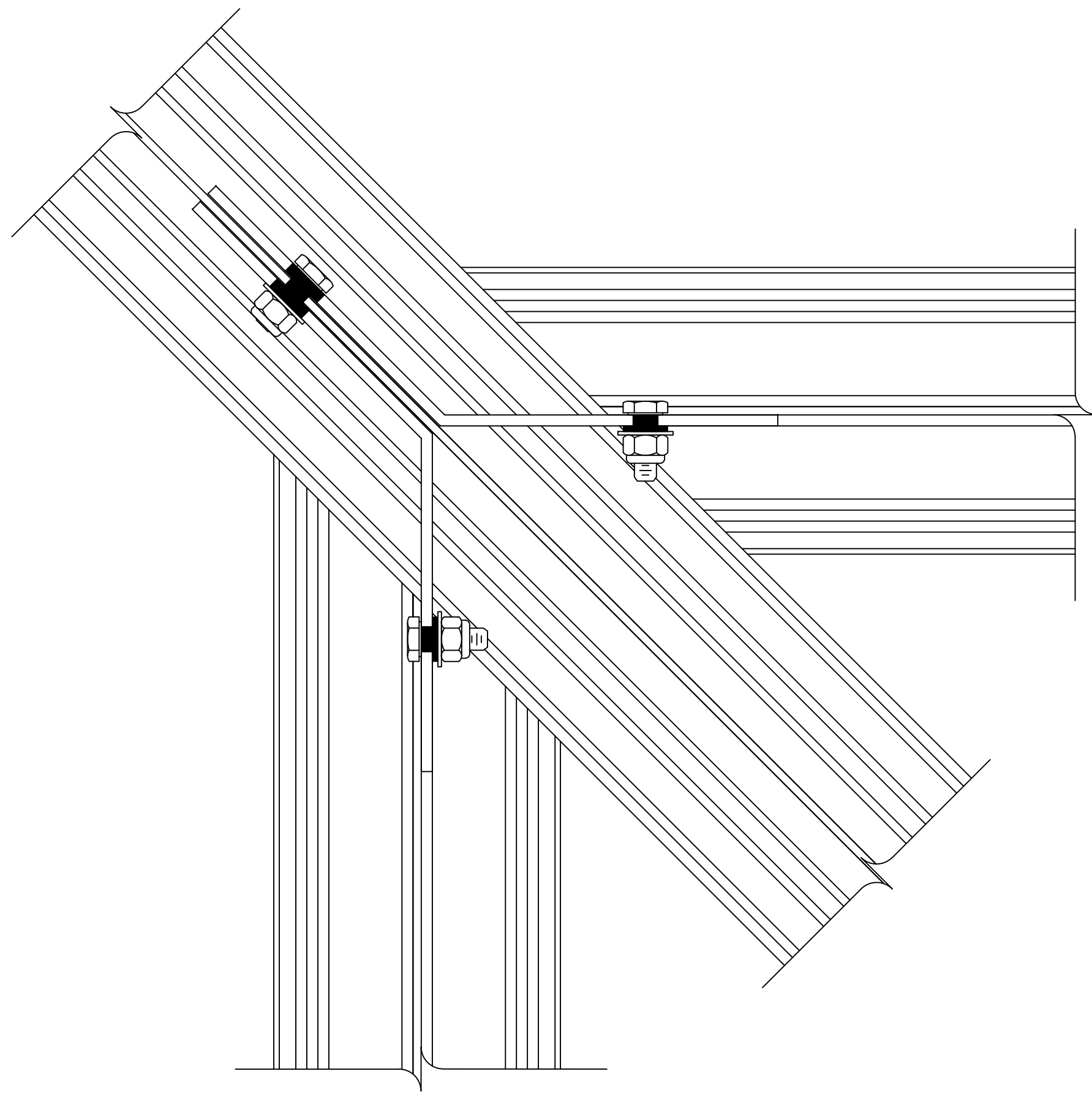
2 3 JACK RAFTER CONNECTION — — SCALE: 3/4" = 1"
