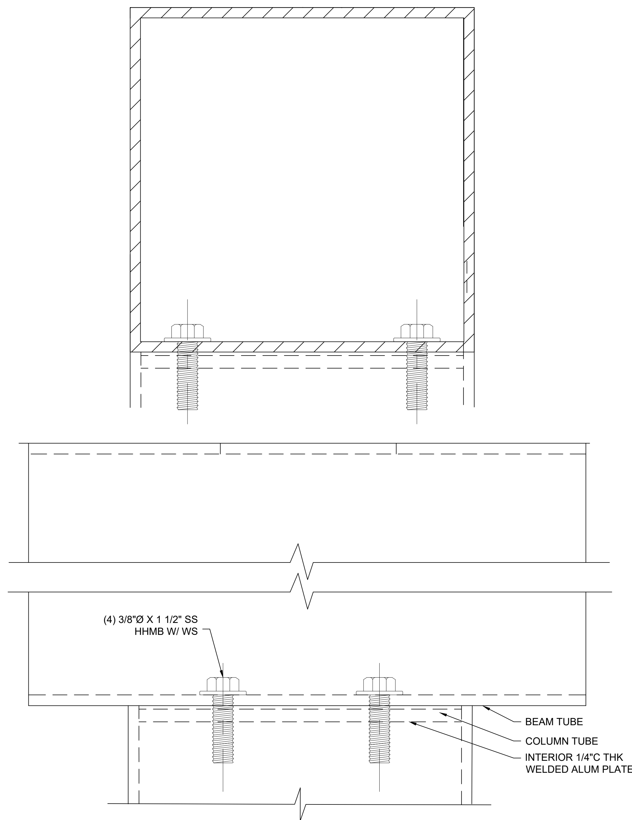
G COLUMN/BEAM CONNECTION 12 MM SINGLE GLAZED (16 MM SINGLE PANEL SIMILAR)
