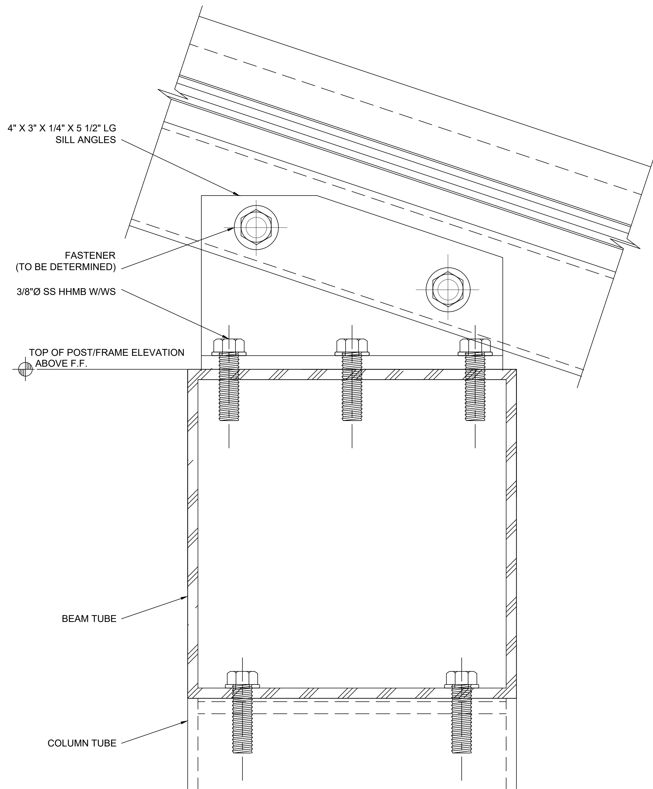
F RAFTER TO BEAM 12 MM SINGLE PANEL (16 MM SINGLE PANEL SIMILAR)
